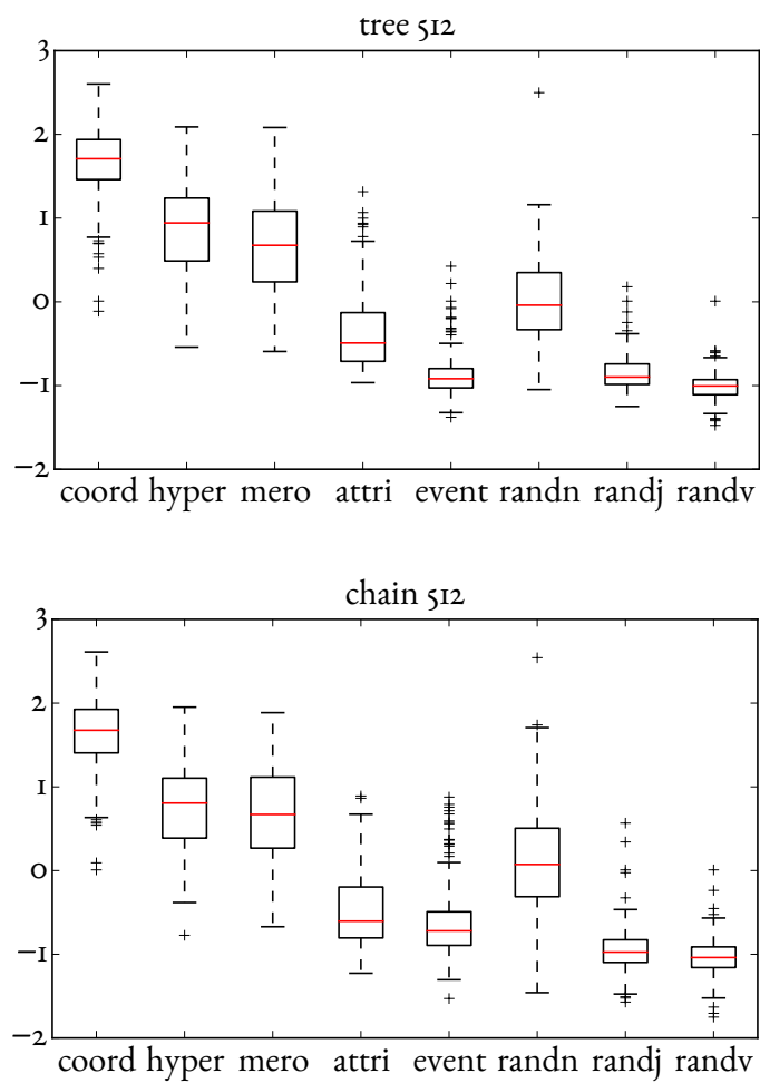
Figure 3.1: Distributions of similarity scores for different relations, for a tree model (top) and a chain model (bottom) on the BLESS dataset.
