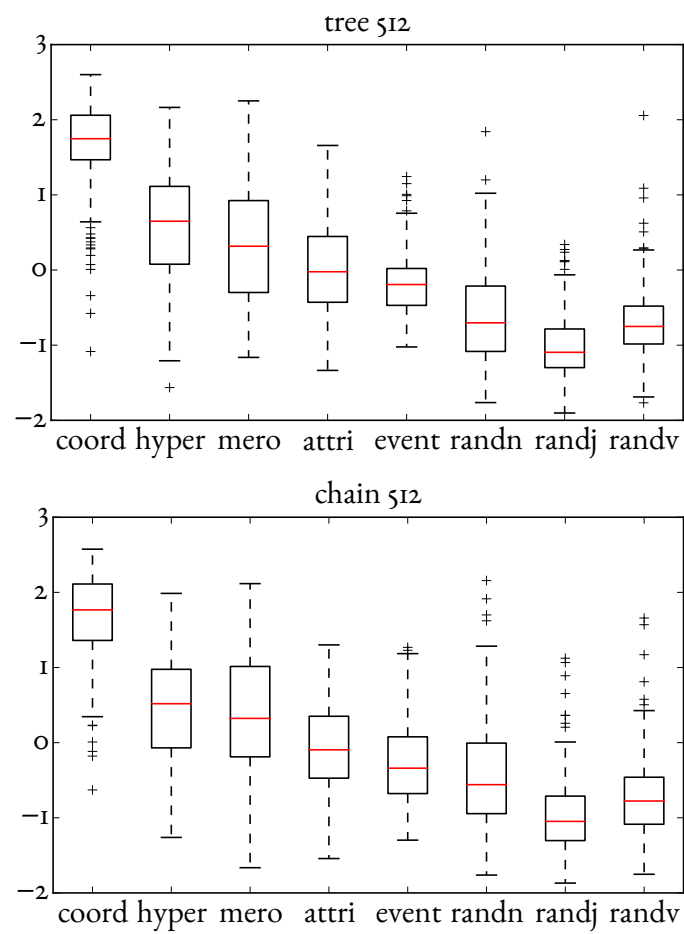
Figure 3.2: Distributions of similarity for different relations, for a tree model (top) and a chain model (bottom) on the BLESS dataset.
