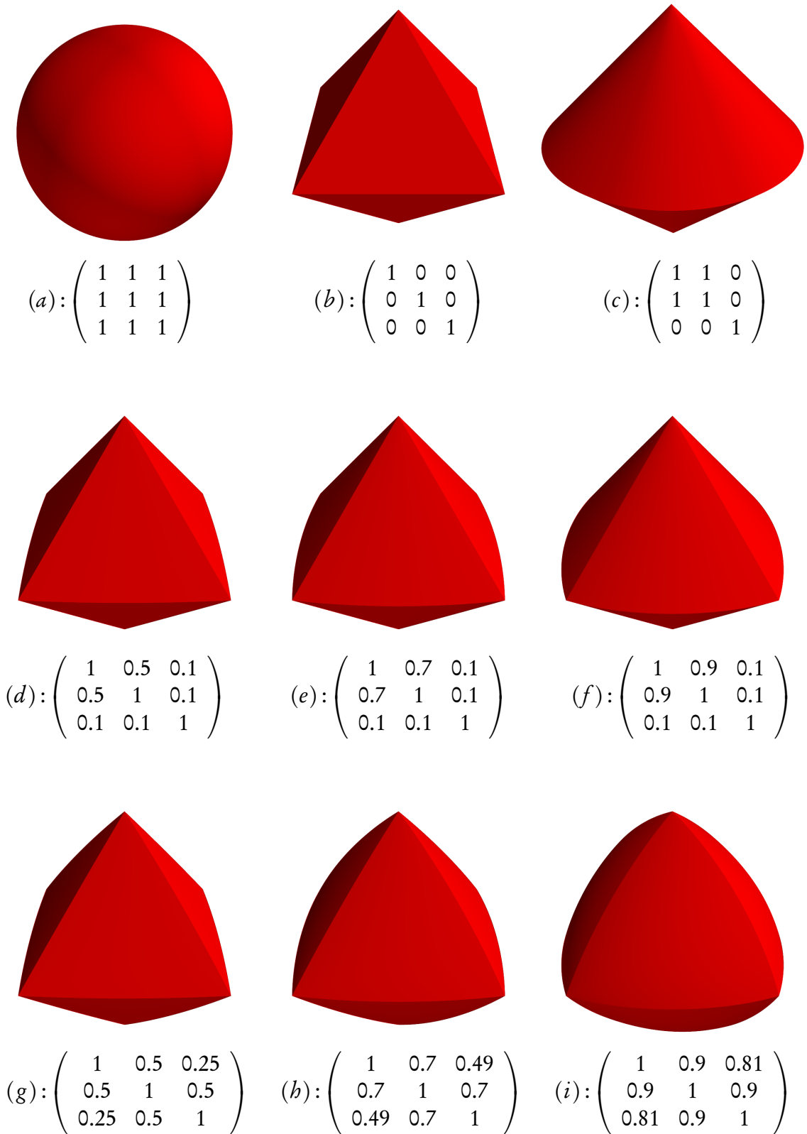
Figure 7.2: Unit balls for various value of \mathbf{P}^\top \mathbf{P} .
