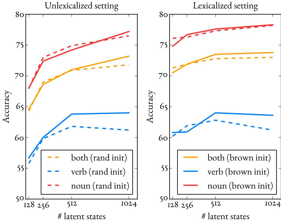
Figure 4.2: Classification accuracy for supsense tagging as a function of the number of latent classes for tree models. Accuracy for verbs is in blue, for nouns is in red and for both is in orange. Dashed lines are for random initialization, while plain lines are for Brown initialization.
