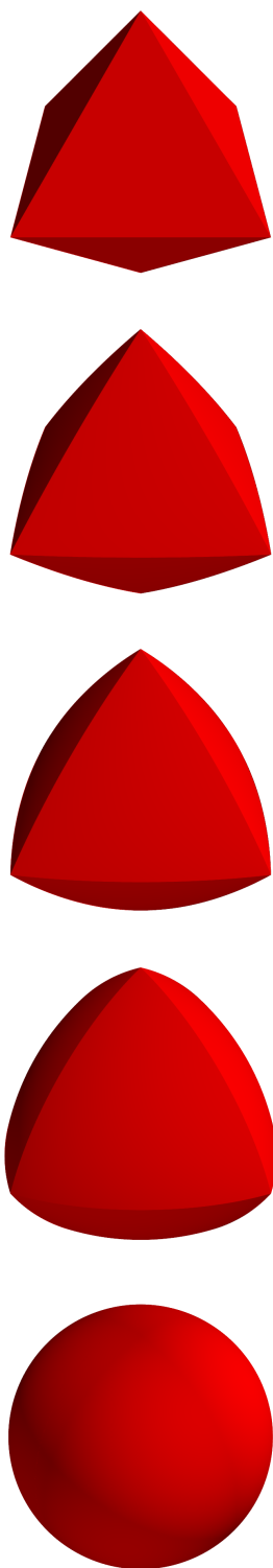
Figure 2: Unit balls of the trace Lasso norm for various value of \mathbf{X}^T \mathbf{X} . See the text for details.
