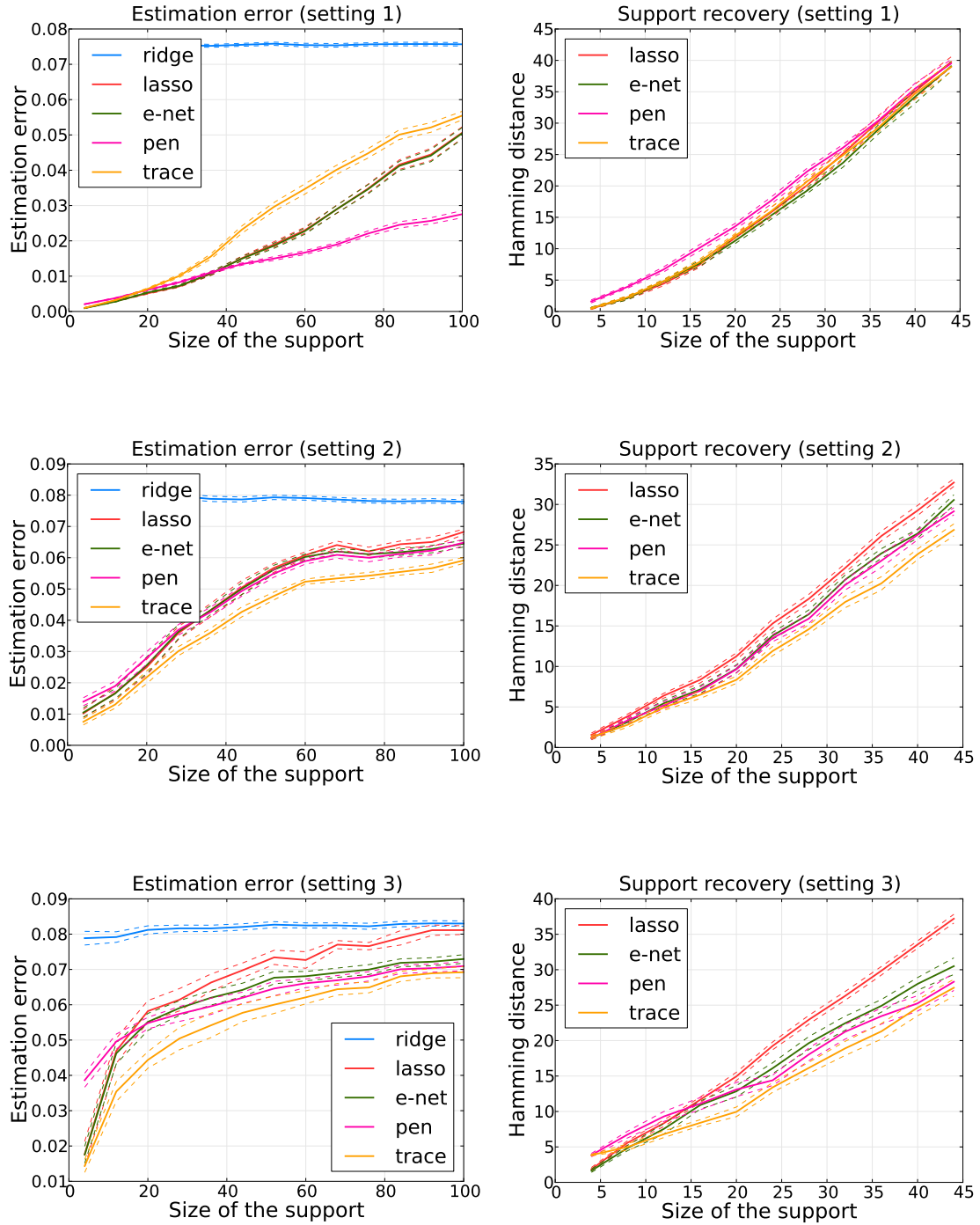
Figure 7.4: Left: estimation error ( p = 1024 , n = 256 ), right: support recovery ( p = 512 , n = 128 ). (Best seen in color. e-net stands for elastic net, pen stands for pairwise elastic net and trace stands for trace Lasso. Error bars are obtained over 20 runs.)
