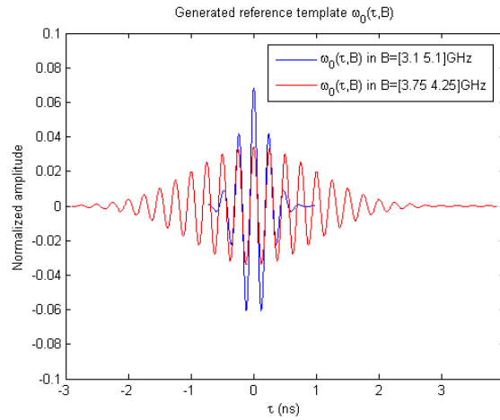
Figure 3.2: Energy-normalized templates w_0(\tau, B) used for the generation of synthetic received signals and for correlation-based TOA estimation.
