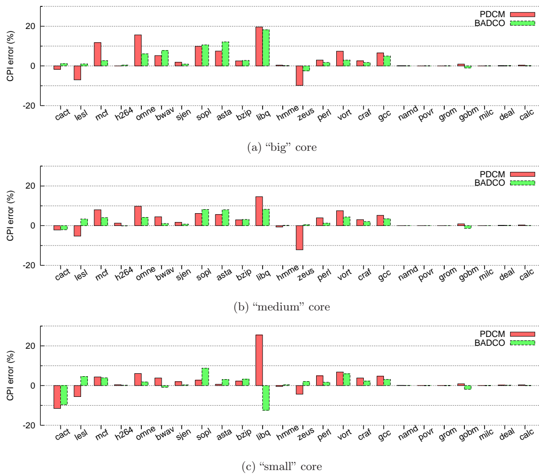
Figure 3.6: CPI error of PDCM and BADCO for the "small", "medium" and "big" cores, with the uncore configuration "001".
