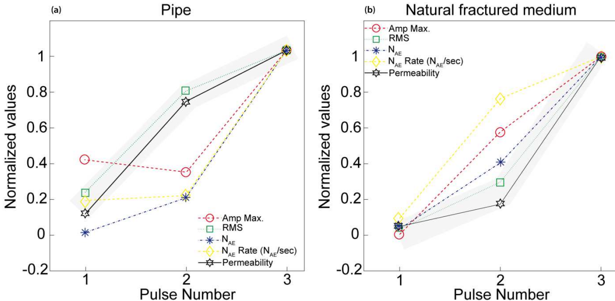
Figure 45: Normalized values of the different AE parameters: maximum amplitude of the signal ( Amp. Max. ), RMS value ( RMS ), number of acoustic events ( N_{AE} ), count rate ( N_{AE} Rate) and permeability in the case of (a) the pipe and (b) the fracture experiments.
