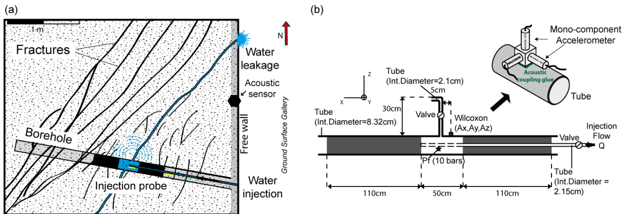
Figure 39: (a) Geological structure and experimental set-up in the field and (b) schematic cross-section of the experimental steel pipe used in the laboratory tests.
