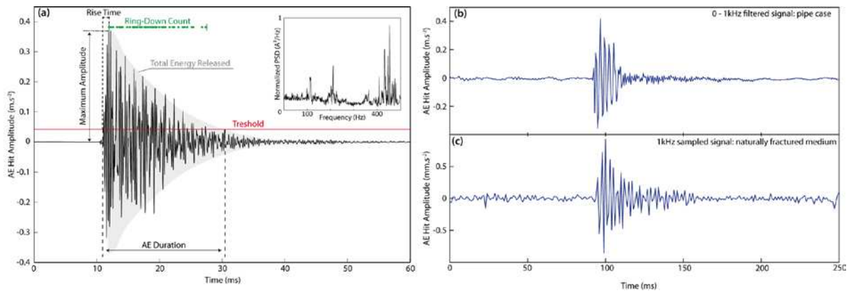
Figure 43: (a) Typical Acoustic Emission (AE) and its attributes recorded on the X-component of the sensor during the first pulse in the pipe experiment. The right up signal corresponds to its PSD computed with equation (2). (b) Same signal as in (a) but filtered with a band-pass Butterworth filter from 0 to 1kHz. (c) Typical AE recorded in the naturally fractured medium.
