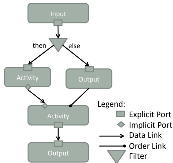
Figure 3.6: Graphical Convention - Abstract Elements
