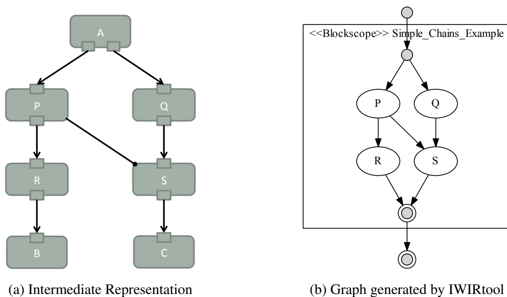
Figure 4.40: Conversion to IWIR - Simple Chains Example
