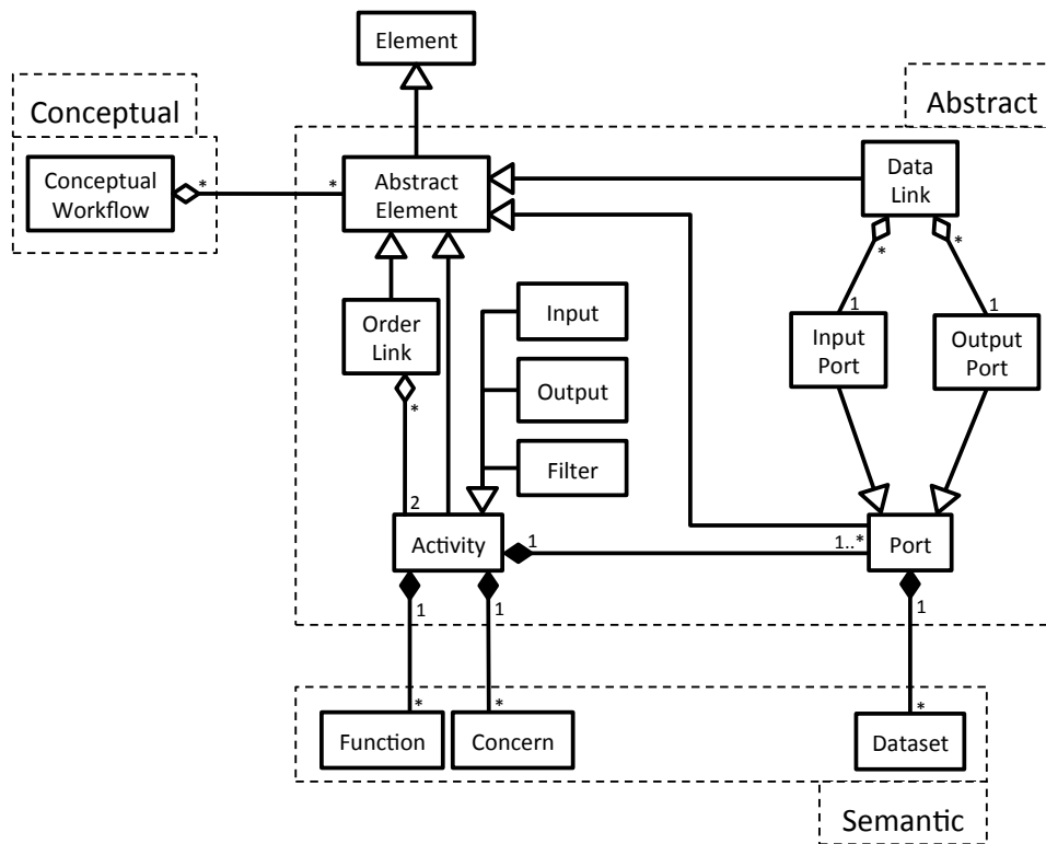
Figure B.2: Conceptual Workflow Meta-model - Abstract Part
