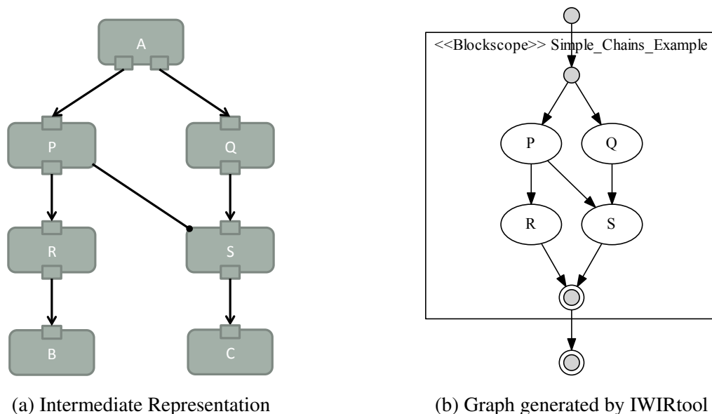
Figure 4.40: Conversion to IWIR - Simple Chains Example
