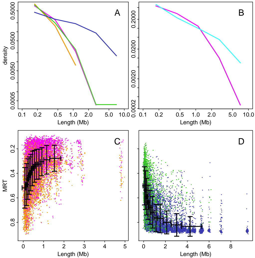
Figure V.11: Spatial organization of chromatin states in Nhdad . (A) Histogram of chromatin state block length in a logarithmic representation (Sect. V.5.13). (B) same as (A) for chromatin states C1 and C2 (C1+C2, light red) or by states C3 and C4 (C3+C4, light blue). (C) MRT in chromatin state blocks C1+C2 with respect to their length. Each 100 kb window in a chromatin state block is represented by the color of its state defined in Fig. V.3D',E'. The mean profile was obtained by (i) ordering data points according to their block length, (ii) grouping them in classes of equal number of data points and (iii) computing the average length and MRT over each class. Vertical bars represent the standard deviation. Horizontal bars represent the range of length over each class. (D) Same as (C) for chromatin state blocks C3+C4.
