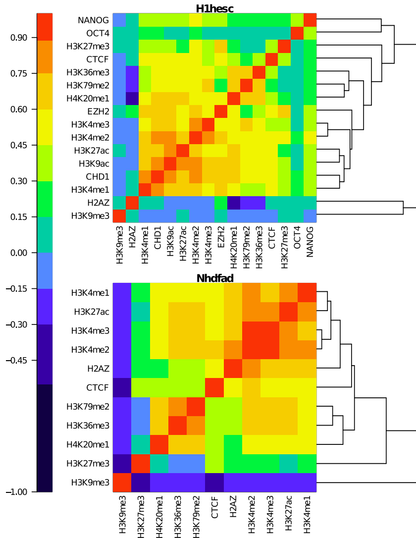
Figure V.1: Spearman correlation matrix between epigenetic marks in H1hesc (top) and Nhd1ad (bottom). For each cell line, we computed the Spearman correlation over all 100 kb non-overlapping windows with a valid score. Spearman correlation value is color coded using the color map shown on the left. Lines for the epigenetic marks were reorganized by a hierarchical ordering using Spearman correlation distances (Eq. (V.1)) as illustrated by the dendrograms on the right of the corresponding matrices. This ordering implies that highly correlated epigenetic marks are close to each other.
