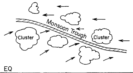
Figure 1.7 - Schematic picture of the typical organization of cloud clusters in the south-westerly monsoon or trade wind flow. Figure from Gray [1998].
