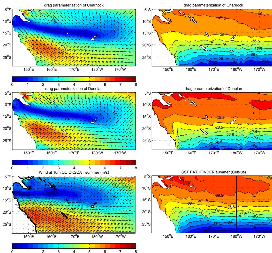
Figure 2.13 - Summer 10-m wind speed and SST ( ^{\circ}\text{C} ) for two WRF-ROMS coupled simulations differing by their surface drag parameterization: (a) the Charnock parameterization and (b) the Donelan parameterization.
