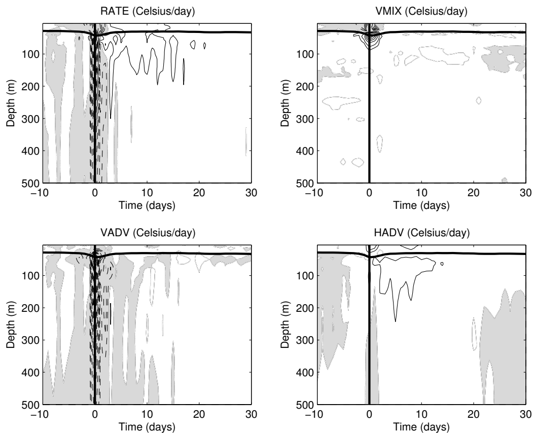
Figure 4.11 - Model composited anomalies of temperature tendencies ( ^{\circ}\text{C}\cdot\text{day}^{-1} ) in the cyclone wake over the first 500 m in the storm-track center (averaged over 0.25^{\circ} radius) as a function of time relative to occurrence. Shown are (a) rate of change, (b) vertical mixing, (c) vertical advection, and (d) horizontal advection. Dashed contours and gray areas are for negative values; solid contours and white areas are for positive values. The contour interval is 0.05^{\circ}\text{C}\cdot\text{day}^{-1} with additional 0.025 positive and negative contours. The bold solid line is the mixed layer.
