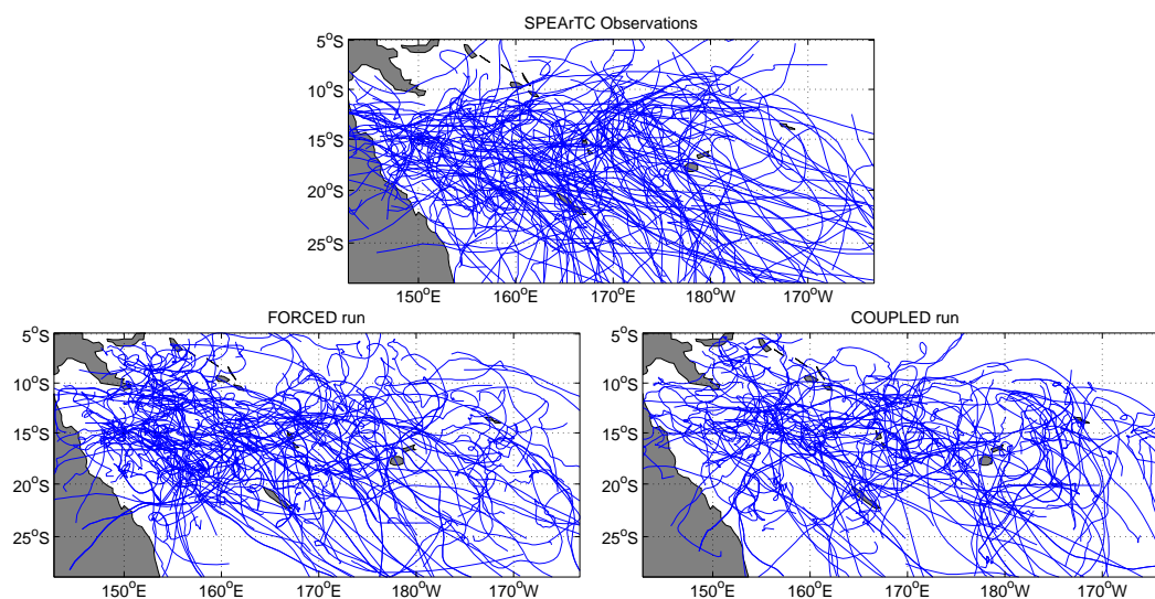
Figure 2.19 - 1979-1998 TC tracks for the observations, the forced run and the coupled run with chosen tracking criteria ( \text{VOR} = 20 \cdot 10^{-5} \text{ s}^{-1} , \text{WT} = 17 \text{ m} \cdot \text{s}^{-1} and \text{TT} = 1 \text{ K} ).
