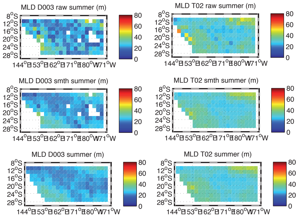
Figure 3.1 - Climatological summer MLD from Montegut et al. [2004] dataset computed with (left) density criterion ( \rho - \rho_{10m} > 0.03kg.m^{-3} ), (right) temperature criterion ( T - T_{10m} < -0.2^{\circ}C ). (a-b) are the raw estimates (median value in each grid box), (c-d) are the estimates with smoothing by weighted neighboring profiles and (e-f) are the final estimate after smoothing and kriging.
