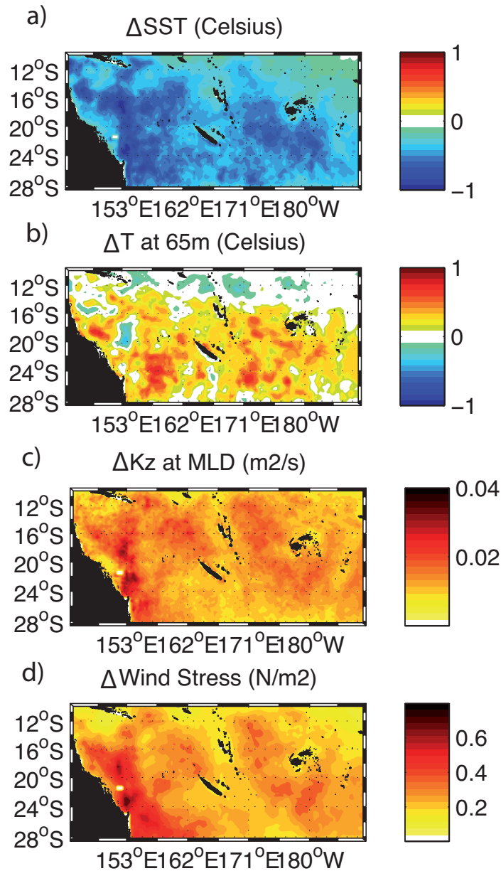
Figure 4.8 - Composite anomalies of all cyclone tracks (using a 6° radius) representing the model composited effect of cyclones within a day of their occurrence for (a) the SST (°C); (b) the temperature at 65 m (°C); (c) the vertical mixing coefficient ( m^2 \cdot s^{-1} ); and (d) the wind stress ( N \cdot m^{-2} ).
