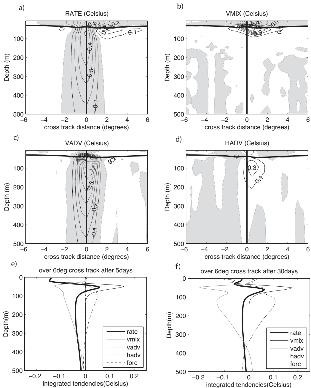
Figure 4.12 - Model composited anomalies of temperature tendencies ( ^{\circ}\text{C} ) integrated between days -2 and +5 on a cross-track section: (a) rate of change; (b) vertical mixing; (c) vertical advection; and (d) horizontal advection. Dotted contours and gray areas are for negative values; solid contours and white areas are for positive values. The contour interval is 0.1^{\circ}\text{C} . The bold solid curve is the mixed layer depth and the vertical solid line is the track center. (e) Section-averaged composite anomalies integrated between days -2 and +5. (f) As in (e), but integrated between days -2 and 30. The black bold curve is the rate of change, the black thin curve is vertical mixing, the gray curve is vertical advection, the dotted curve is horizontal advection, and the dashed curve is surface forcing.
