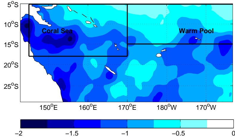
Figure 5.13 - Composite map of storm-induced SST cooling ( ^{\circ}\text{C} ). In the construction of this map, if two TC tracks overlap, the coolings are averaged.
