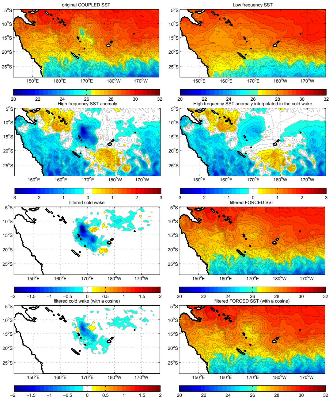
Figure 2.21 - SST fields ( ^{\circ}\text{C} ) in the different steps of cold wake filtering procedure: (a) original coupled model SST during a particular TC event; (b) low-frequency SST filtered with a 90-day FFT low-pass filter; (c) high-frequency SST anomaly computed as the difference between SST and low-frequency SST; (d) high-frequency SST anomaly in which the cold wake was removed and the surrounding HF SST anomaly interpolated; (e) the filtered cold wake, (f) the final SST field used as forcing for the forced atmospheric model. (g) and (h) are similar to (f) and (g) but using a 90-day cosine filter.
