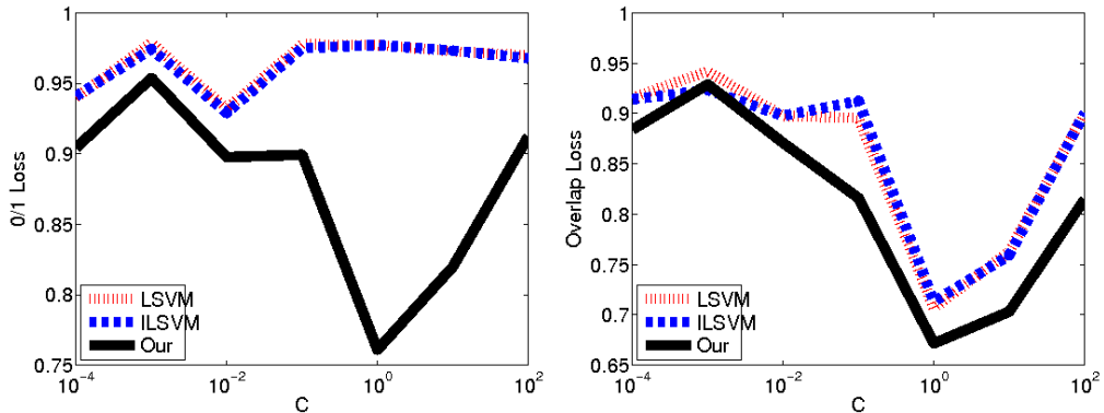
FIGURE 4.2: The average test loss over five folds (y-axis) of the action detection application for different values of C (x-axis, shown in log-scale). Left: 0/1 loss; Right: Overlap loss. Our framework outperforms both latent SVM and ILSVM and provides statistically significant improvements for both types of loss (see text for details).
