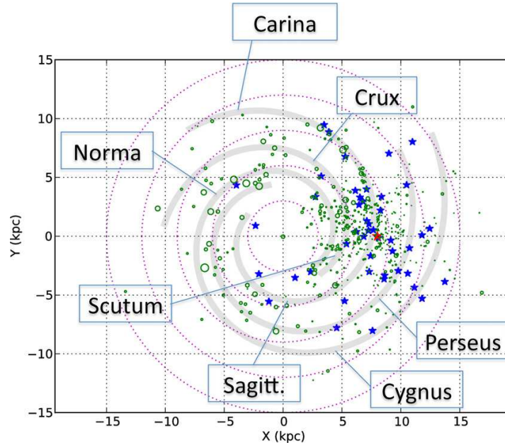
Figure 4. Distribution of HMXBs (blue stars) and SFCs (green circles). The circle radius of SFCs represents the excitation parameter value. The spiral arm model from Russeil (2003) is also plotted, and the red star at (8.5; 0) represents the Sun position. (A color version of this figure is available in the online journal.)
