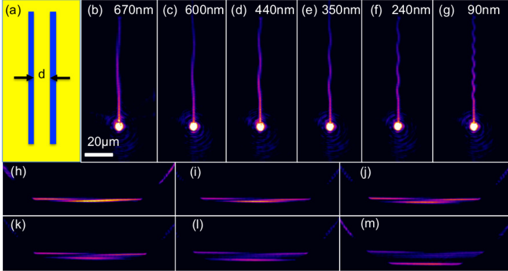
Figure 2.8: (a) Schematic of a linear DLSPPW coupler. (b) to (g) are direct-space images of the intensity distribution in linear DLSPPW couplers with edge-to-edge distance d equals to 670 nm, 600 nm, 440 nm, 350 nm, 240 nm and 90 nm respectively. (h) to (m) are the corresponding wave-vector distributions unambiguously demonstrating the degeneracy lift of the coupled waveguides for small values of d .
