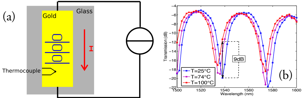
Figure 3.6: (a) Schematic view of the experimental set-up used for the thermo-optics DC characterization of the resonators. (b) Change of the transmission spectra of the resonator with R = 5.8\mu\text{m} , L = 2.5\mu\text{m} and G = 240 \pm 40\text{nm} as a function of the temperature.
