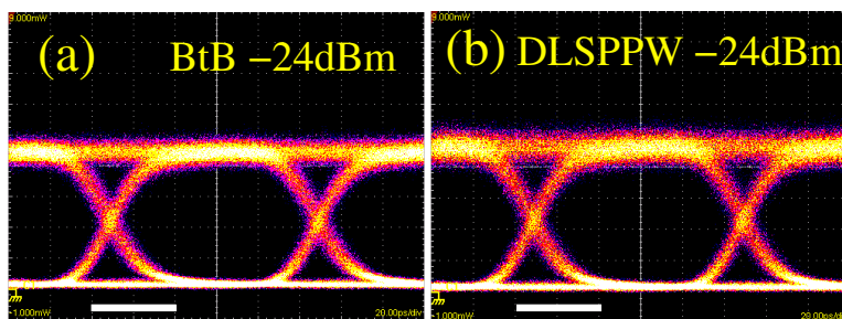
Figure 4.13: Eye-diagrams of the Back-to-Back (a) and transmitted 10 Gbits/S signal (b) for a received average power of -24\text{dBm} at \lambda_o = 1545\text{nm} . Scale bar= 40 ps.
