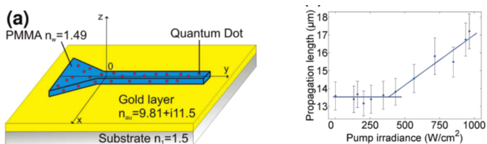
Figure 1.16: (a) Schematic view of Q-dots doped DLSPPW, (b) Propagation length in function of the pump power (Adapted from [76]).
