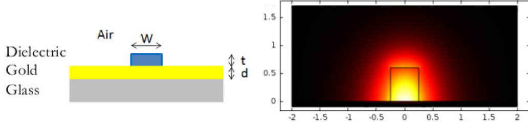
Figure 2.1: (a) Schematic view of a basic PMMA DLSPW cross section of a width w=600 nm and thickness t=500 nm onto a 60 nm thick gold film. (b) Corresponding Electric field map of the DLSPW mode at \lambda=1550 nm ( n_{\text{PMMA}} = 1.489 , n_{\text{Au}} = 0.55 + i11.5 , n_{\text{substrate}} = 1.5 ).
