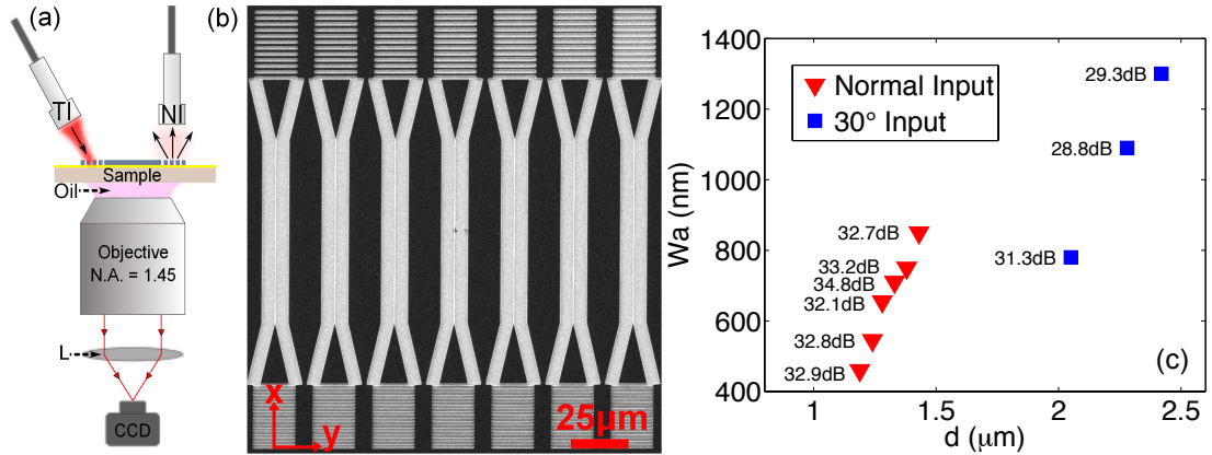
Figure 4.10: (a) Schematic representation of the characterization setup. The DLSPPW-mode is excited by focusing fiber-guided laser light onto the input grating whilst the scattered light at the output grating is collected by an identical focuser at normal incidence (NI) or tilted incidence (TI). The DLSPPW leakage radiation is collected by an oil-immersion objective (NA = 1.45) and focused onto an infrared CCD camera by a lens L. (b) SEM-image of a typical EBL writing-field comprising seven DLSPPWs.
