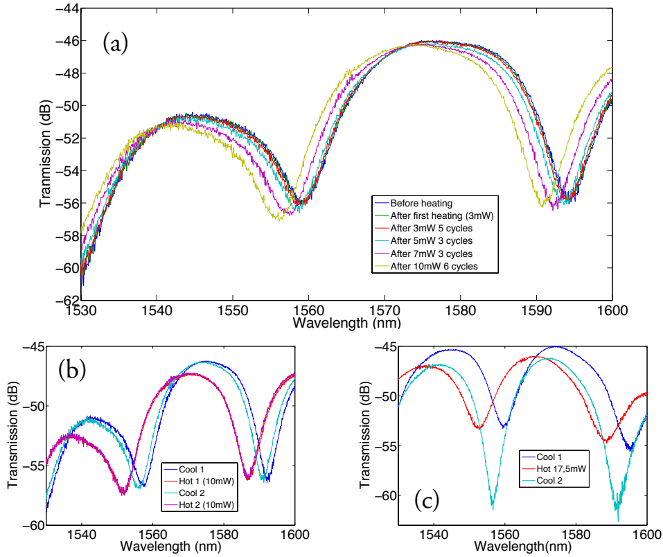
Figure 4.21: (a) Transmission spectra at the cool states after various heating cycles. (b) Thermo-optical effect shifting at moderated power. (c) Example of overheating illustrated by before/after transmission spectra.
