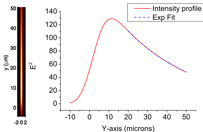
Figure 2.4: Intensity map (a) and profile (b) of a DLSPW obtained by Differential method
