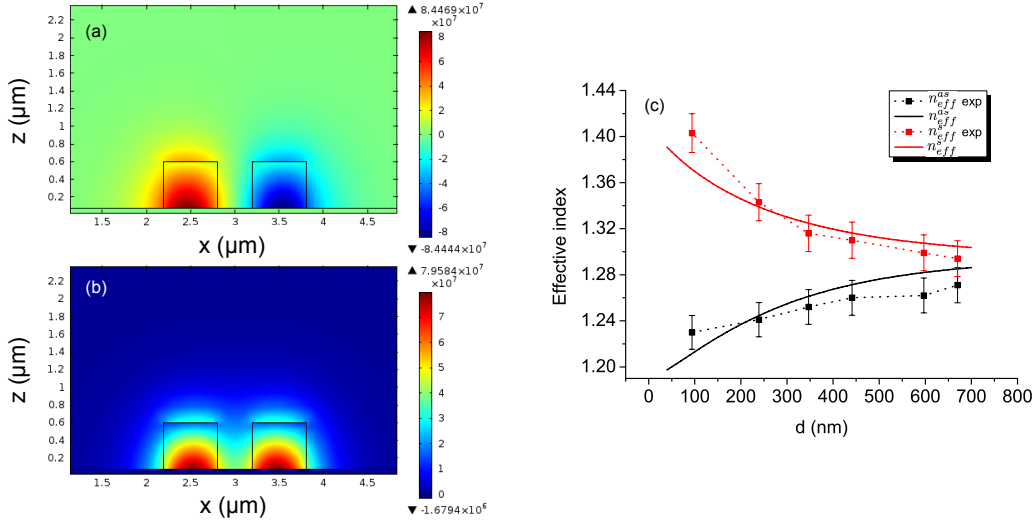
Figure 2.10: (a) and (b) are the electric field profiles of the asymmetric and symmetric modes propagating in two coupled DLSPWs separated by a d=400 nm. (c) Comparison between the experimental splitting of the modes and the calculated values for various coupling distance d .
