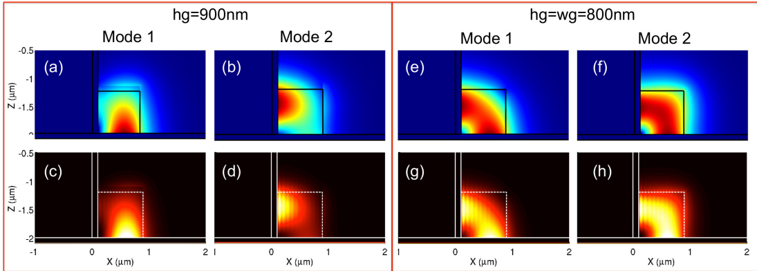
Figure 5.5: (a,b) Electric field distribution resulting from COMSOL Mode Analysis with h_g = 900 nm, (c,d) Electric field distribution resulting from the Differential method calculation with h_g = 900 nm, (e,f) Electric field distribution resulting from COMSOL Mode Analysis with h_g = w_g = 800 nm, (g,h) Electric field distribution resulting from the Differential method calculation with h_g = w_g = 800 nm
