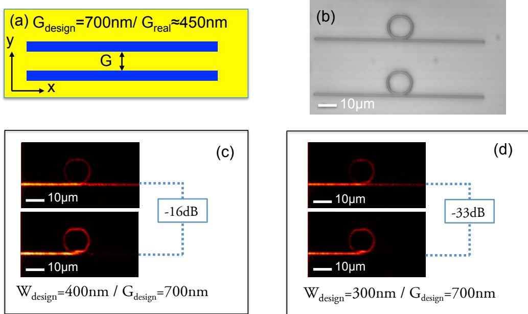
Figure 3.9: (a) Schematic view of a gap between two DLSPW, (b) Optical images of RTR made of Cyclomer, (c-d) LRM images of resonant/non-resonant RTR for different lithography parameters.
