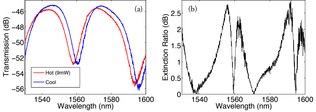
Figure 4.17: (a) Typical thermo-optical spectrum measured by Fiber-to-Fiber. (b) Corresponding Extinction Ratio spectrum (Eq. 3.10).
