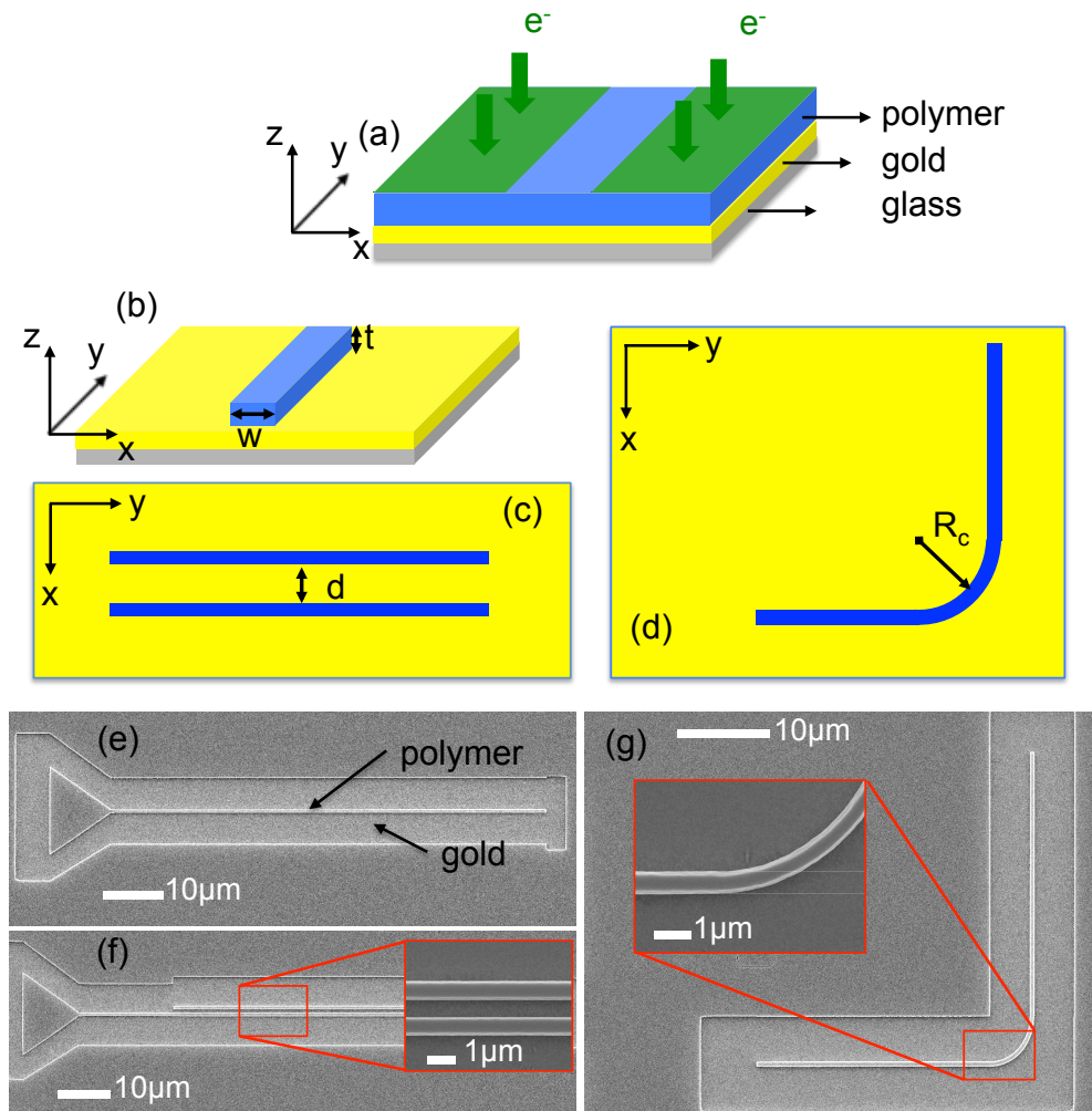
Figure 2.5: (a) Electron Beam exposure (b) Schematic view of a basic DLSPPPW with a width w of 600 nm and thickness t=560 nm. (c) Schematic view of two coupled waveguides separated by a gap d . (d) Schematic view of a waveguide with a curved section with a bend radius R_c . (e), (f) and (g) are scanning electron micrographs of typical devices corresponding to the configurations (b), (c), and (d), respectively.
