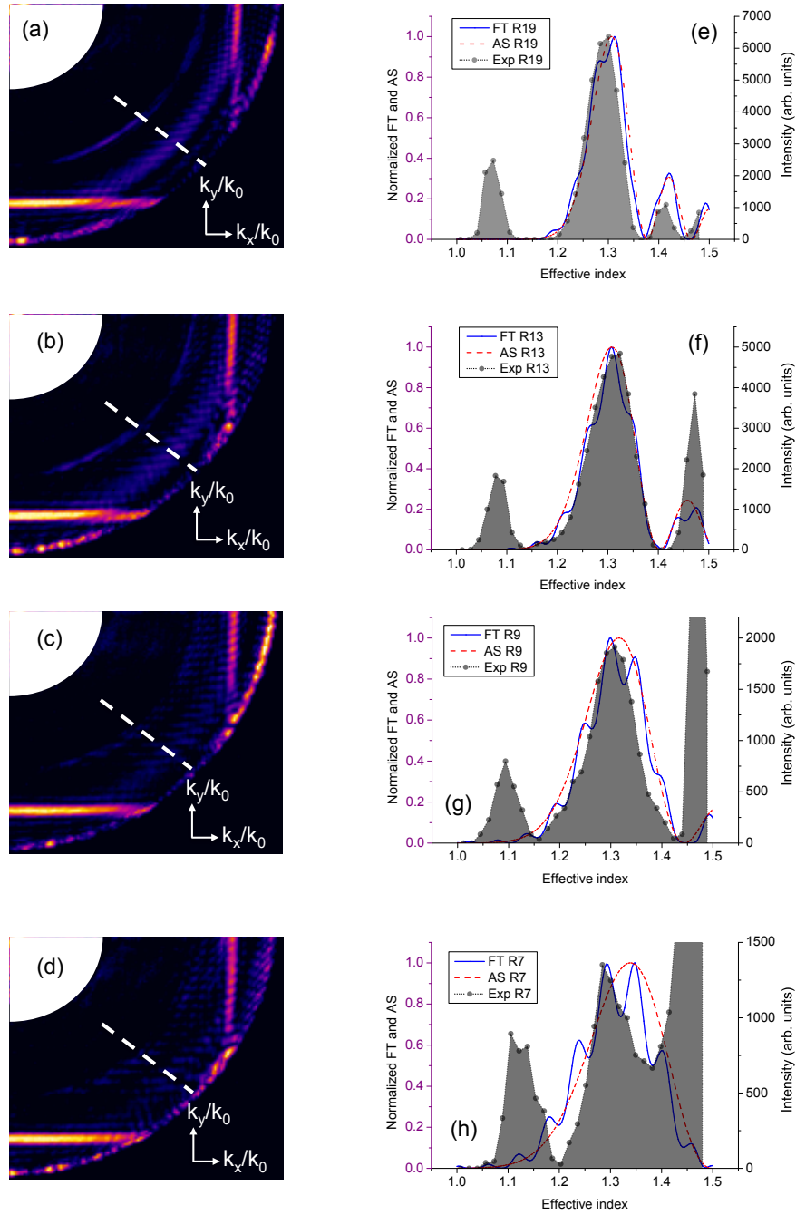
Figure 2.14: (a-d) Selected region of interest of the experimental momentum-space images for curved waveguides with R_c = 19 \mu\text{m} , 13 \mu\text{m} , 9 \mu\text{m} , and 7 \mu\text{m} , respectively. (e) to (h) Experimental profiles (shaded areas) of the wave-vector distribution taken along the dashed line in (a) to (d). The solid blue lines are the calculated profiles using Eq. 2.8 already reported in Fig. 2.12. The red dashed lines show the analytical solutions obtained with the n^{\text{th}} order rendering the best agreement with the data. n = 100, 68, 43, and 37 , respectively.
