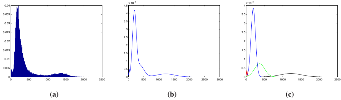
Figure A.1: Gaussian Mixture Model of the resection cavity intensity. (a) Intensity histogram, (b) Modeled intensity distribution, (c) Gaussians constituting the GMM.
