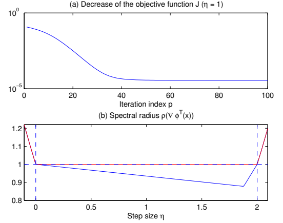
Fig. 3. Unsupervised NMF
