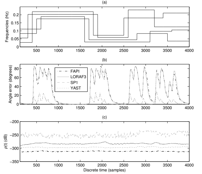
Fig. 1. Simulation results
