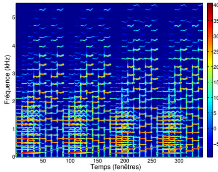
(a) Spectrogramme original
