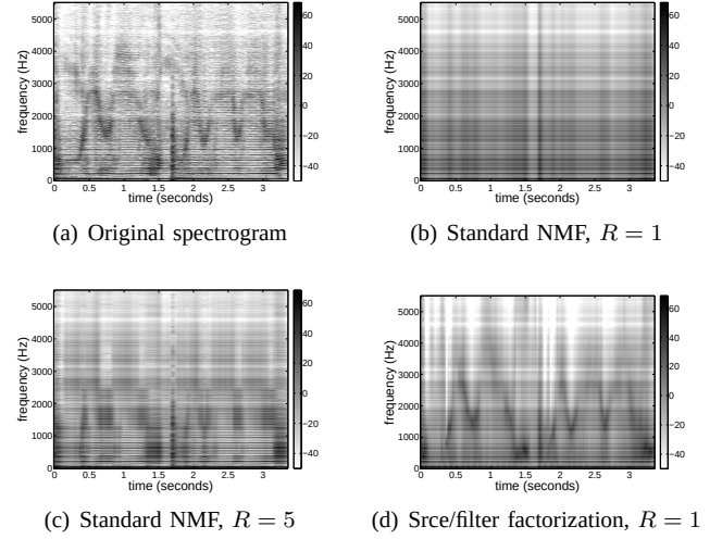
Fig. 1. Original power spectrogram of the extract of didgeridoo 1(a) and reconstructed spectrograms 1(b), 1(c) and 1(d)
