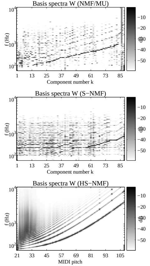
Fig. 3. Example basis matrices \mathbf{W} for algorithms without and with harmonicity constraint. Columns are sorted by increasing pitch.
