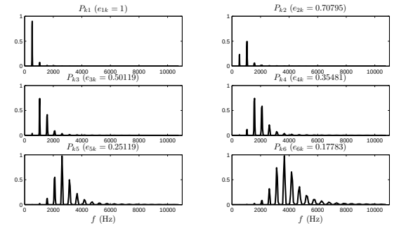
(b) Corresponding patterns \mathbf{P}_{km}
