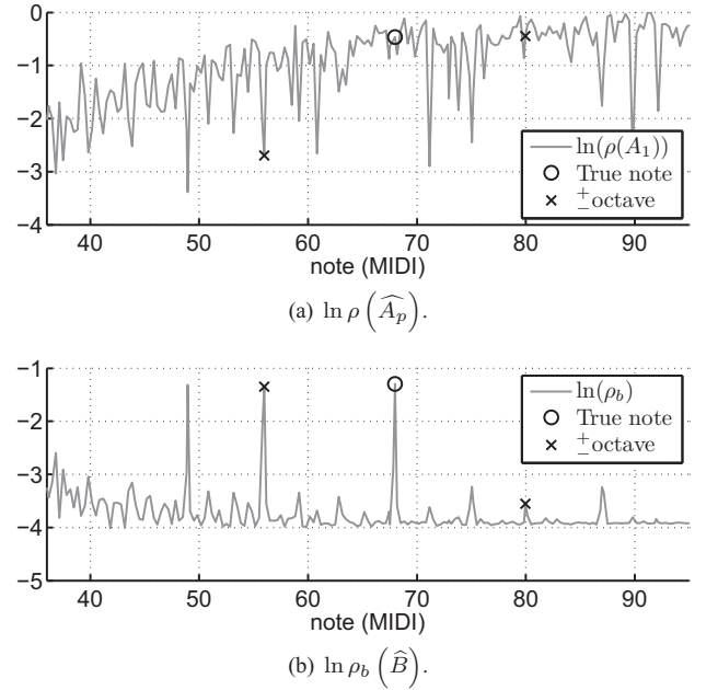
Fig. 6. \ln \rho(\widehat{A}_1) (top) and \ln \rho_b(\widehat{B}) (bottom) as a function of a single-note model (true note: A\flat_4 ).
