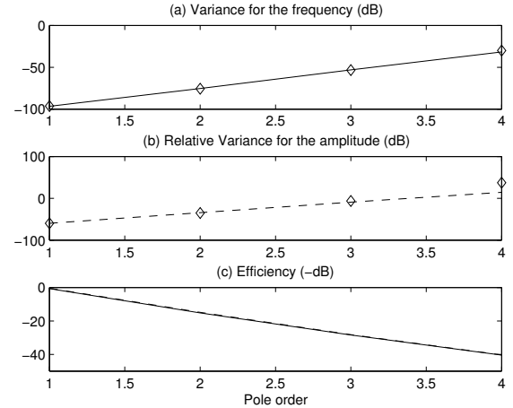
Fig. 5. Variation of the variances with respect to the pole order
