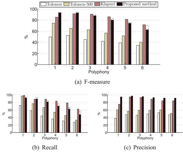
Fig. 7. Multipitch estimation results with unknown polyphony: for each algorithm, the F-measure, the precision and the recall are rendered as a function of the true polyphony. For the proposed method, the performance on the training set is plotted using a dashed line.
