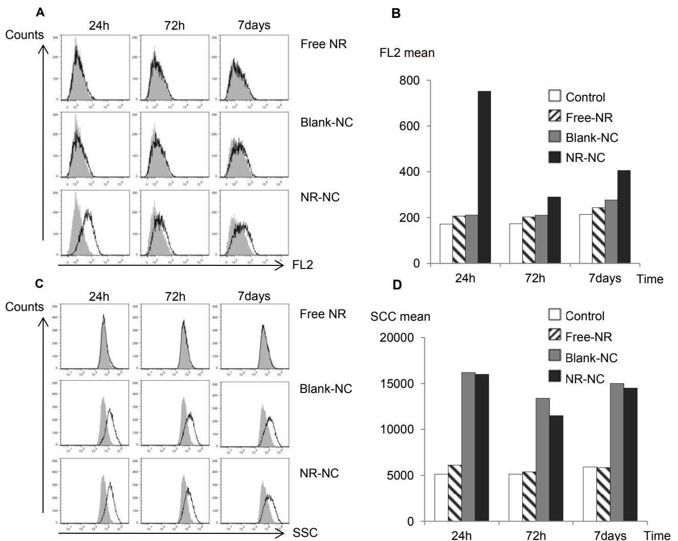
Figure 26 : In vitro uptake of NR labeled NC performed by flow cytometry. Non-treated BMM was used as control. Histograms show the mean of fluorescence intensity in FL2 channel (A and B), and the mean of side scattering channel intensity (C and D)
