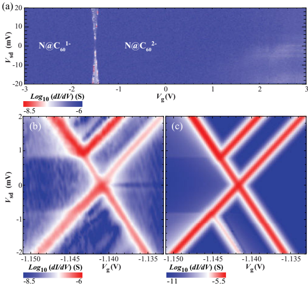
FIG. 2. (Color online) Color- (gray-) scale plot of the differential conductance dI/dV as a function of bias voltage V_{sd} and gate voltage V_g (a) on the entire accessible V_g range and (b) in the vicinity of V_g^D . (c) Numerical results obtained from Eqs. (4) and (5) for \epsilon_d = -3.1625 eV, U = 3.0 eV, J = -0.4 meV, C_g:C_R:C_L = 1:3.09:2.96 , and \Gamma_R/\Gamma_L \approx 10 .
