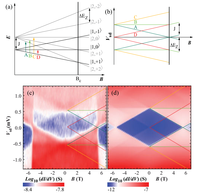
FIG. 4. (Color online) (a) Zeeman diagram of the multiplets S = 1 and 2 for N@C_{60}^{1-} ( n_{C_{60}} = 1 ). (b) Schematic showing the expected cotunneling steps. (c) Experimental and (d) numerical results, with J = -0.3 meV, of dI/dV for a fixed gate voltage V_g < V_g^D . Colored (different grayscale) lines indicate the positions of the magnetic excitations illustrated in (a) and (b).
