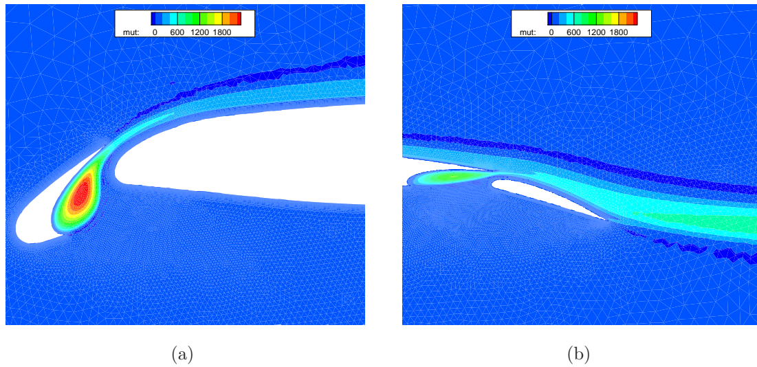
Figure 6.17: Zoom of the contours of the turbulent working variable near the leading (a) and trailing (b) of the airfoil
