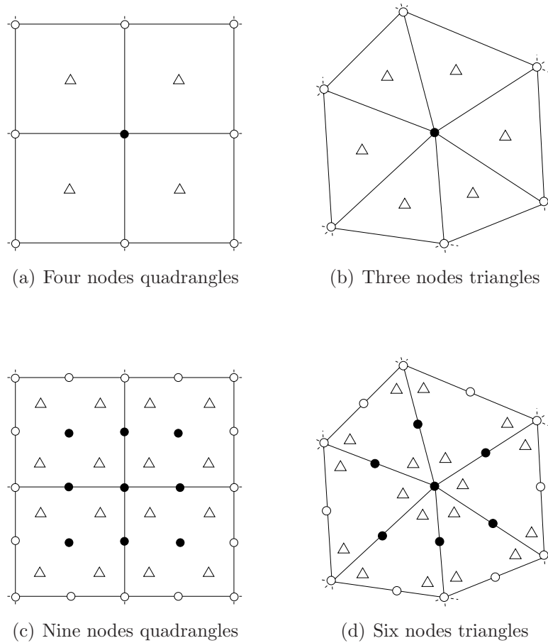
Figure 4.3: Interior super-convergent patches for quadrilateral and triangular elements: top linear elements, bottom quadratic elements. The symbols ( \circ ) indicate the patch assembly points, the symbols ( \bullet ) indicate the points where the gradient is reconstructed and the symbols ( \triangle ) indicate the super-convergent sampling points.
