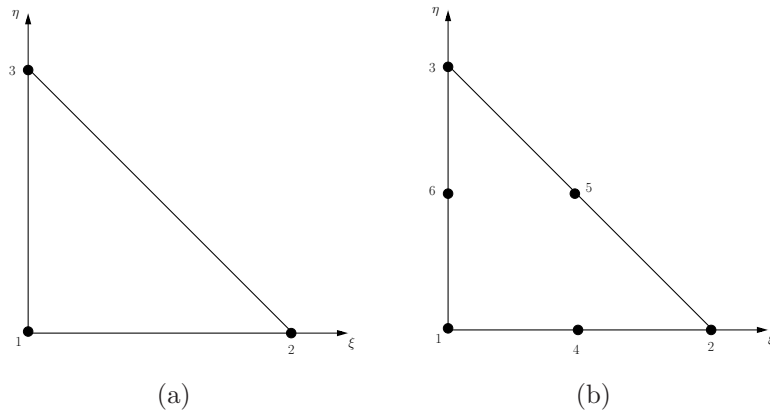
Figure 3.2: Reference triangular element for linear (a) and quadratic (b) approximations.
