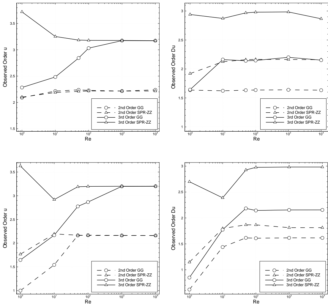
Figure 5.11: Observed orders of accuracy for the solution (left) and the gradient (right) in the manufactured solutions test, at different Reynolds numbers and with two type of gradient reconstruction. On the top row are reported the results for the linear scheme, on the bottom row are reported the results for the non-linear scheme.
