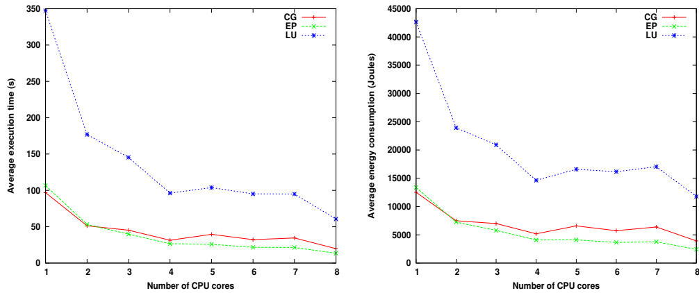
(a) Impact of the number of CPU cores available on workloads' performance. (b) Impact of the number of CPU cores available on workloads' energy consumption.
