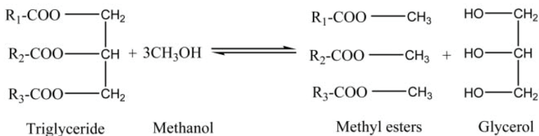
Scheme 1. Overall reaction for production of biodiesel through transesterification reaction of vegetable oils (from [18]).
