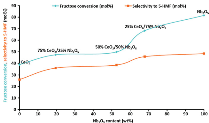
Fig. 12. Conversion of fructose and selectivity to 5-HMF as a function of Nb 2 O 5 loading, after 6 h of reaction.
