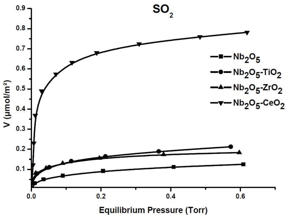
Fig. 7. Volumetric isotherms of \text{SO}_2 adsorption on investigated materials.
