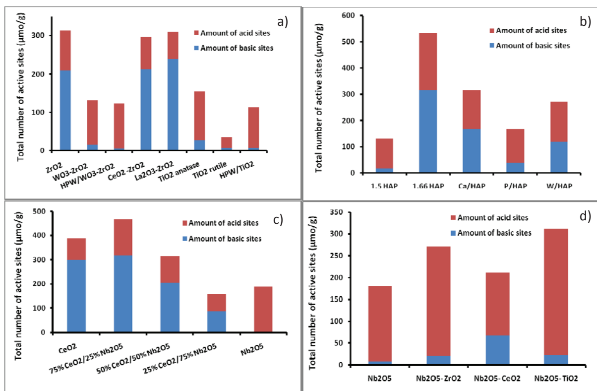
Figure 5.1. Histograms of amounts of acid and basic sites for each material investigated in this work.
