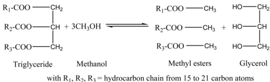
Scheme 1. Overall reaction for production of biodiesel through transesterification reaction of vegetable oils (from [18]).
