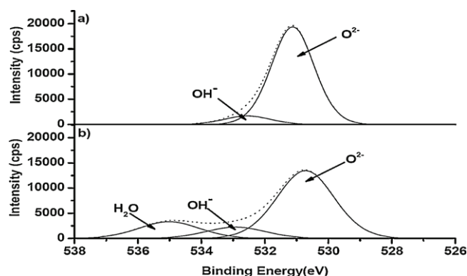
Fig. 9. XPS O 1s spectra of Ca/HAP sample (a) before reduction and (b) after reduction. Dotted lines present overall spectra, while solid lines correspond to specific surface species and have been obtained by deconvolution.
