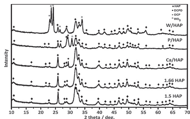
Fig. 1. Wide XRD patterns of investigated materials.
