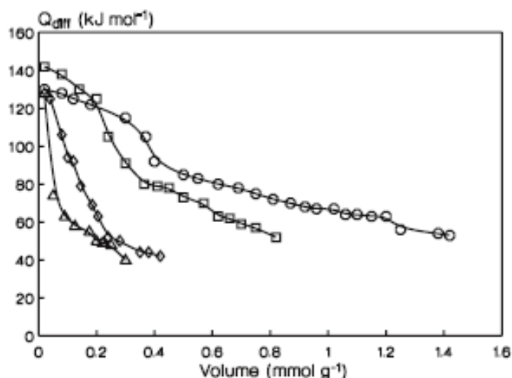
Fig. 9.12 Differential molar heats of ammonia chemisorption at 423K on MFI zeolites as a function of the adsorbed amount: \square Al-Sil, \circ Fe-Sil, \diamond In-Sil, \Delta silicalite. Pretreatment temperature 673 K ([135])
