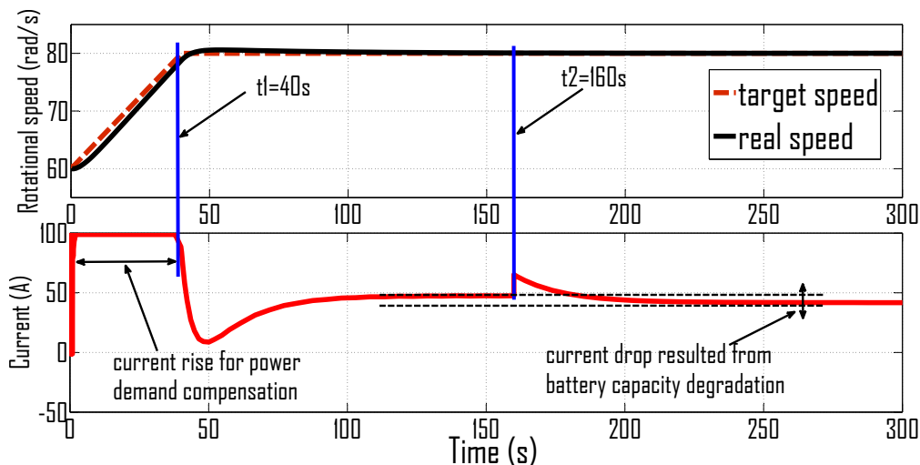
Figure 8.14: Battery current regulating
