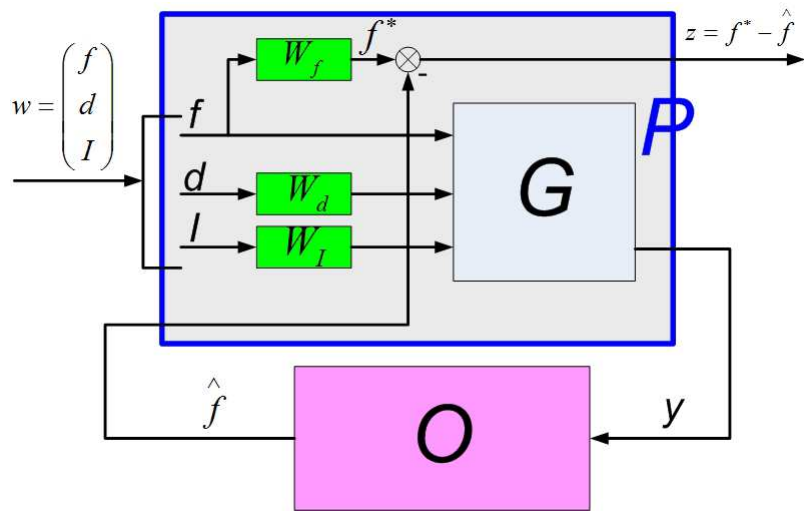
Figure 5.3: Observer scheme on standard H_\infty form
