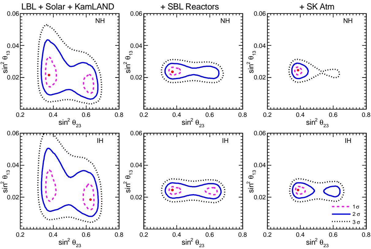
Figure 1.3: Results of the global analysis of neutrino masses, mixings and phases in the plane charted by (\sin^2\theta_{13}, \sin^2\theta_{23}) , all other parameters being marginalized away. From left to right, the regions allowed at 1, 2 and 3\sigma refer to increasingly rich datasets: LBL+solar+KamLAND data (left panels), plus SBL reactor data (middle panels), plus SK atmospheric data (right panels). Best fits are marked by dots. A preference emerges for \theta_{23} in the first octant [0, \frac{\pi}{4}] in both normal hierarchy (NH, upper panels) and inverted hierarchy (IH, lower panels)[27].
