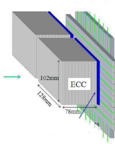
Figure 2.6: Sketch of ECC bricks associated with TT plane. The CSd in the blue box is attached to the downstream side of the ECC brick, so placed between the TT wall and the brick.
