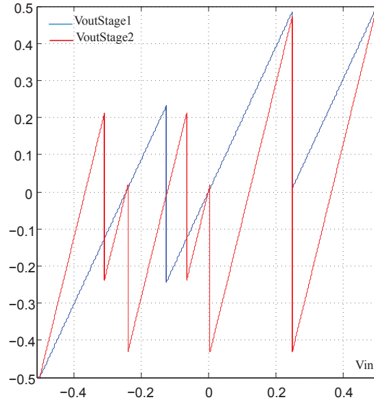
Figure 3.17: Residues of the first and second stages of 1.5-bit/stage pipeline ADC in the presence of errors.
