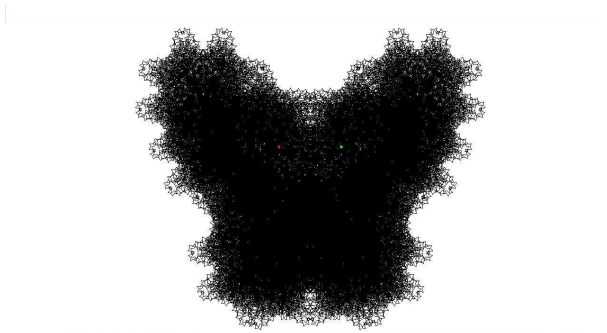
FIGURE 3.13 – \zeta = e^{\frac{3-2i\pi}{19}} .
