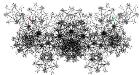
FIGURE 3.10 - \zeta = e^{\frac{2i\pi}{13}} .
