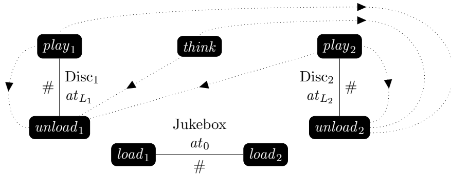
Figure 6.3: Conflict graph of the example from Figure 5.1.
