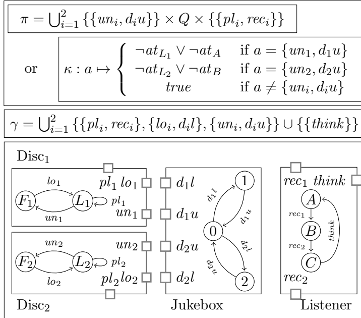
Figure 4.2: An example of abstract composition of 4 components using Interaction and either Priority or Condition.
