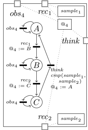
Figure 4.7: Observable version of the Listener component from Figure 4.6.
