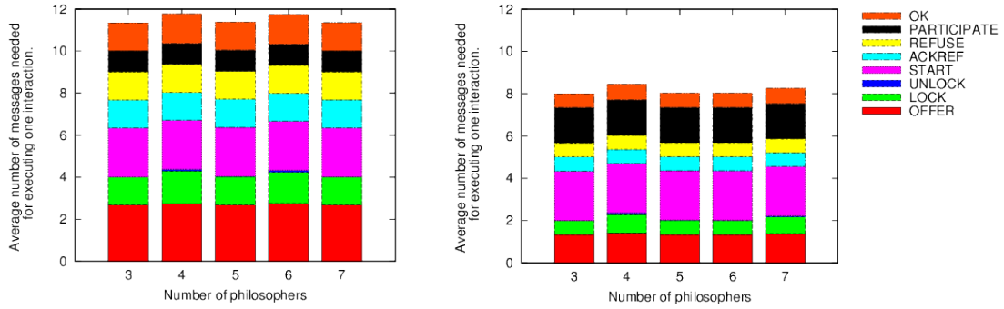
Figure 8.30: Dining philosophers: messages per interaction, standard version. Figure 8.31: Dining philosophers: messages per interaction, optimized version.
