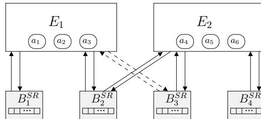
Figure 8.16: 3-layer Send/Receive BIP model for Bitonic Sorting Algorithm (6c).
