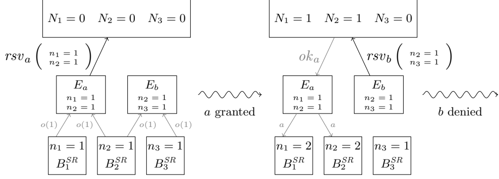
Figure 6.8: Principle of conflict resolution based on offer numbers.
