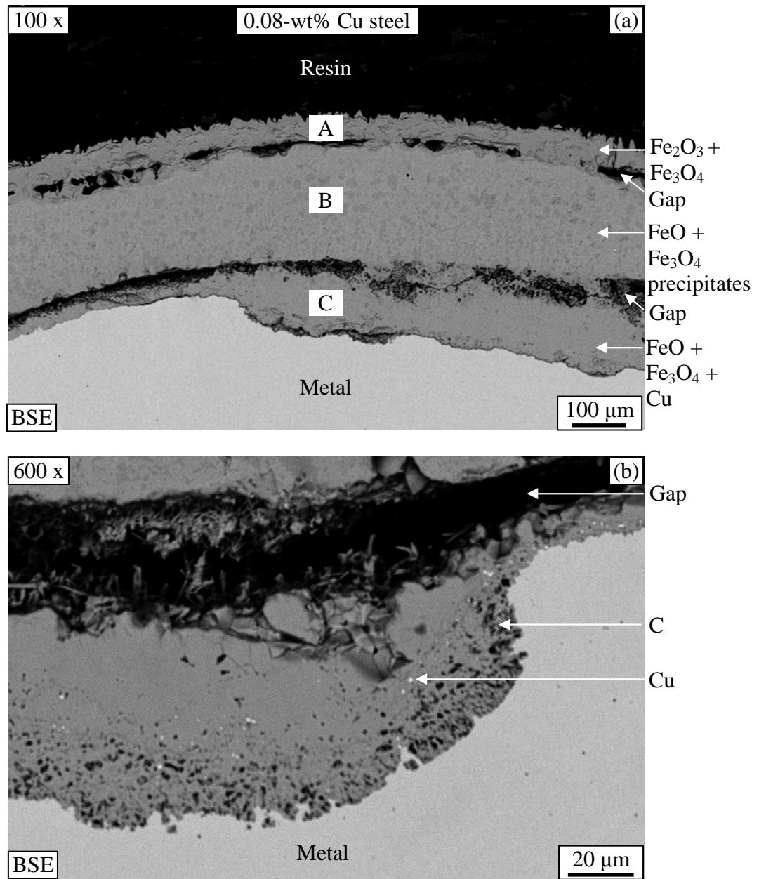
Figure 6.13: Cross-section of scale on the 0.08-wt% Cu steel oxidised in 20% H 2 O/Ar at 900°C for 16 h observed on (a) oxide scale, and (b) interface magnified from (a).
