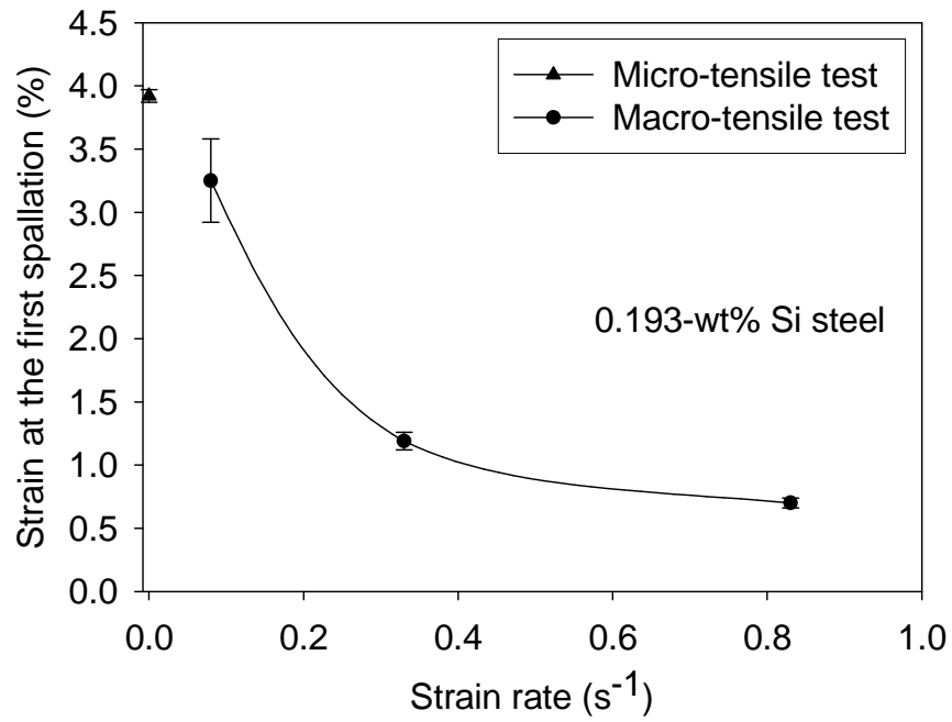
Figure 4.12: Strain at the first spallation of scale on the as-received hot-rolled 0.193-wt% Si steel as a function of strain rates.
