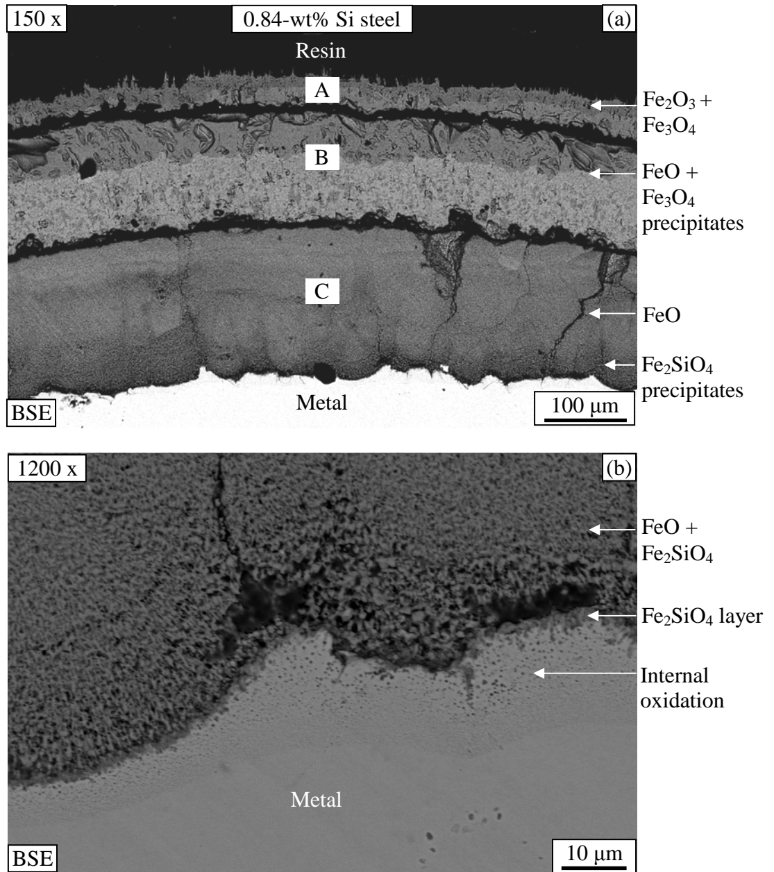
Figure 5.28: Cross-section of scale on the 0.84-wt% Si steel oxidised in 20% H 2 O/Ar at 900°C for 16 h showing (a) oxide scale, and (b) the interface magnified from (a).
