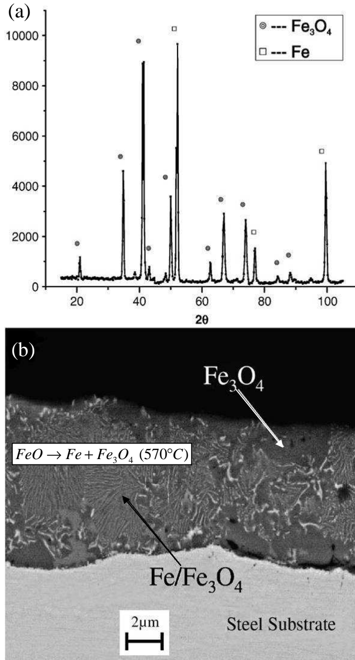
Figure 1.10: Oxide scale formed on the hot-rolled low carbon steel (a) XRD spectra, (b) SEM backscattered electron image of Fe/Fe _3\text{O}_4 eutectoid [Jie (2008)].
