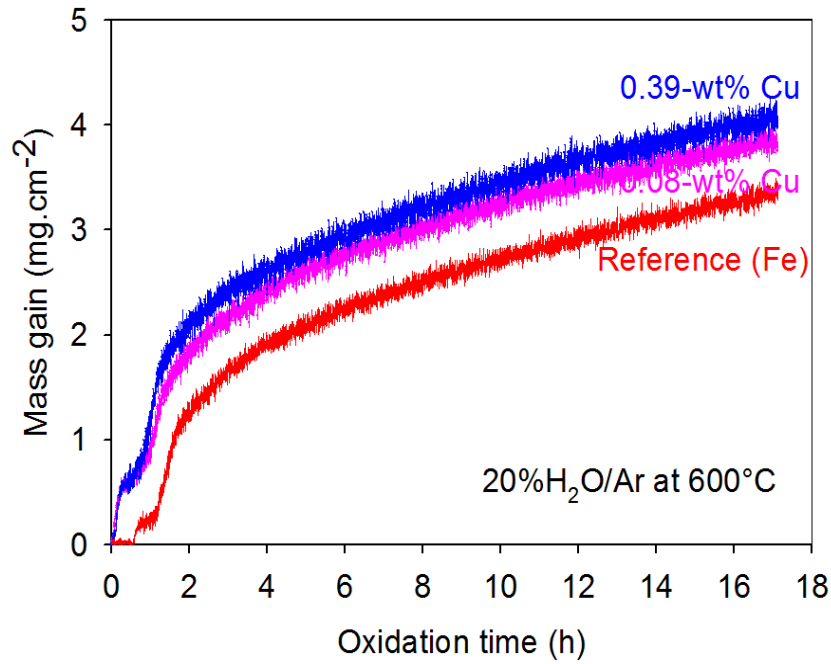
Figure 6.4: Mass gain of the reference steel (Fe), 0.08-wt% Cu and 0.39-wt% Cu steels oxidised in 20% H 2 O/Ar at 600°C.
