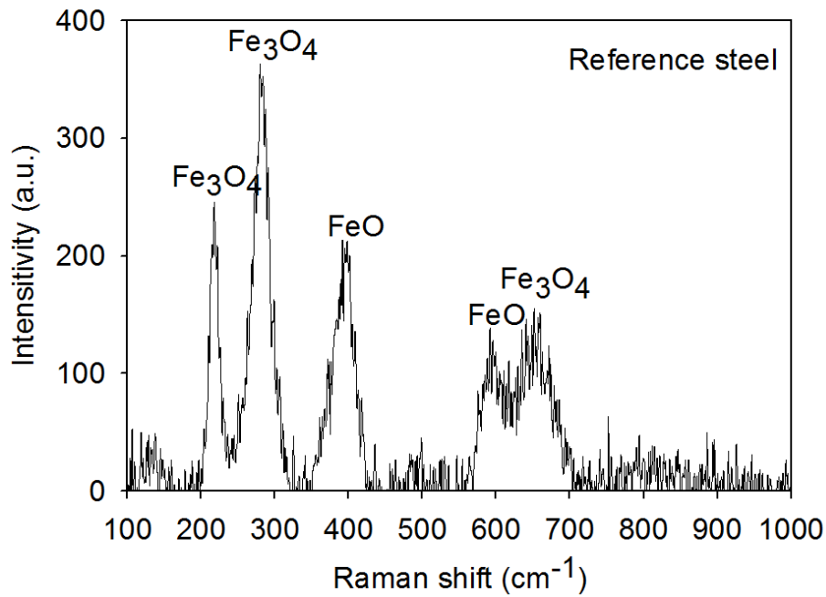
Figure 5.21: Raman peak on oxide scale observed on C in the Fig. 5.17 (a) of reference steel oxidised in 20% \text{H}_2\text{O}/\text{Ar} at 900°C for 16 h.
