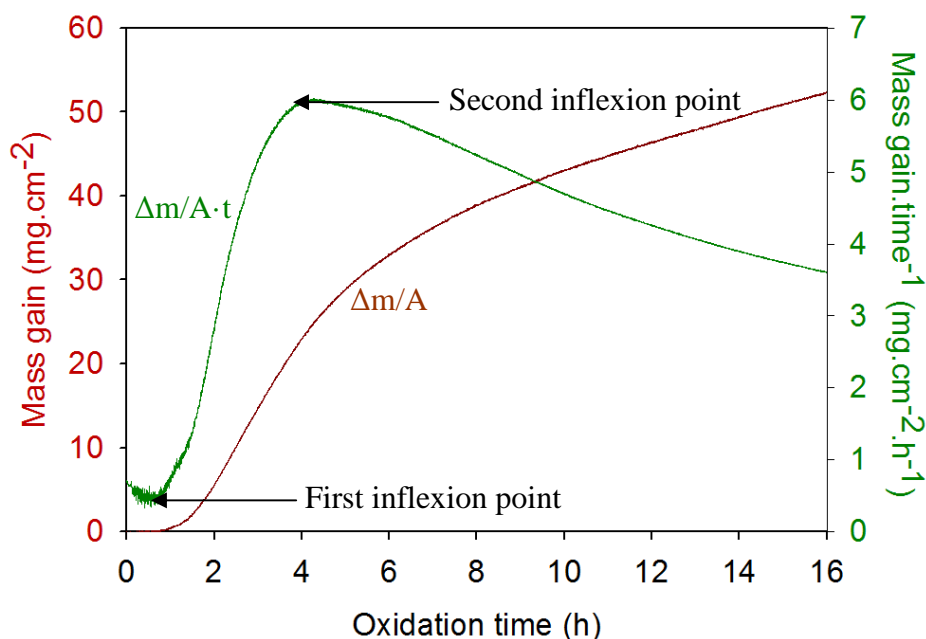
Figure 5.12: Derivative of mass gain in function of the oxidation time of the reference steel oxidised in 20% \text{H}_2\text{O}/\text{Ar} at 900^\circ\text{C} .
