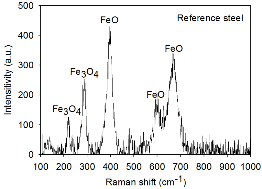
Figure 5.20: Raman peak on oxide scale observed on B in the Fig. 5.17 (a) of reference steel oxidised in 20% \text{H}_2\text{O}/\text{Ar} at 900°C for 16 h.
