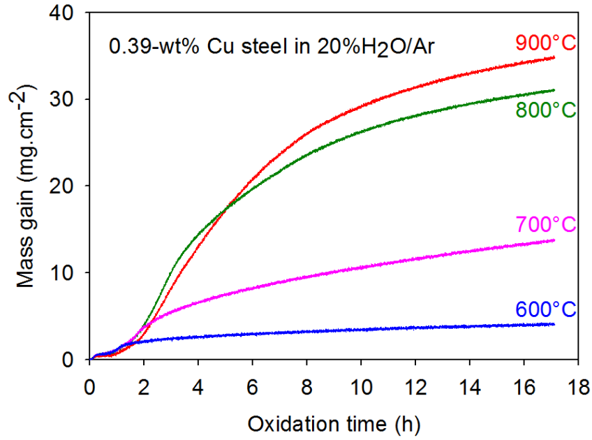
Figure 6.6: Mass gain of the 0.39-wt% Cu steel oxidised in 20% \text{H}_2\text{O}/\text{Ar} at different temperatures.
