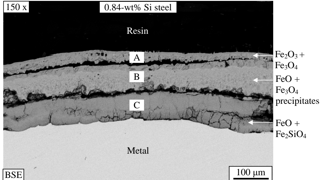
Figure 5.40: Cross-section of scale on the 0.84-wt% Si steel oxidised in 20% \text{H}_2\text{O}/\text{Ar} at 800°C for 16 h.
