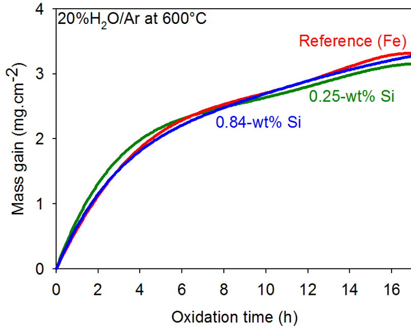
Figure 5.4: Mass gain of the reference (Fe), 0.25-wt% Si and 0.84-wt% Si steels oxidised in 20% \text{H}_2\text{O}/\text{Ar} at 600°C.
