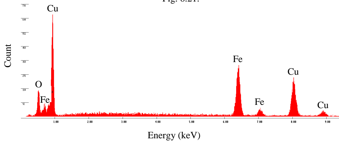
Figure 6.24: EDS pattern on oxide scale as Cu on scale near internal interface in the Fig. 6.21.
