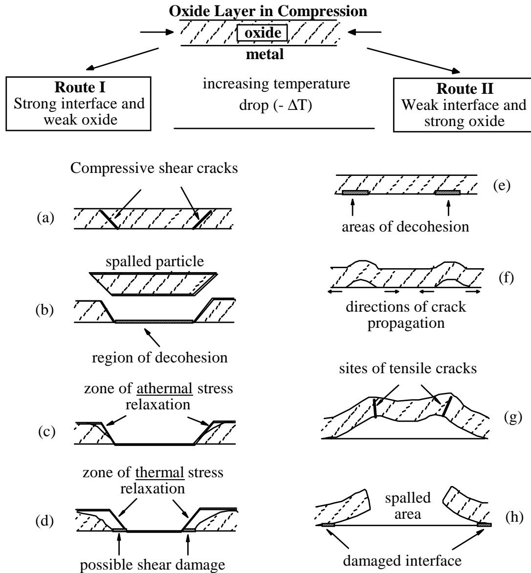
Figure 1.28: Cracking and spallation caused by compressive oxide stresses [Sarrazin (2000); redrawn from Evans (1995)].
