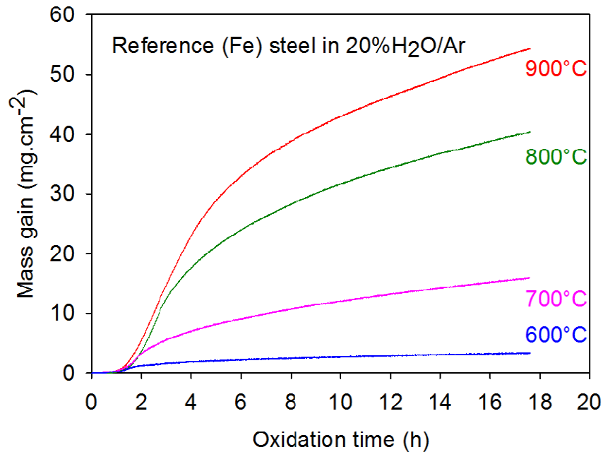
Figure 5.5: Mass gain of the reference (Fe) steel oxidised in 20% \text{H}_2\text{O}/\text{Ar} at different temperatures.
