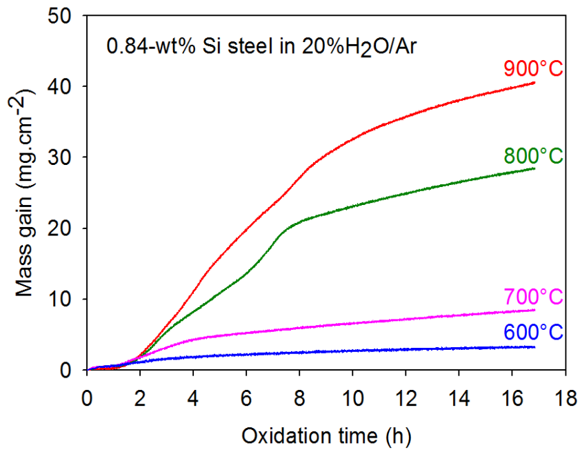
Figure 5.7: Mass gain of the 0.84-wt% Si steel oxidised in 20% \text{H}_2\text{O}/\text{Ar} at different temperatures.
