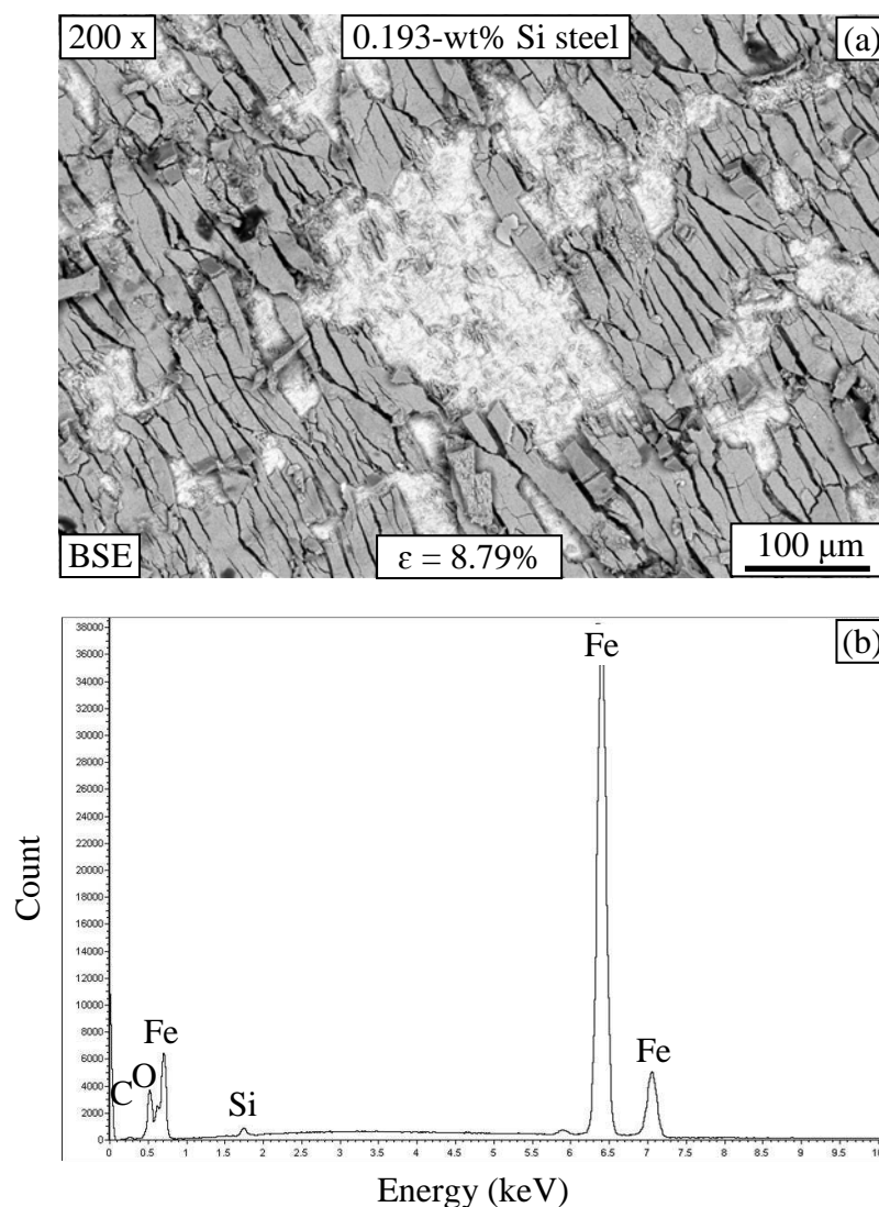
Figure 4.23: (a) Oxide scale and steel substrate of 0.193-wt% Si steel after the macro-tensile test, and (b) EDS pattern on metal substrate observed on the white area in the upper micrograph (a).
