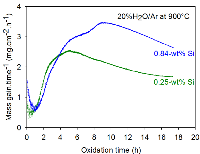
Figure 5.13: Derivative of mass gain in function of the oxidation time of silicon-containing steels oxidised in 20% \text{H}_2\text{O}/\text{Ar} at 900^\circ\text{C} .
