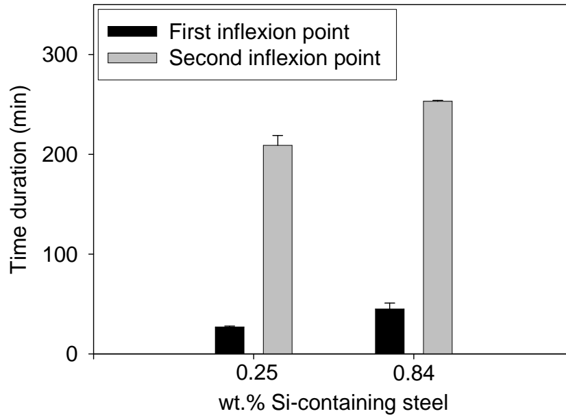
Figure 5.14: The first and second inflexion points of different silicon-containing steels oxidised in 20% H 2 O/Ar at 900°C.
