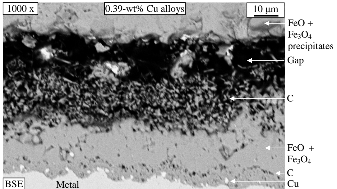
Figure 6.21: A metal-scale interface showing the carbon- and copper-rich phase in scale parallel to the metal-scale interface.
