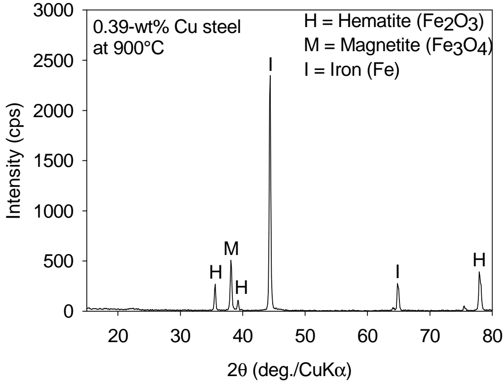
Figure 6.25: XRD pattern on oxide scale of the 0.39-wt% Cu steel oxidised in 20%H 2 O/Ar at 900°C for 16 h.
