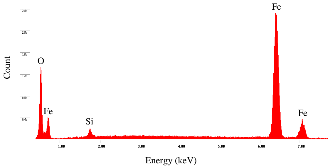
Figure 5.32: EDS pattern at the internal oxidation area in Fig. 5.28 (b).
