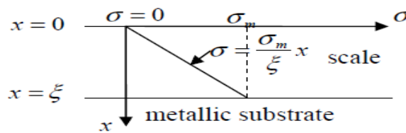
Figure 3.11: Schematic sketch of the linear distribution of stress in scale under tensile test [Chandra-ambhorn (2013)].
