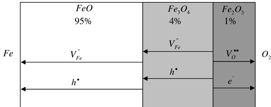
Figure 1.24: Vacancy diffusion for the growth of the three-layered oxide scale on iron [Sarrazin (2008)].
