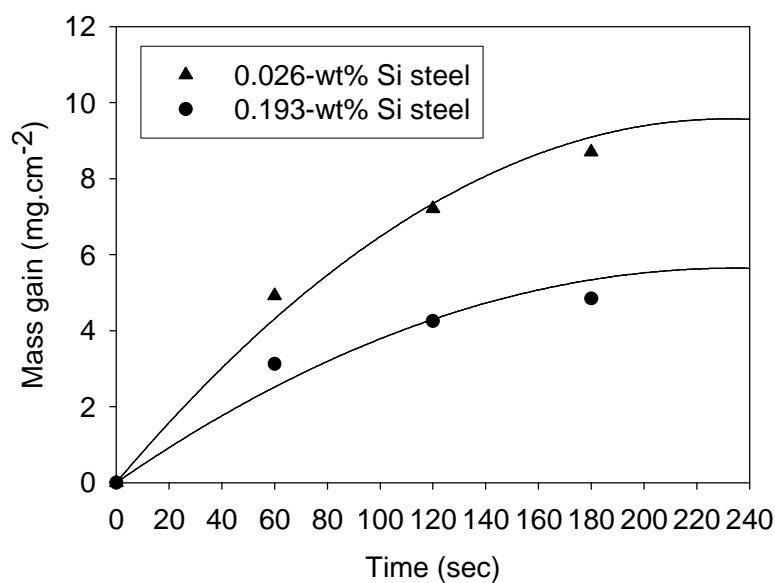
Figure 4.27: Mass gain as a function of the oxidising period of time of 0.026-wt% Si and 0.193-wt% Si steels in 20% \text{H}_2\text{O}/\text{Ar} .
