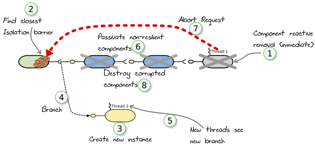
Figure 50: Reactive removal of an active component causes requests to be aborted. A ServiceUnavailableException is thrown when aborting a request. Dynamically-resilient components remain consistent and valid because they can recover, while non-resilient components are potentially corrupted by the exception and will be removed.
