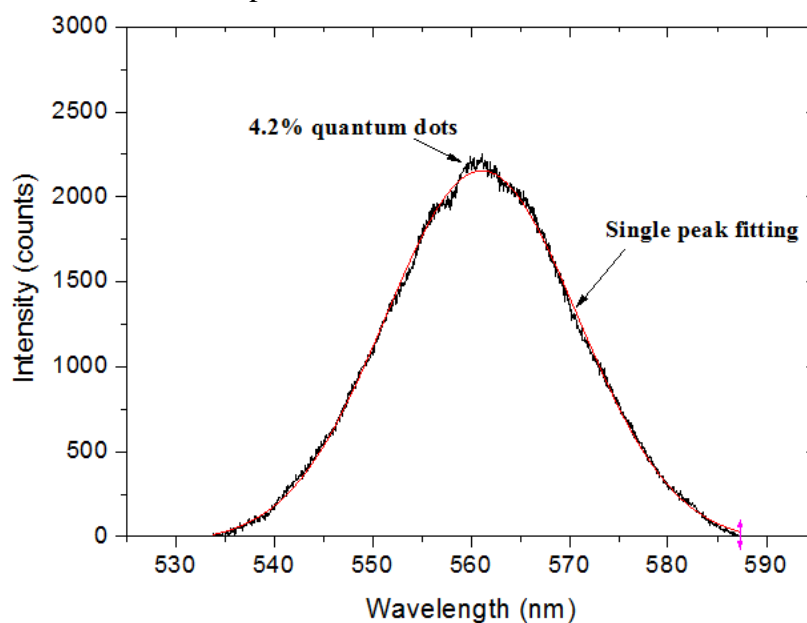
Figure 4.2.10: Luminescence of weight ratio percentage 4.2 % CdSe/ZnS QDs.
