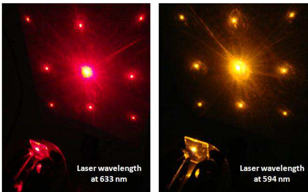
Figure 5.1.5: Periodic structure with good transfer. Left: Tunable laser at emission wavelength of 633 nm. Right: Tunable laser at emission wavelength of 594 nm.
