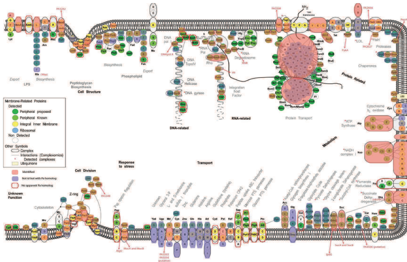
Figure 39 Comparison of the E. coli peripherome (Figure 38) and the results obtained in this study. Three protein categories have been identified and added to the figure legend. See the text for details.
