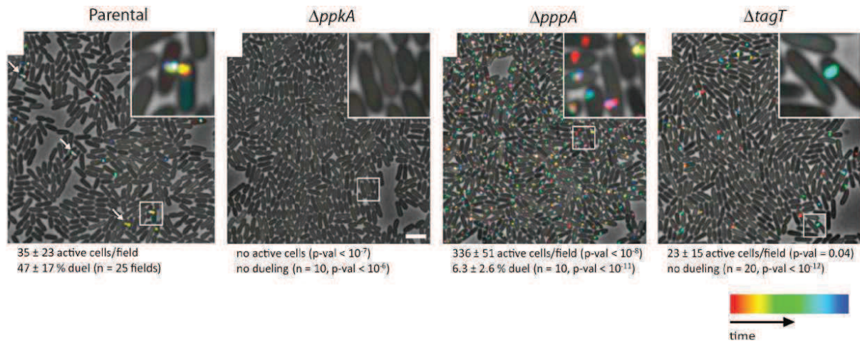
Figure 35 T6SS duelling depends on PpkA, PppA and TagT. ClpV1-GFP localisation was followed for 3min and temporally colour coded. The bar represents 3µm. n indicates the amount of fields analyzed; p value is compared to the parental strain. Adapted from Basler et al. (2013).
