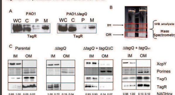
Fig5. A) Subcellular fractionation and immunodetection of TagR in PAO1 and PAO1ΔtagQ. WC: whole cells, C: cytosol, M: membrane fraction, P: periplasm. B) Representative discontinuous sucrose gradient samples. The IM (red, upper ring) and the OM (white, lower ring) are shown. Fractions were collected from the top and analyzed by WB and discovery mass spectrometry. C) Representative IM and OM markers. NADH oxidase activity (NADHox) and XcpY were used as IM markers. Porines were used as OM markers. Parental strain: PAO1.
