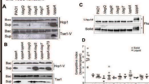
Fig2. Hcp1 and Tse1 production and secretion in Δtag (A) or ΔppkAΔtag strains (B) grown on liquid medium. C) Fla1 phosphorylation (marked with an asterisk) in solid and liquid medium. D) P. aeruginosa requires the tag genes for H1-T6SS-dependent fitness. The competitive index is plotted for competitions between each indicated donor strain and a H1-T6SS-susceptible recipient strain of P. aeruginosa . Bac: bacteria, sup: supernatant.
