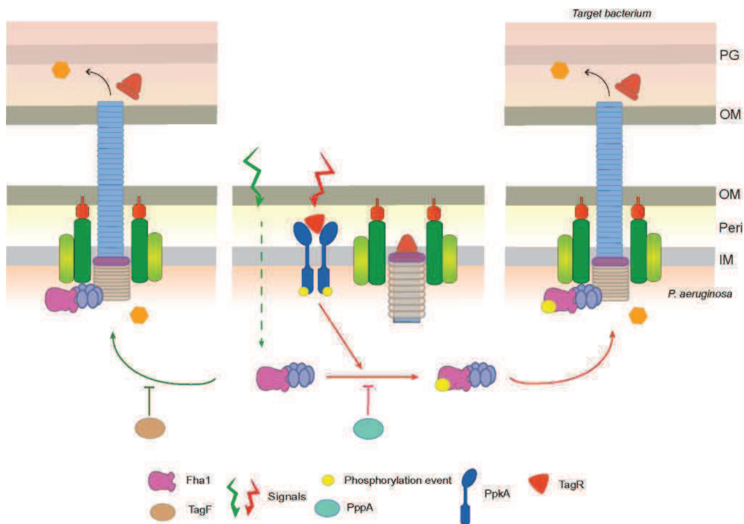
Figure 24 Schematic representation of the two posttranslational pathways that modulate H1-T6SS activity in P. aeruginosa . Red pathway: TPP. The environmental cue is associated with surface growth, that triggers dependent of TagR, PpkA dimerization and auto-phosphorylation. Green pathway: independent of TPP. The signal that derepresses TagF is unknown. Proteins not depicted in the legend have already been described in Figure 20 (Chapter III).
