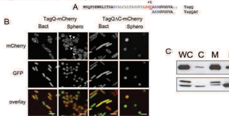
Fig3. A) The IpoBox of TagQ is shown in red. The underlined C is the conserved C that has been deleted in TagQΔC. B) TagQ is an OM lipoprotein. GFP-expressing P. aeruginosa bacteria and spheroplasts expressing TagQ-mCherry or TagQΔC-mCherry were analyzed using laser scanning confocal microscopy. Arrows indicate the OM. Bact: bacteria, Sphero: spheroplasts. The bar represents 2 \mu m . C) Subcellular separation and immunoblotting of TagQ in PAO1 \Delta tagQ expressing either TagQ (WT) or TagQΔC ( \Delta C ). The asterisk indicates the partial cleavage of TagQΔC. WC: whole cells, C: cytosol, M: membrane fraction, P: periplasm.
