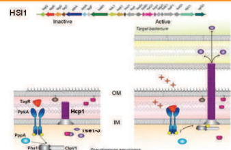
Fig1. Posttranslational activation of H1 T6SS of P. aeruginosa . The putative signal is represented with red stars. Inner membrane (IM) and outer membrane (OM) of P. aeruginosa and the target bacterium are shown. Tse1-3 are T6S exported effectors.
