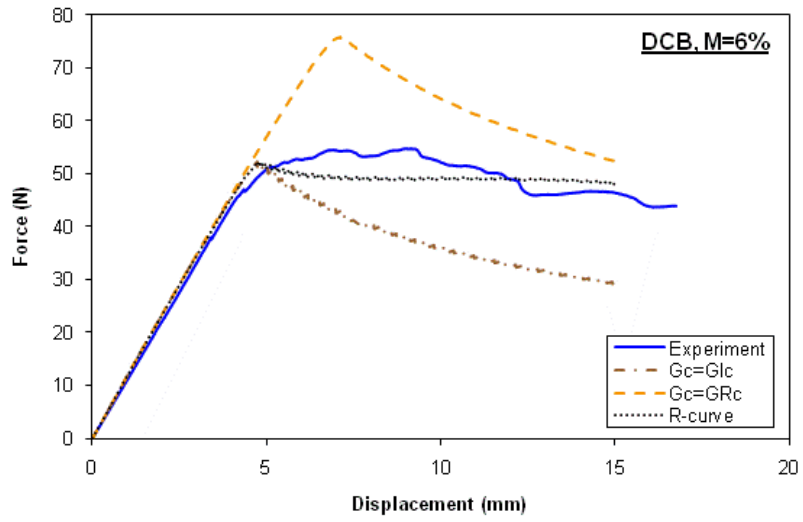
(a) DCB
