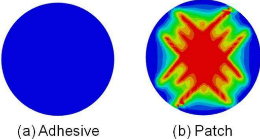
Figure 6.20: Damage in the adhesive and the patch of ARA-sp repair using ENF CDM parameters.
