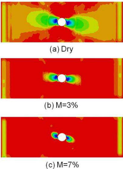
Figure 7.9: Extension of matrix tension damage initiation at peak load in layer 1 (L1 with 45° fibres) at different moisture levels.
