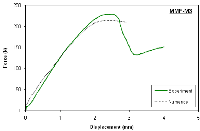
(c) MMF
