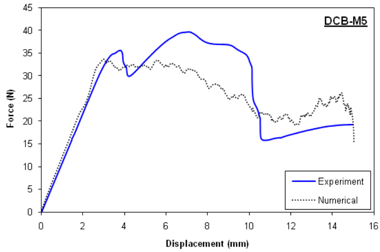
(a) DCB
