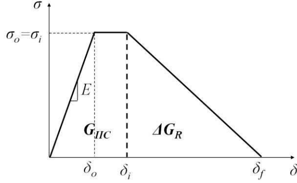
Figure 5.15: Linear bridging law for mode II R-curve modelling.
