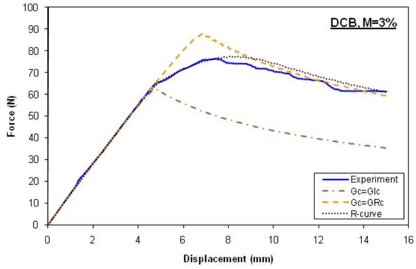
(a) DCB
