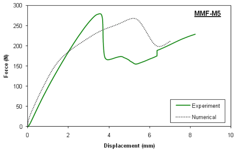
(c) MMF
