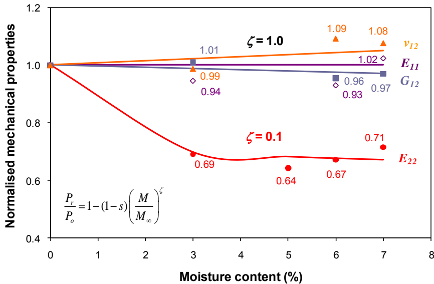
Figure 4.16: Normalised experimental and refitted (using Equation (4.9)) modulus and Poisson's ratio of T600S/R368-1 composite laminates at various moisture content levels.
