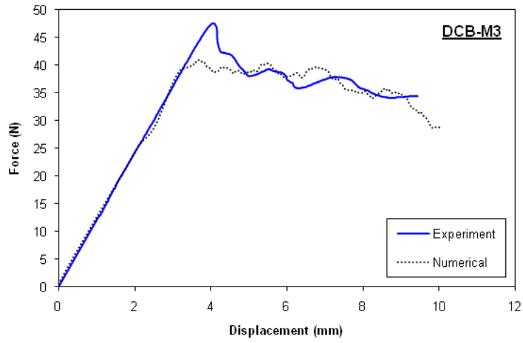
(a) DCB
