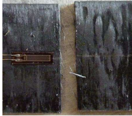
Figure 4.10: Failure mode of transverse specimens: matrix cracking across the width with some fibre peeling
