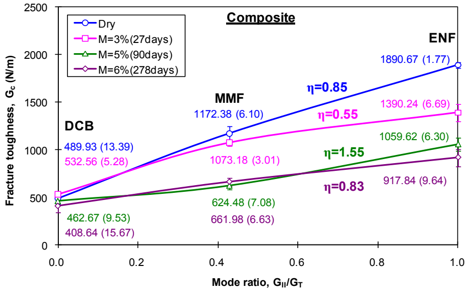
Figure 4.13: Mode I, II and mixed-mode I+II fracture toughness of unidirectional carbon/epoxy composites at different moisture content levels.
