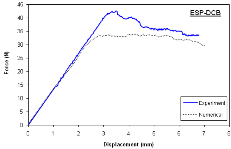
(a) DCB
