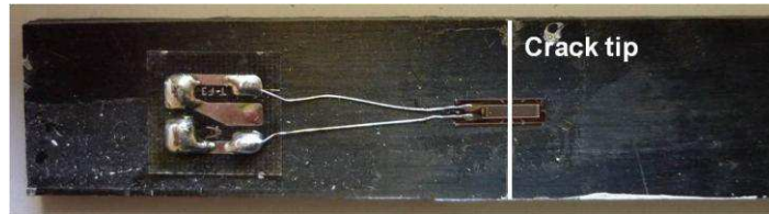
Figure 5.2: Location of strain gauge attached on upper adherend of an ENF specimen.
