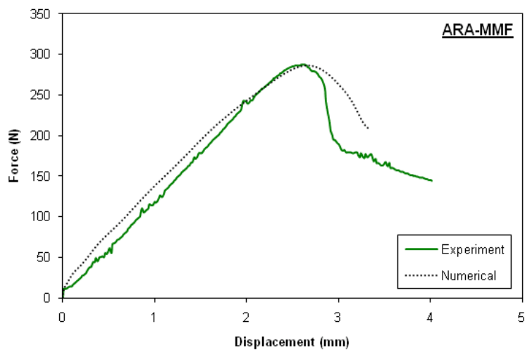
(c) MMF
