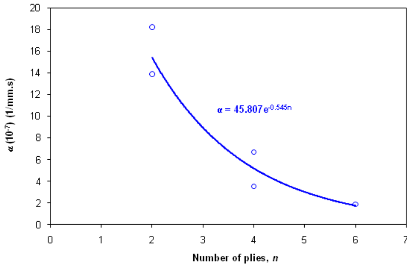
Figure 3.10: Experimental and fitted \alpha relationship with number of plies for 170\text{g/m}^2 composite laminates.
