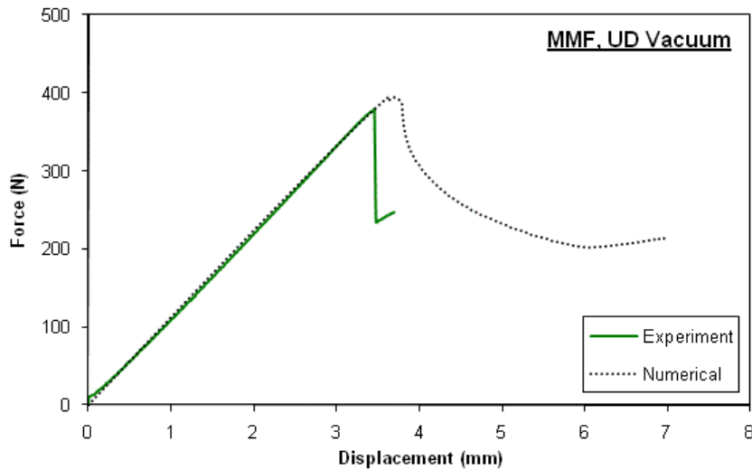
(c) MMF
