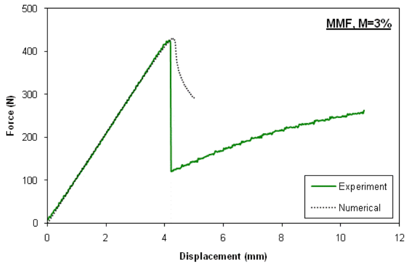
(c) MMF
