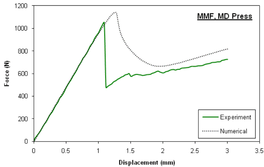
(c) MMF
