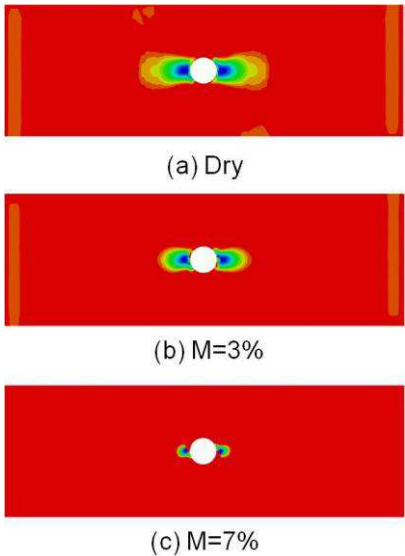
Figure 7.10: Extension of matrix tension damage initiation at peak load in layer 2 (L2 with 90° fibres) at different moisture levels.
