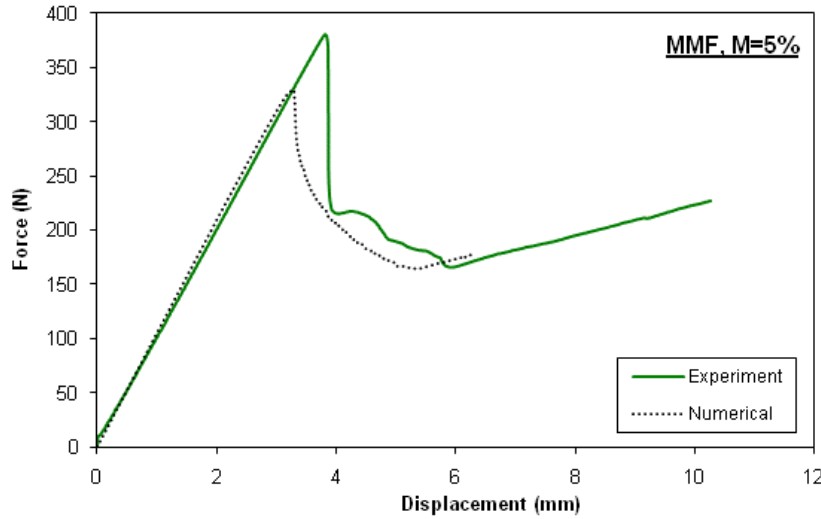
(c) MMF
