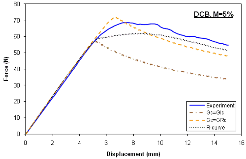
(a) DCB
