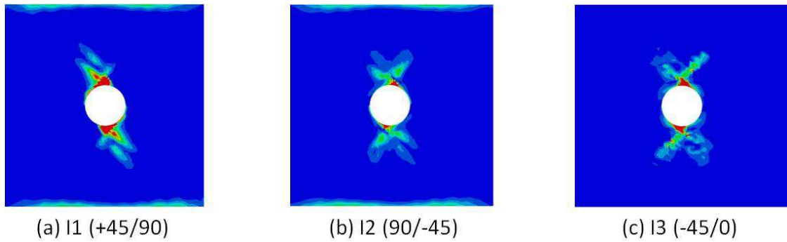
Figure 6.17: Interface delamination at peak load.
