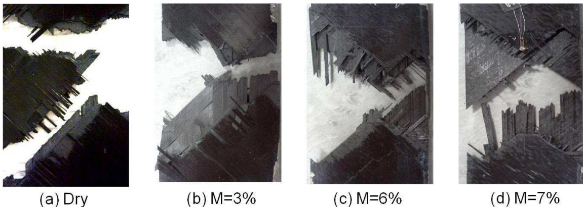
Figure 7.4: Fractured unnotched specimens at various moisture content levels.
