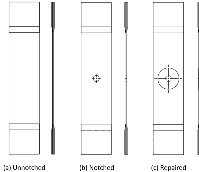
Figure 6.1: Configurations of unnotched, notched and repaired specimens.
