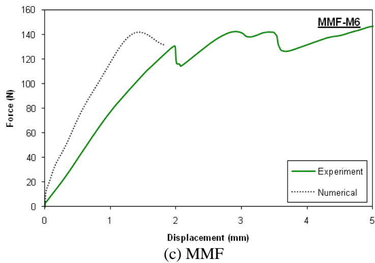
Figure 5.22: Experimental and numerical force-displacement curves of Araldite2015 bonded specimens at M=6\% .
