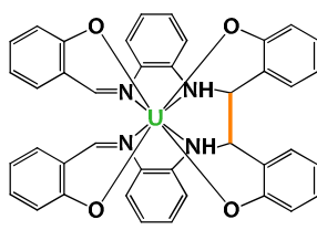
[\text{U}(\text{bis-H}_2\text{salophen})] 9
