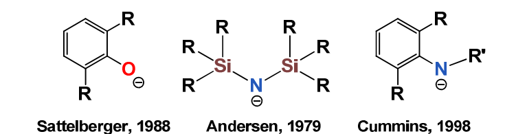
Figure I.5. Monodentate O and N-donor ligands for U(III) chemistry. 91, 92, 95
