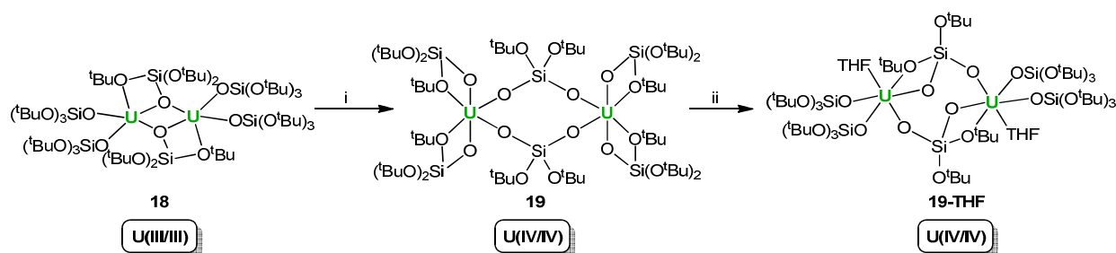
Scheme III.3. Decomposition of the U(III)/U(III) [U(OSi(O^tBu)_3)_2(\mu-O_2Si(O^tBu)_2)]_2 complex 18 i) solid state, r.t. 7 days or 80^\circ\text{C} 30 min ; ii) THF, r.t.
