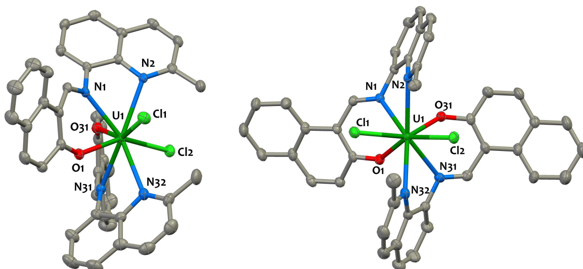
Figure II.41. Side and top views of the solid-state molecular structure of [UCl 2 ( Me naphtquinolen) 2 ], 14-Cl . Hydrogen atoms and solvent molecules are omitted for clarity. Uranium (deep green), nitrogen (blue), oxygen (red), chlorine (light green) and carbon (grey) atoms are represented with 50% probability ellipsoids. Selected bond distances are given in Table II.8 .
