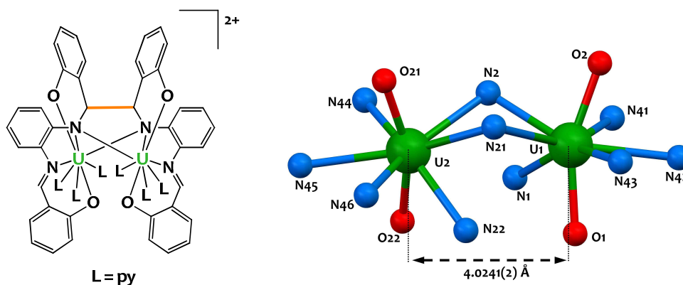
Figure 11.29. Schematic representation (left) and view of the core (right) of complex [U_2(\text{bis-salophen})(\text{py})_6]I_2 11-I .
