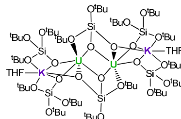
[K(\text{THF})U(\text{OSi}(\text{O}^t\text{Bu})_3)_2(\mu\text{-O}_2\text{Si}(\text{O}^t\text{Bu})_2)_2] 21
