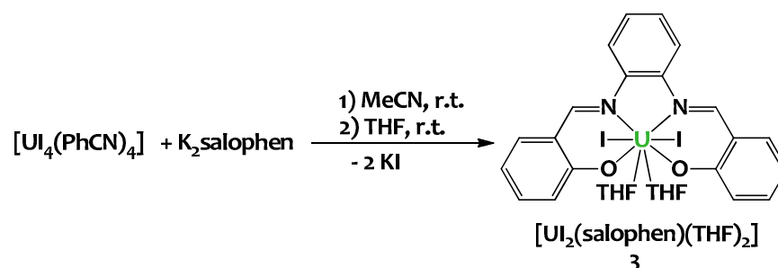
Scheme II.7. Synthesis of the heteroleptic U(IV) complex [\text{U}_2(\text{salophen})(\text{THF})_2] 3 by salt metathesis from the tetravalent uranium precursor [\text{U}_4(\text{PhCN})_4] .
