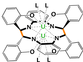
[\text{U}_2(\text{cyclo-salophen})(\text{L})_4] 4-THF (L = THF) 4-py (L = pyridine)
