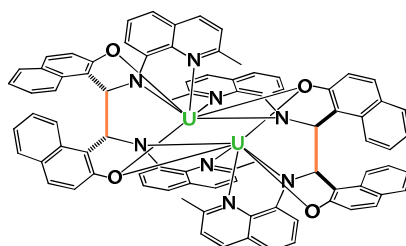
[U(\mu\text{-bis-Me-naphthquinolen})_2] 15
