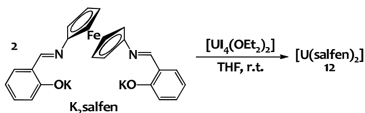
Scheme II.24. Synthesis of [\text{U}(\text{salfen})_2] 12 .
