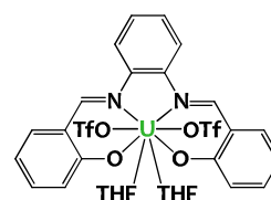
[U(salophen)(OTf)_2(THF)_2] 8
