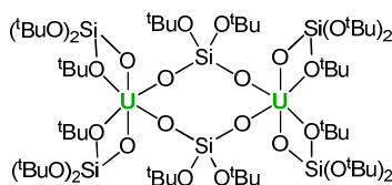
[U(\text{OSi}(\text{O}^t\text{Bu})_3)_2(\mu\text{-O}_2\text{Si}(\text{O}^t\text{Bu})_2)_2] 19
