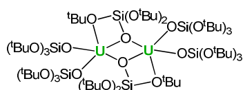
[U(\text{OSi}(\text{O}^t\text{Bu})_3)_2(\mu\text{-OSi}(\text{O}^t\text{Bu})_3)_2] 18
