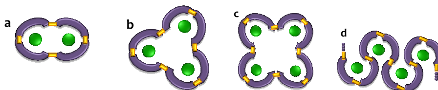
Figure II.25. Schematic representation of possible oligomeric complexes resulting from reductive coupling of imino moieties in Na 2 [U(bis-salophen)] 7 . Uranium is represented as a green sphere, the ligand is represented in gray and the C-C bridging bonds in yellow.
