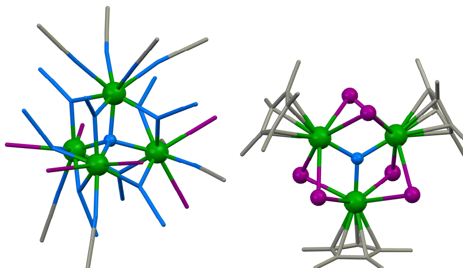
Figure I.12. Mercury diagrams of the solid-state molecular structures of the uranium nitrido clusters ([U_4(\mu^4-N)(\mu-1,1-N_3)_8(CH_3CN)_8]I_6)[(Cs(CH_3CN)_3)]_n (left) and [U(Cp^*)(\mu-1)_2]_3(\mu^3-N) (right).
