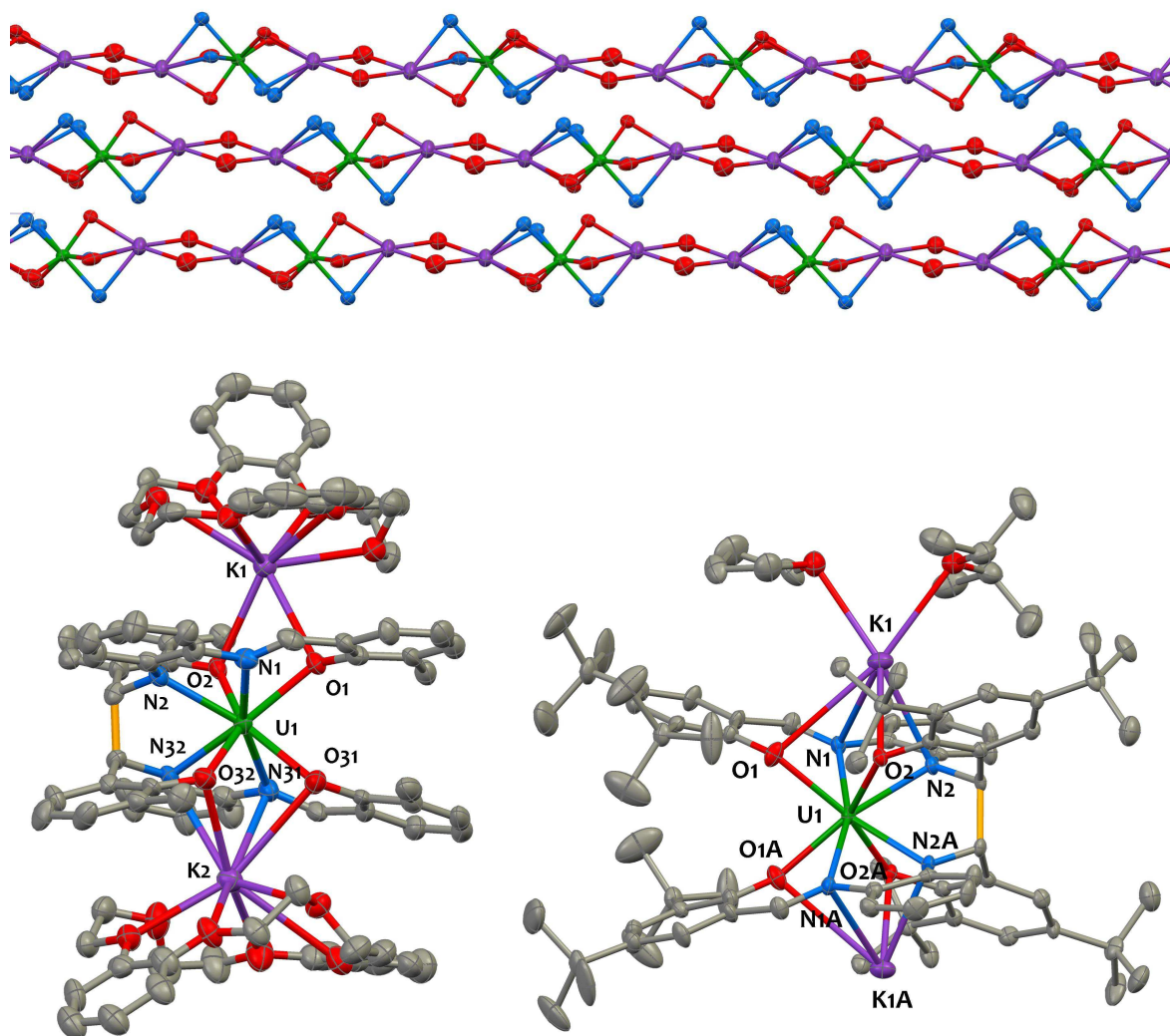
Figure II.18. Top : Mercury view of the 1-D polymeric network in 7-tBu . Only U, K, N and O atoms are presented for clarity. Bottom : Solid-state molecular structure of [K(\text{dibenzo18c6})]_2[U(\text{Me})\text{bis-salophen}] 7-Me-dibenzo18c6 (left) and K_2[U(\text{tBu})\text{salophen}]_2 \cdot (\text{THF}) \cdot (\text{DIPE}) 7-tBu (right). Hydrogen atoms and disorder are omitted for clarity. Uranium (green), potassium (purple), nitrogen (blue), oxygen (red) and carbon (grey) atoms are represented with 50% probability ellipsoids. The C-C bond bridging the two original salophen units is represented in yellow. Selected bond distances are given in Table II.2 .
