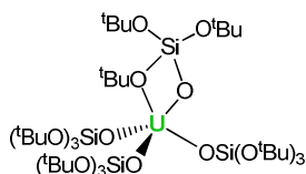
[U(\text{OSi}(\text{O}^t\text{Bu})_3)_4] 23
