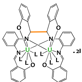
[U_2(bis-salophen)(py)_6] L = py 11
