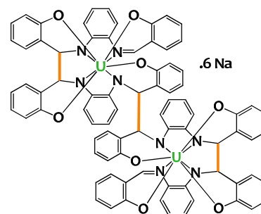
Na_6[U_2(bis(bis-salophen))] 10
