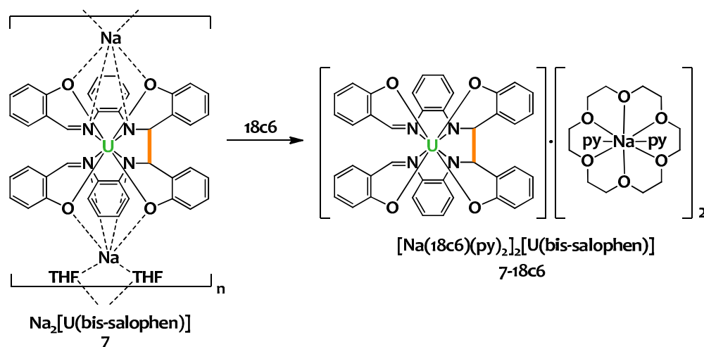
Figure II.15. Addition of 18c6 to a pyridine solution of 7 prevents the coordination of the alkali cation to the ligand and affords the ion pair [\text{Na}(\text{18c6})(\text{py})_2]_2[\text{U}(\text{bis-salophen})] 7-18c6 .
