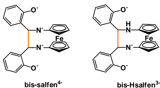
Figure II.35. Drawing of ligands bis-salfen 4- and bis-Hsalfen 3-
