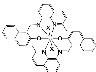
[UX_2(\text{Me-naphthquinolen})_2] X = Cl, I 14-X
