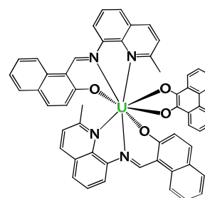
[U(9,10\text{-phenanthrenediol})(\text{Me-naphthquinolen})_2] 16
