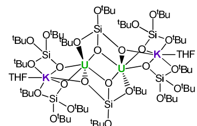
[K(\text{THF})U(\text{OSi}(\text{O}^t\text{Bu})_3)_2(\mu\text{-O}_2\text{Si}(\text{O}^t\text{Bu})_2)_2] 21
