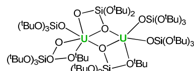
[U_2(\mu\text{-O}_2\text{Si}(\text{O}^t\text{Bu})_2)(\mu\text{-OSi}(\text{O}^t\text{Bu})_3)(\text{OSi}(\text{O}^t\text{Bu})_3)_4] 20
