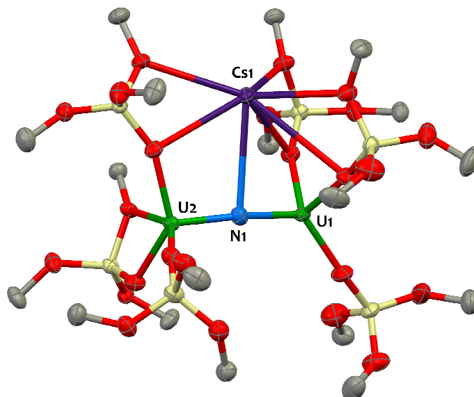
Figure III.40. Solid-state molecular structure of \text{Cs}\{[(\mu\text{-N})[\text{U}(\text{OSi}(\text{O}^t\text{Bu})_3]_2)]\} 32 , crystallized from a saturated hexane solution. Hydrogen atoms and methyl groups are omitted for clarity. Uranium (green), silicon (yellow), cesium (purple), nitrogen (blue), oxygen (red) and carbon (grey) atoms are represented with 50% probability ellipsoids. Selected bond distances [Å] and angles (deg): U1-N1 2.058(5), U2-N1 2.079(5), U1-O - avg 2.183(14), U2-O - avg 2.19(3), U2-O t Bu 2.713(4), U2-O - avg 2.19(3).
