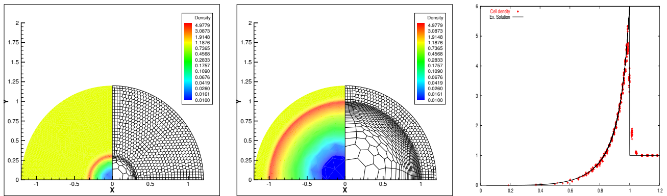
FIGURE 2.5 – Numerical results from paper [8]. Sedov problem on polygonal Mesh —Sedov blast wave on a polygonal mesh (1325 nodes and 775 cells). ALE-10 regime — Left-Middle : mesh and density contours (exponential scale) at t = 0.1 and t = 1.0 . Right : density at t = 1.0 (cell-based value as a function of the radius)
