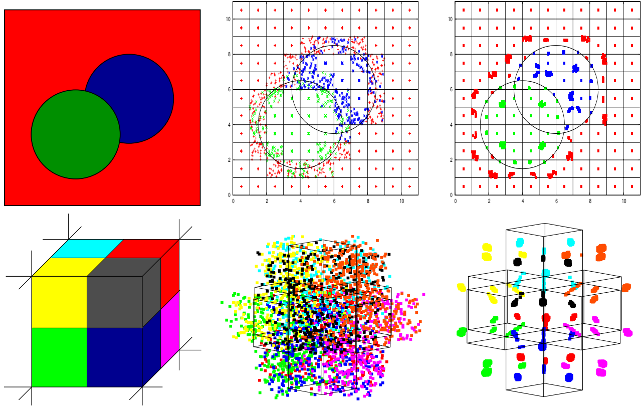
FIGURE 2.20 – Numerical results obtained with the particle attraction model to infer the relative location of the materials in mixed cells. Top panels : two enclad disks (left panel) are described by particles which are randomly distributed with mixed cells (middle). At convergence of the particle model (right panel) particles do represent an accurate approximation of the material centroids — Bottom panels : approximation for 3D eight materials case (zoom on the central 8 materials mixed cell on the left panel), initial distribution of particles in the neighborhood of the central mixed cell (middle panel) and final location of particles in the enighborhood (right panel).
