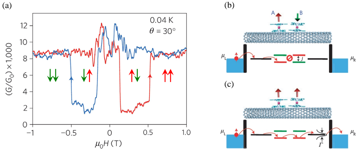
Figure 2.22: Spin valve behaviour in a supramolecular spintronic device based on a carbon nanotube quantum dot functionalized with \text{TbPc}_2 SMM's. Figures from [48] (a) Butterfly hysteresis loop at T = 40 mK. (b) Antiparallel spin configuration. The spin states are inverted in the dot A and the energy mismatch between levels with identical spin results in a current blockade. (c) Parallel spin configuration for both molecules A and B. Energy levels with same spin are aligned allowing electron transport through the carbon nanotube.
