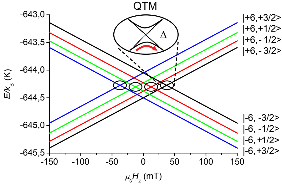
Figure 2.14: Zeeman diagram for the ground state multiplet J = 6 in a TbPc 2 SMM. Avoided level crossings are highlighted by the black circles. The enlarged region shows an avoided level crossing with tunnel splitting \Delta caused by the mixing of the m_J = -6 and m_J = +6 states. The dotted lines show the two states without mixing and the red arrows depict the QTM process.
