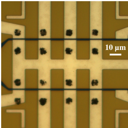
Figure 4.12: Impact of catalyst concentration: (a) Low catalyst density results almost exclusively in single tube devices, but to a very low yield of \eta_{\text{tot}} \sim \eta_1 \sim 1\% . (b) Higher catalyst density increases the yield for single tube devices \eta_1 \sim 5\% , but also results in multiple tube devices and a higher overall yield of \eta_{\text{tot}} . The images in the right column are false color SEM images with the localgate colored in blue and the source-drain junction in gold. The contrast was enhanced for better visibility of the carbon nanotubes.
