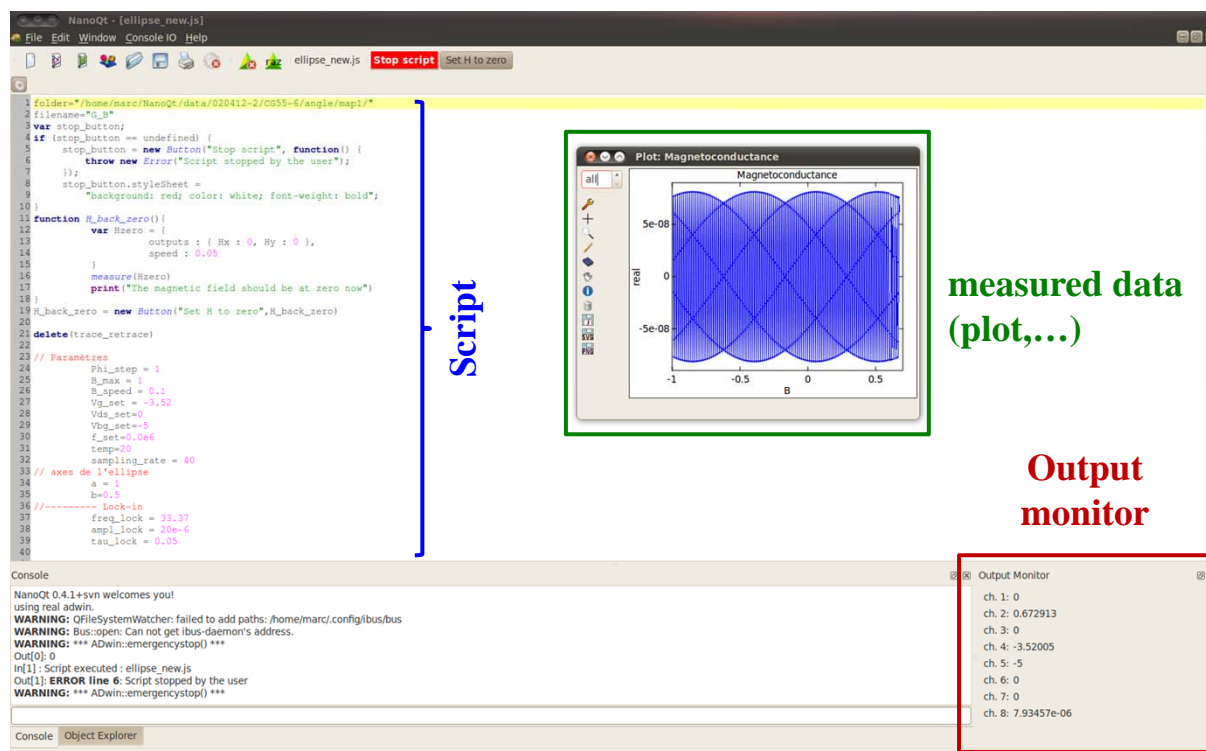
Figure 4.15: User interface NanoQt: A measurement sequence is defined in a script (Javascript) and sent to the ADWIN DSP which generates the desired signals. The output can be monitored in real time. The response of the sample is recorded by the ADWIN and the data sent back to the NanoQT interface, where it is displayed in real time in a separate graph window (green).
