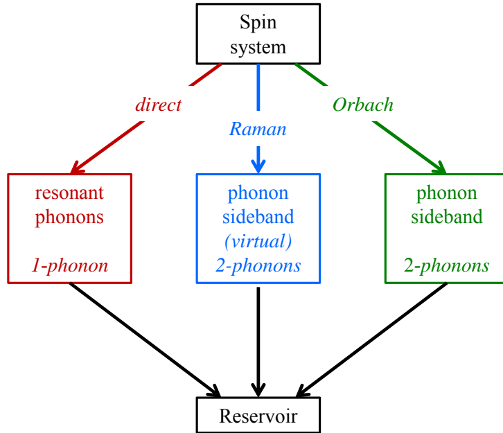
Figure 6.3: Spin-phonon relaxation processes in TbPc 2 * single molecule magnets: A direct one-phonon process dominates at lowest temperatures, whereas two-phonon Orbach and Raman processes take over as the temperature increases. The phonon energy is then transferred to a thermal reservoir. The arrows indicate the direction of the energy transfer. Figure inspired from [50].
