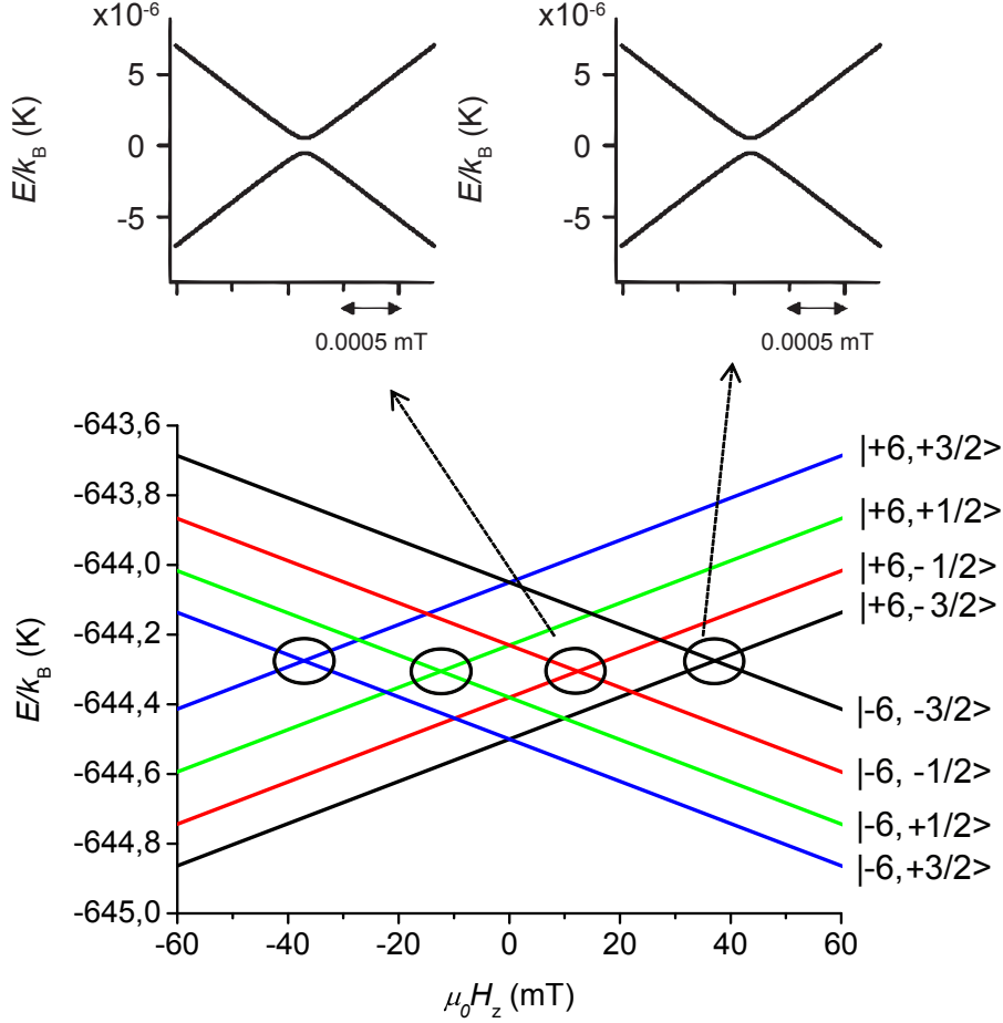
Figure 2.12: Calculated Zeeman diagram for the ground state multiplet J = 6 in a \text{TbPc}_2 SMM extracted from [49]. The black circles highlight the avoided level crossing.
