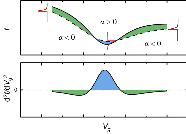
Figure 3.17: Nonlinearity modulation by single-electron tunneling in a carbon nanotube NEMS. The sign of \alpha_{SET} follows the curvature \frac{d^2f}{dV_g^2} of the frequency modulation induced by SET.
