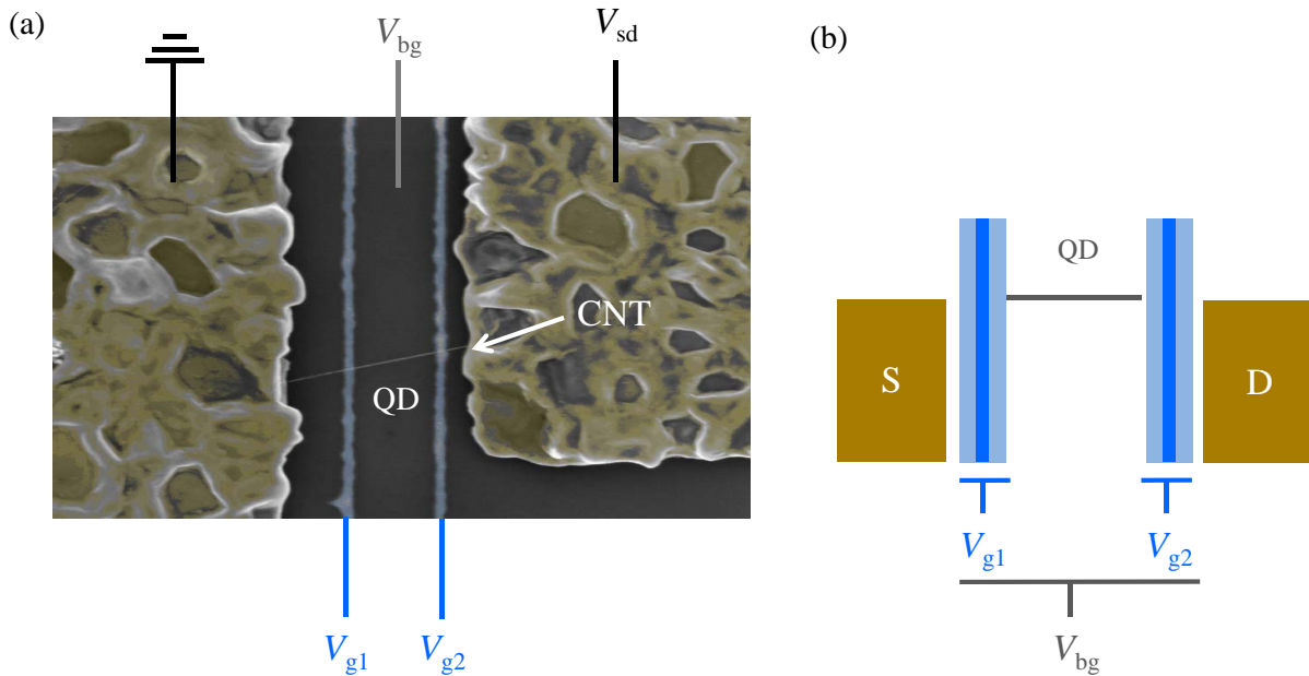
Figure 7.1: (a) False color SEM image of a carbon nanotube NEMS with two 50 nm wide metal gates, V_{\text{g1}} and V_{\text{g2}} , and Si++ backgate V_{\text{bg}} . (b) One can tune the tunnel barriers of the quantum dot independantly using the two local gate voltages. Light blue (dark blue) corresponds to an opaque (transparent) tunnel barrier.
