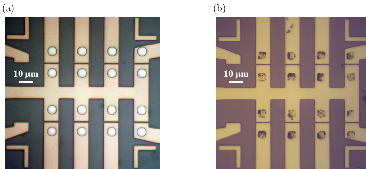
Figure 4.10: Photography of the backbone junction array for carbon nanotube NEMS (a) after lithography and (b) after catalyst deposition.
