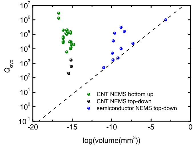
Figure 3.3: Quality factor Q_{cryo} at cryogenic temperatures ( T < 4K ) as a function of the NEMS' volume. The quality factors for conventional (blue dots) and carbon nanotube (black dots) top-down NEMS were extracted from [1]. Quality factors for bottom-up carbon nanotube NEMS (green dots) were compiled from [1, 19, 65, 66]. The dashed line represents the expected trend of the Q factors of top-down conventional NEMS upon reduction of their dimensions.
