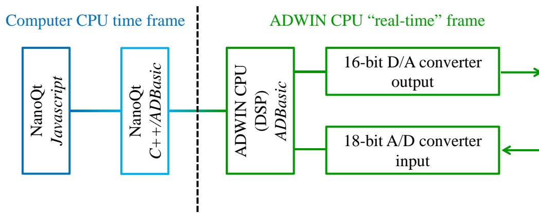
Figure 4.14: Schematic representation of the real-time data acquisition system: A measurement procedure can be impletped in Javascript in NanoQt and sent to digital signal processor (DSP) of the ADWIN in the form of a sequence of ADBasic instructions. The DSP will carry out those instructions within the reference time frame given its frequency (300 MHz).
