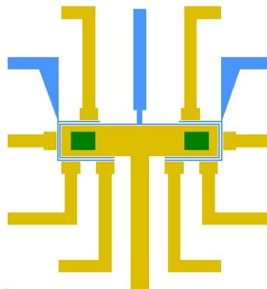
Figure A.6: Multiple gate carbon nanotube NEMS, third layer catalyst islands (green colors). 50 \mu\text{m} writefield, showing two 3 \times 4 \mu\text{m} catalyst islands on the central drain electrode.
