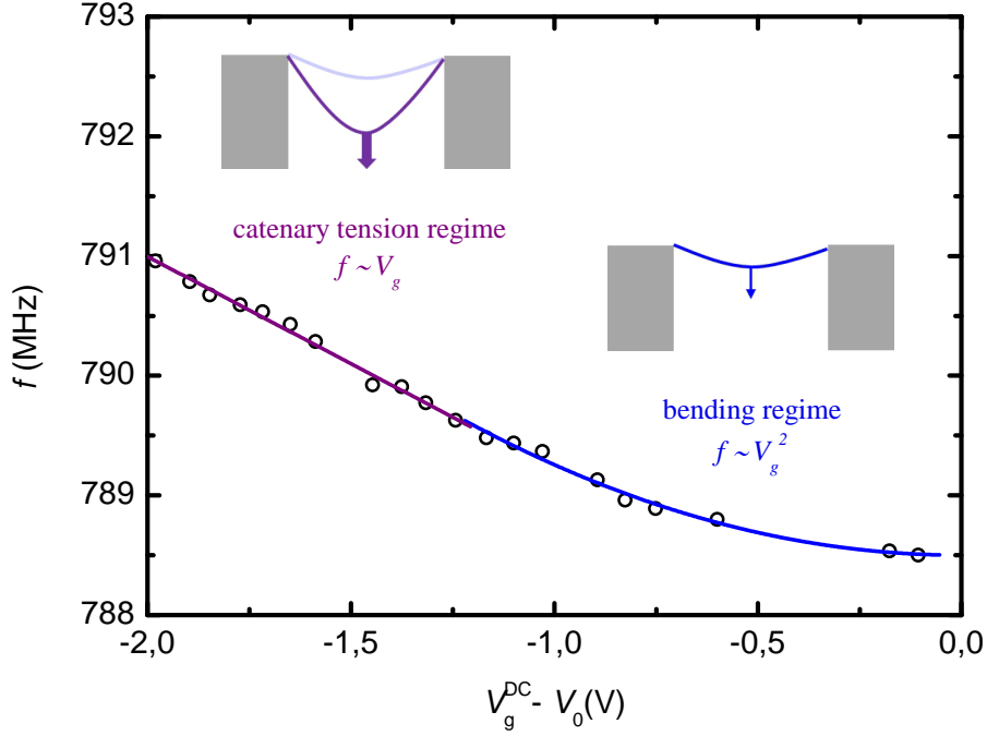
Figure 3.8: Frequency dispersion of a carbon nanotube NEMS at T = 20 mK. In the bending regime (blue segment), the applied force to the nanotube is small and the frequency follows a quadratic dependance on the gate voltage. In the catenary tension regime (purple segment), the force becomes large and the frequency depends linearly on the gate potential.
