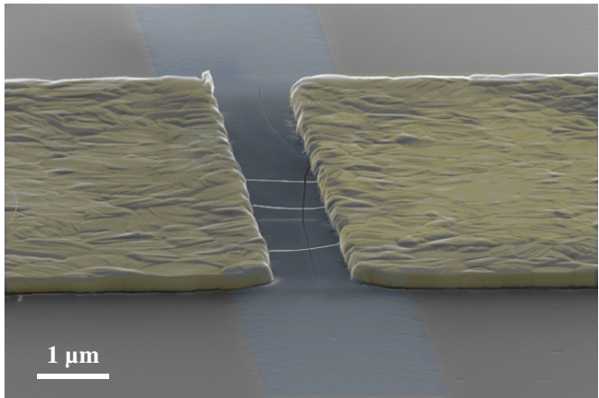
Figure 4.12: Impact of catalyst concentration: (a) Low catalyst density results almost exclusively in single tube devices, but to a very low yield of \eta_{\text{tot}} \sim \eta_1 \sim 1\% . (b) Higher catalyst density increases the yield for single tube devices \eta_1 \sim 5\% , but also results in multiple tube devices and a higher overall yield of \eta_{\text{tot}} . The images in the right column are false color SEM images with the localgate colored in blue and the source-drain junction in gold. The contrast was enhanced for better visibility of the carbon nanotubes.
