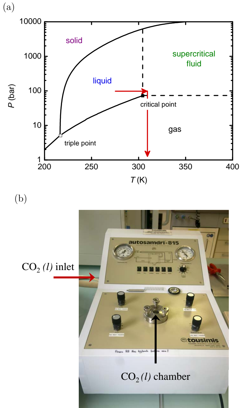
Figure 4.31: Critical point drying: (a) \text{CO}_2 phase diagram. A supercritical point drying (red path) allows to perform a liquid-gas phase transition without crossing the phase boundary. (b) Tousimis Autosamdri 815 critical point dryer.
