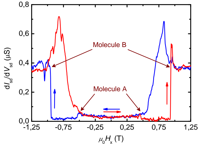
Figure 6.14: Supramolecular spin valve in the hybrid nanotube-molecule device LSM-hybrid . Hysteresis loop at T = 20\text{mK} and a magnetic field H_x applied along the carbon nanotube axis. The red (blue) curve correspond to up(down)-wards magnetic field sweeps. The device exhibits a strong change in magnetoconductance.
