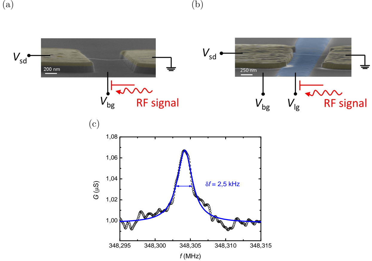
Figure 5.1: False color SEM image of (a) a low capacitance device based on a \text{SiO}_2 covered Si backgate (grey color) and (b) a high capacitance device based on an \text{Al}_2\text{O}_3 covered local metallic gate (blue). The RF actuation signal is injected into the local metallic gate and Si backgate, respectively, through a home-built bias-T. As the induced mechanical motion changes the charge flow through the CNT quantum dot and vice versa, we can detect the CNT resonance through a change in zero-bias conductance. (c) Mechanical resonance of a typical CNT NEMS at low driving power P_{\text{RF}} = -100 dBm. The resonance width \delta f = 2.5 kHz leads to a quality factor of Q \approx 140000 .
