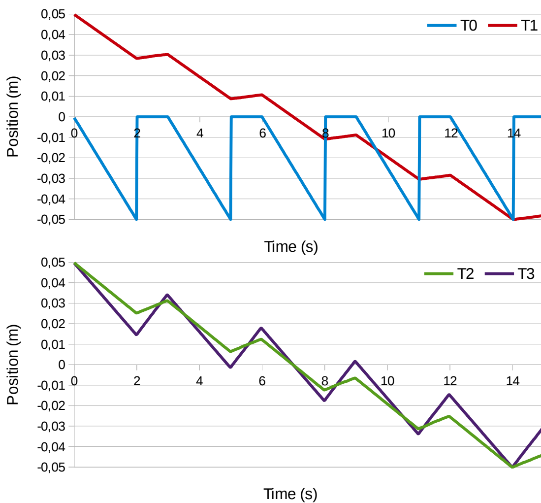
Figure A.3: Haptic effects for the sequence S3. The curves show the positions of an actuator according to the profile selected (T0, T1, T2 or T3). Five effects have been designed.
