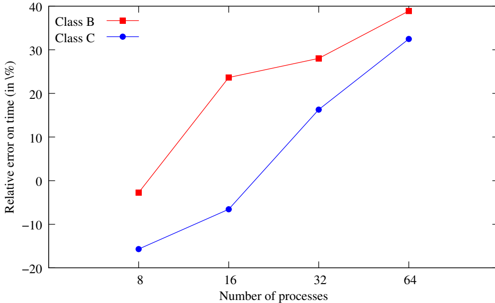
Figure 4.25: Evolution with regard to the number of processes of the relative error between execution and simulated times for the execution of the LU factorization on the borderreau cluster.
