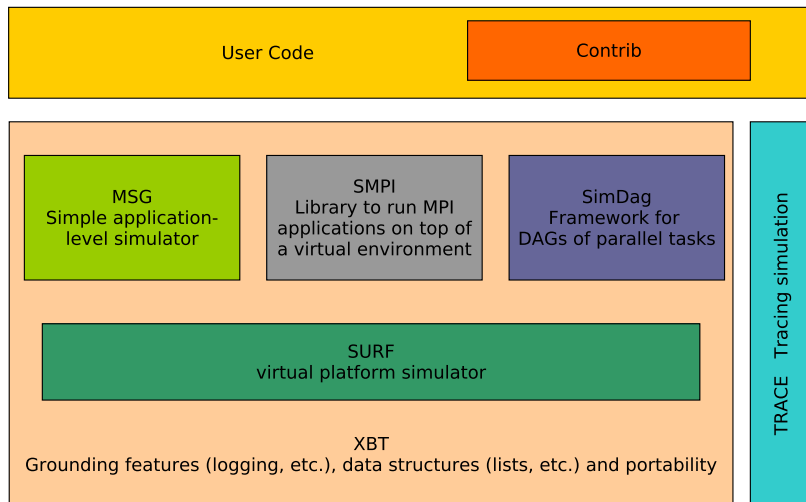
Figure 2.6: SIMGrid components.
