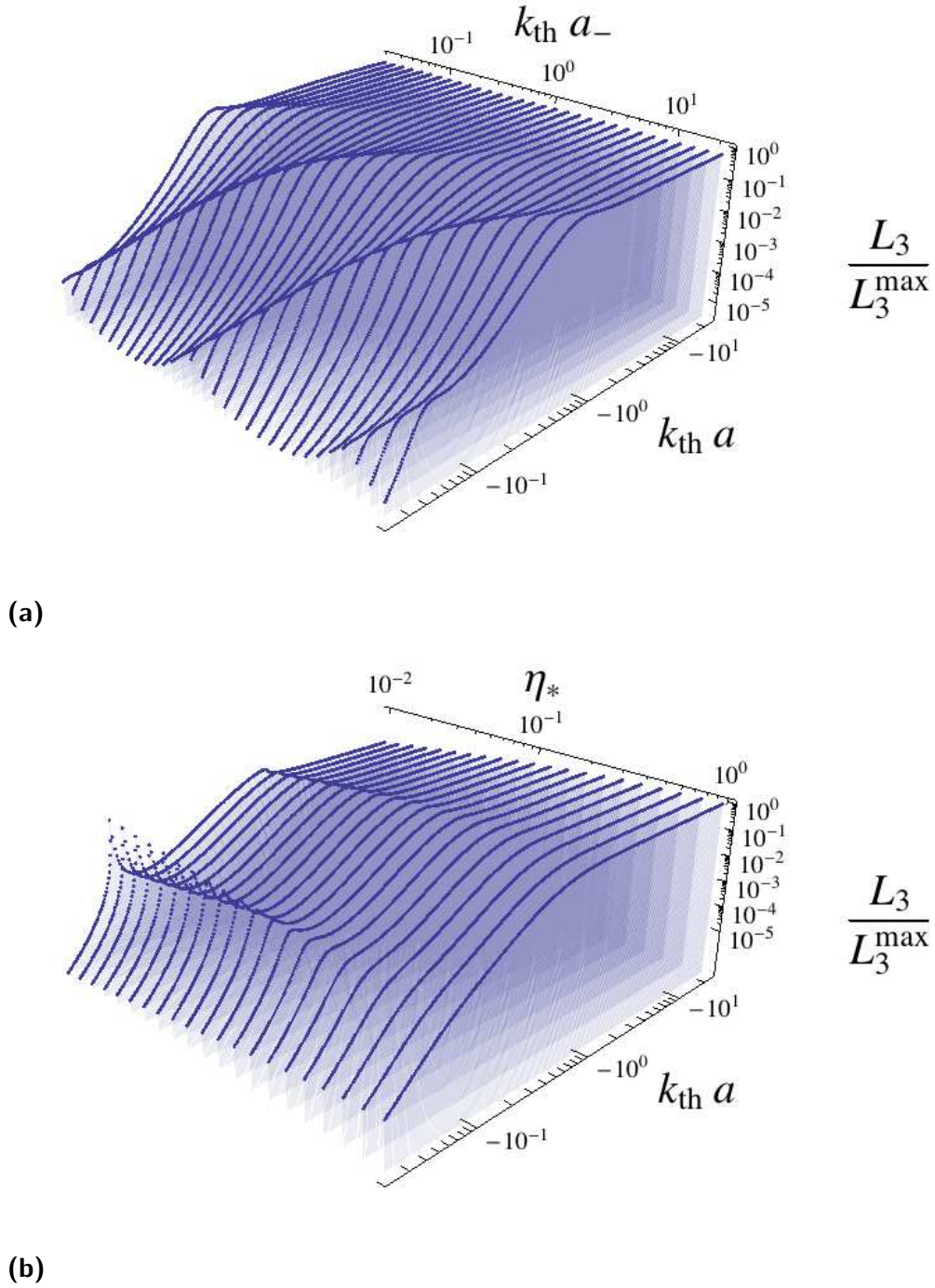
Figure 2.11.: To give an example, the numerical calculations of L_3(a, T) of ^7\text{Li} . For weak interactions, both figures show the behavior of L_3(a) \propto C(a)a^4 and for unitary interactions ( a \rightarrow \infty ) the saturation of L_3(a) to L_3(T) is shown. (a) Fixing the elasticity parameter \eta_* = 0.21 , while varying the position of the Efimov resonance through k_{\text{th}} a_- and the scattering length through k_{\text{th}} a . Four Efimov resonances are showing the log-periodicity. (b) Fixing the Efimov resonance a_- = -274a_0 , varying the width parameter \eta_* . At resonance, the three-particle loss coefficient saturates to the value L_3(T) , which varies with 1 - e^{-4\eta_*} . For smaller \eta_* , the Efimov resonance becomes more pronounced and a second resonance becomes visible. For larger \eta_* , the Efimov resonance is fully washed out ( \eta_* \simeq 1 ).
