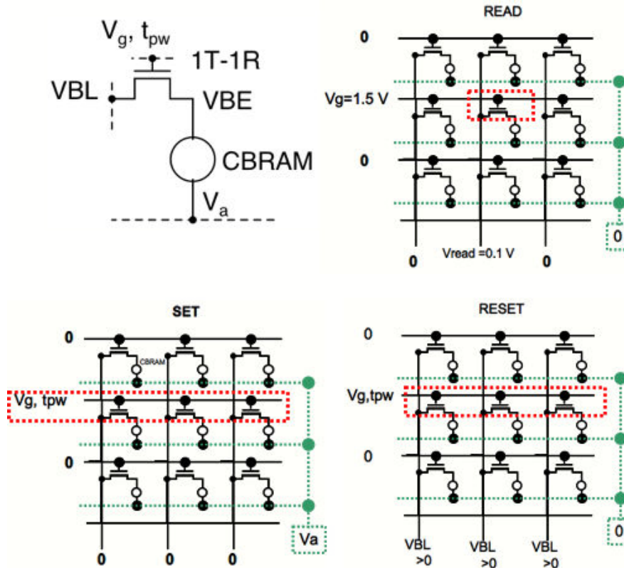
Figure 2.10: (Left up) Schematic of the 1T-1R structure. (Right up) Schematic of the 8 \times 8 NOR memory array (only three lines represented). During the read operation (right up), the anode ( V_a ) is grounded, the bitline ( VBL ) is polarized to 0.1 V and the wordline to 1.5 V. During the set operation (left down), the bitline is grounded, the gate is pulsed ( V_g, t_{pw} ) and the anode is polarized. During the reset operation (right down), the anode is grounded, the gate is pulsed and the bitline is polarized.
