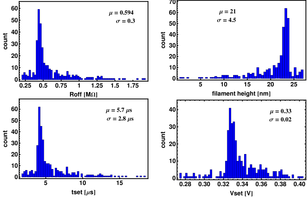
Figure 2.17: (Left up) R_{\text{off}} distributions as obtained in cycling many times GeS 2 based CBRAM devices. A log-normal distributions was used to fit the experimental values. (Right up) Calculated left over filament height as could be obtained after a reset operation. (Left down) Distribution of the time required to set the device starting from different left over filament heights the pulse amplitude used was 1 V. (Right down) Distribution of the voltage required to set the device starting from different left over filament heights, when a staircase ramp of 0.6 V s is used.
