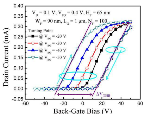
Fig. 4-29: Drain current hysteresis versus back-gate bias. The measurement started at V_{\text{BG}} = +50 V and the turning voltage was varied.
