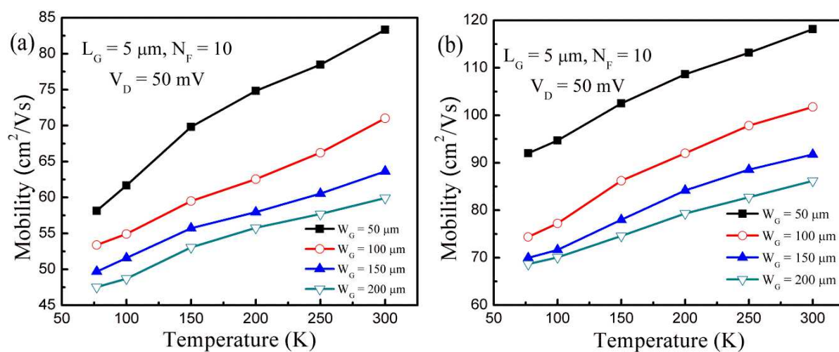
Fig. 2-41: Mobility versus temperature and gate width. (a) Modified Y-function and (b) revised Shur's model were used for mobility extraction.
