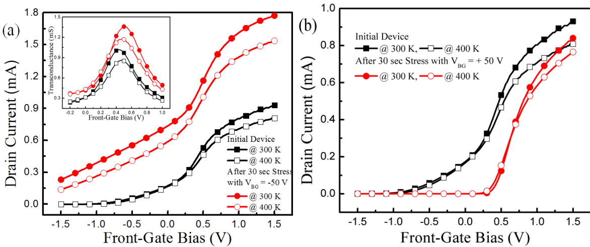
Fig. 4-18: Effect of back-gate biasing at different temperature. Drain current and transconductance (inset) versus front-gate bias measured at V_{BG} = 0 \text{ V} after 30 sec stress with (a) V_{BG} = -50 \text{ V} and (b) V_{BG} = +50 \text{ V} . L_G = 80 \text{ nm} , W_F = 90 \text{ nm} , V_D = 50 \text{ mV} , N_F = 100 .
