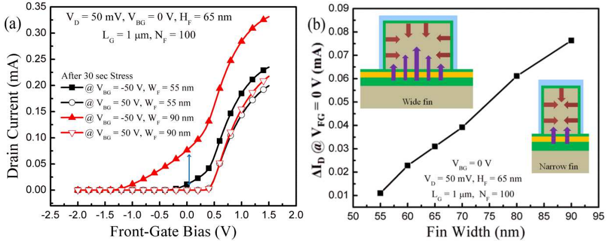
Fig. 4-17: Effect of fin width on sensing margin. (a) Drain current versus front-gate bias and fin width, measured at V_{BG} = 0 \text{ V} after charge trapping with V_{BG} = \pm 50 \text{ V} . (b) Sensing margin defined as in Fig. 4-16, versus fin width. Inset in Fig. 4-17 is cross-section of ONO FinFET showing the effect of injected charges in wide and narrow fin.
