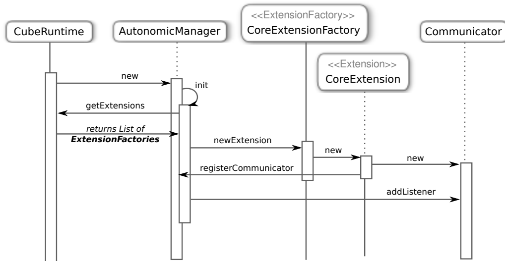
Figure 6.13: Starting Autonomic Manager Sequence Diagram
