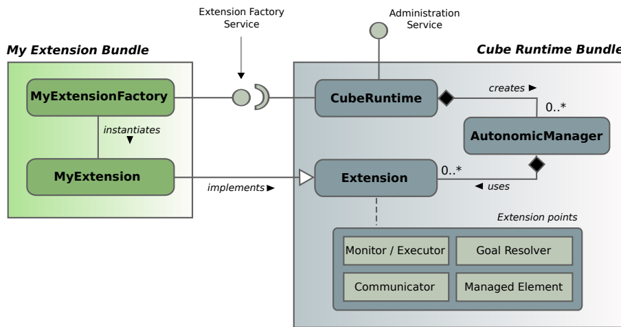
Figure 6.17: Extension mechanism
