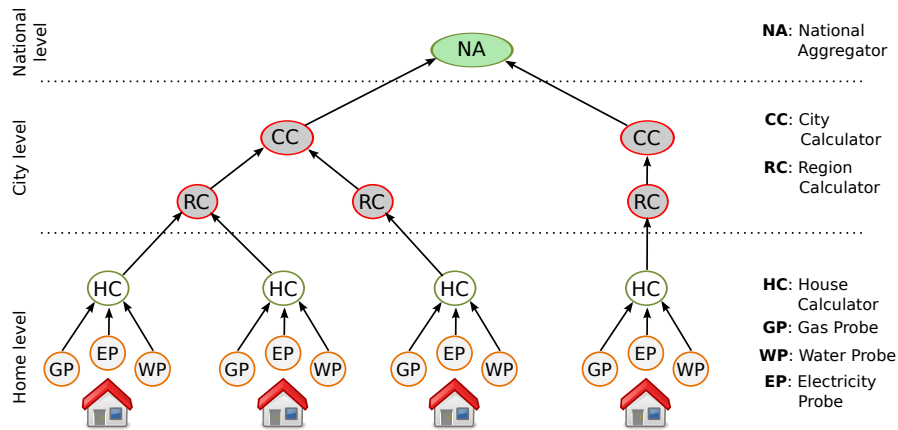
Figure 7.4: Overview of a house resource monitoring application
