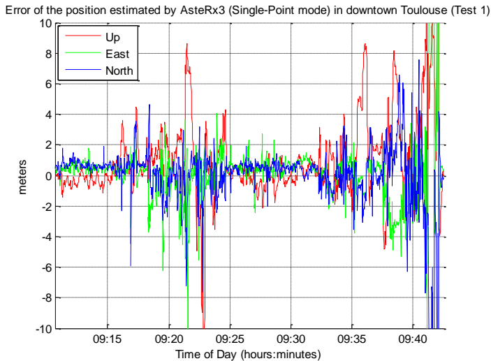
Figure 5.18 Performance of AsteRx3 single-point real-time algorithm (GPS/GLONASS L1/L2 +SBAS corrections), obtained from nmea stream collection in urban environment.
