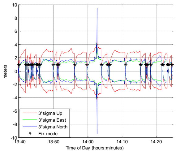
Figure 6.8 Position estimated standard deviation on Toulouse's beltway (data set 2). Black asterisk represents epochs when ambiguity vector is validated and fixed as integer
