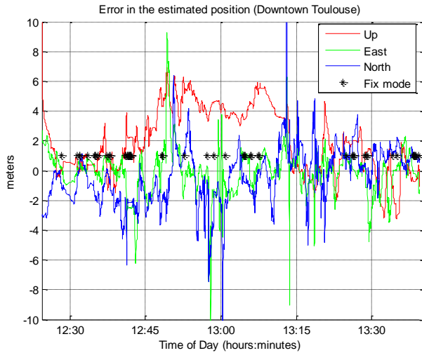
Figure 6.5 Difference between estimated trajectory and reference trajectory in downtown Toulouse (data set 2). Black asterisk represents epochs when ambiguity vector is validated and fixed as integer
