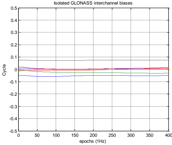
Figure 4.11 Double-differenced carrier phase residuals with the closest integer, after applying an a-priori correction of 4.41 cm for 2 adjacent frequencies, with a data set collected on June 22nd, 2012.
