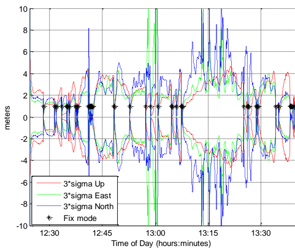
Figure 6.7 Position estimated standard deviation in downtown Toulouse (data set 2). Black asterisk represents epochs when ambiguity vector is validated and fixed as integer
