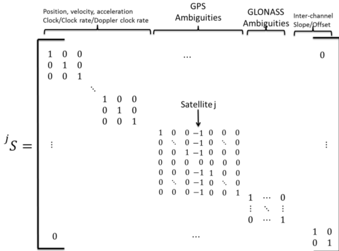
Figure 4.5 Rotation matrix related to reference satellite j
