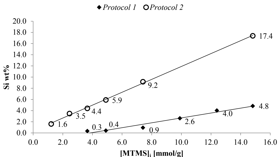
Figure 28: Evolution of Si content as a function of [MTMS]_i for NFC treated with MTMS according to Protocol 1 (pH 0.4) or Protocol 2 (pH 4).
