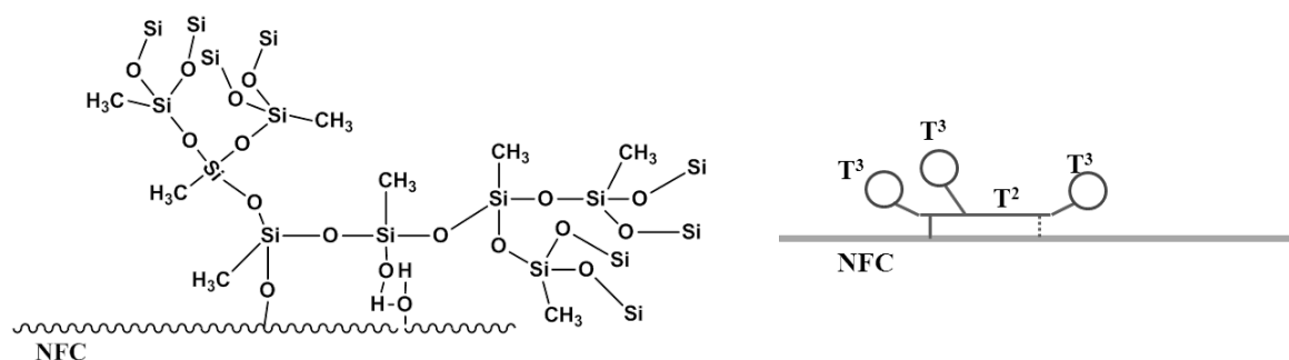
Scheme 19: Hypothesis for the bonding of polysiloxane at the NFC surface after silylation with Protocol 2
