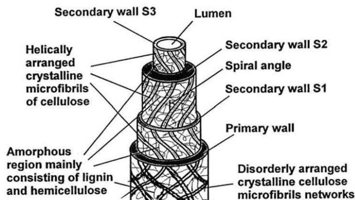
Figure 6: Structural constitution of a plant fibre cell. 18
