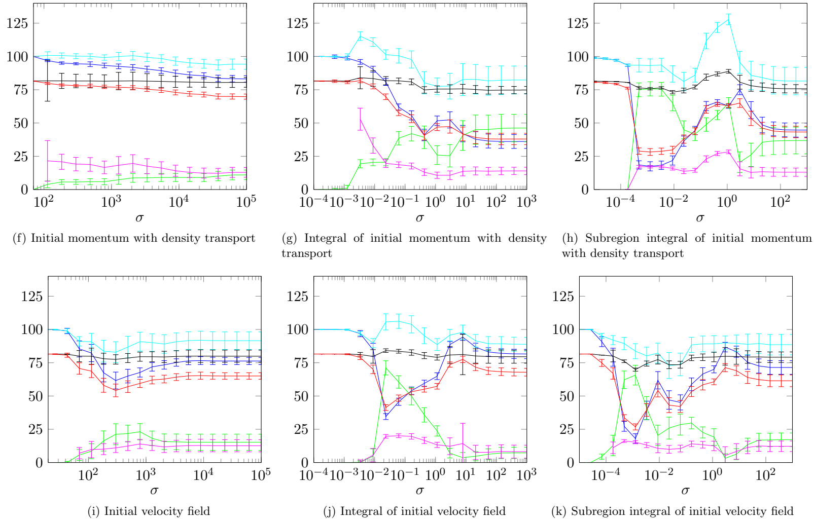
Figure 9.8: Classification performance (depending on the SVM Gaussian kernel width \sigma ) for global descriptors (9.8a, 9.8b), local (9.8c, 9.8f, 9.8i), local integrated on the whole image (9.8d, 9.8g, 9.8j) and local integrated on a subregion (9.8e, 9.8h, 9.8k). Higher for Spec + Sens (in cyan blue) is better.
