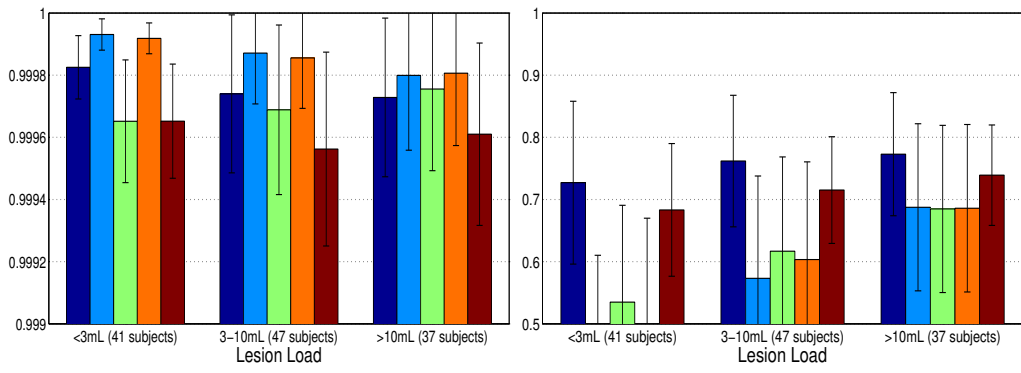
(f) Specificity
