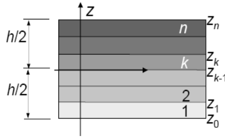
Figure 1.2: Sketch of the laminate layers and interfaces.
