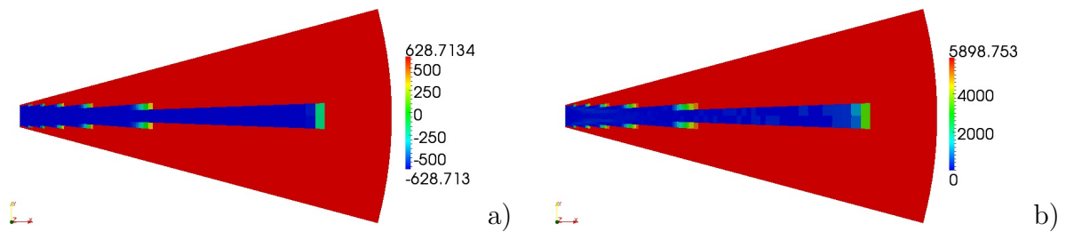
Figure 7.35: \bar{A}_{0L} (a) and \bar{A}_1 (b) for the optimal configuration, algorithm a posteriori , circular sector.
