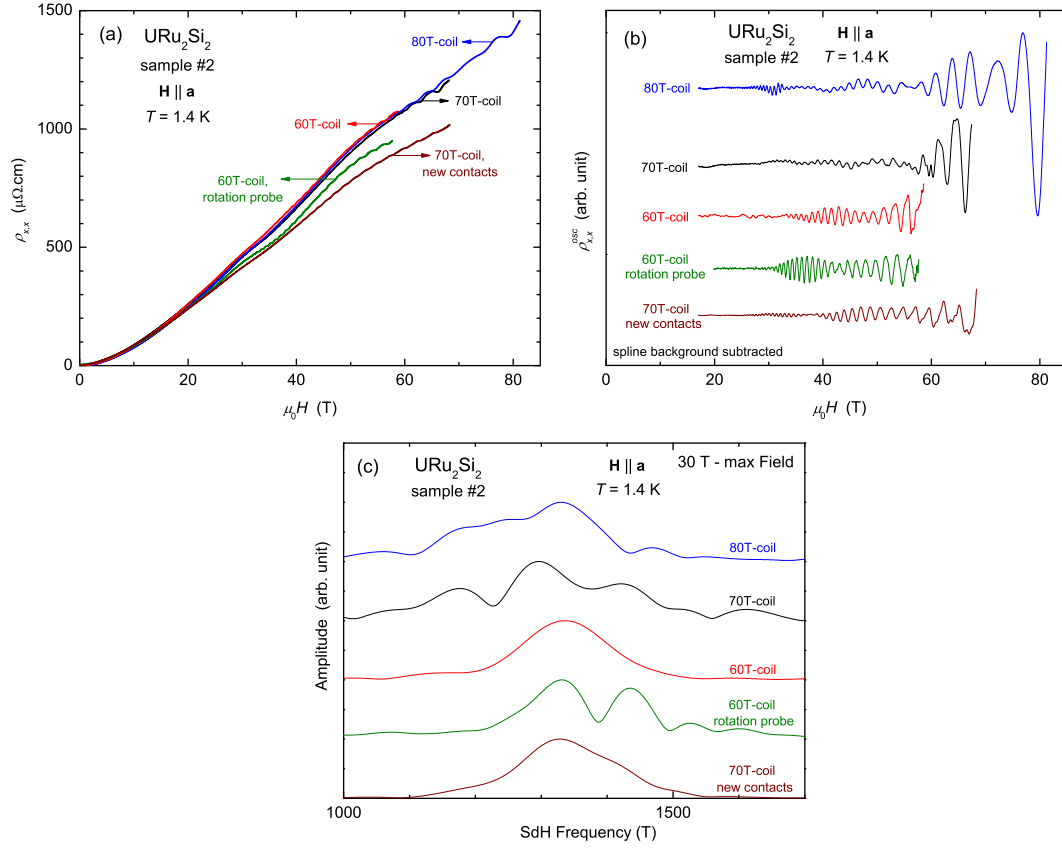
Figure 3.15: Comparison of resistivity data from measurements on URu 2 Si 2 sample #2 in different cryostat-coil setups. (a) Transverse magnetoresistivity \rho_{x,x} versus the magnetic field H applied along the a -axis at T = 1.4 K. (b) Corresponding oscillating signals \rho_{x,x}^{osc}(H) . (c) Resulting Fourier transforms.
