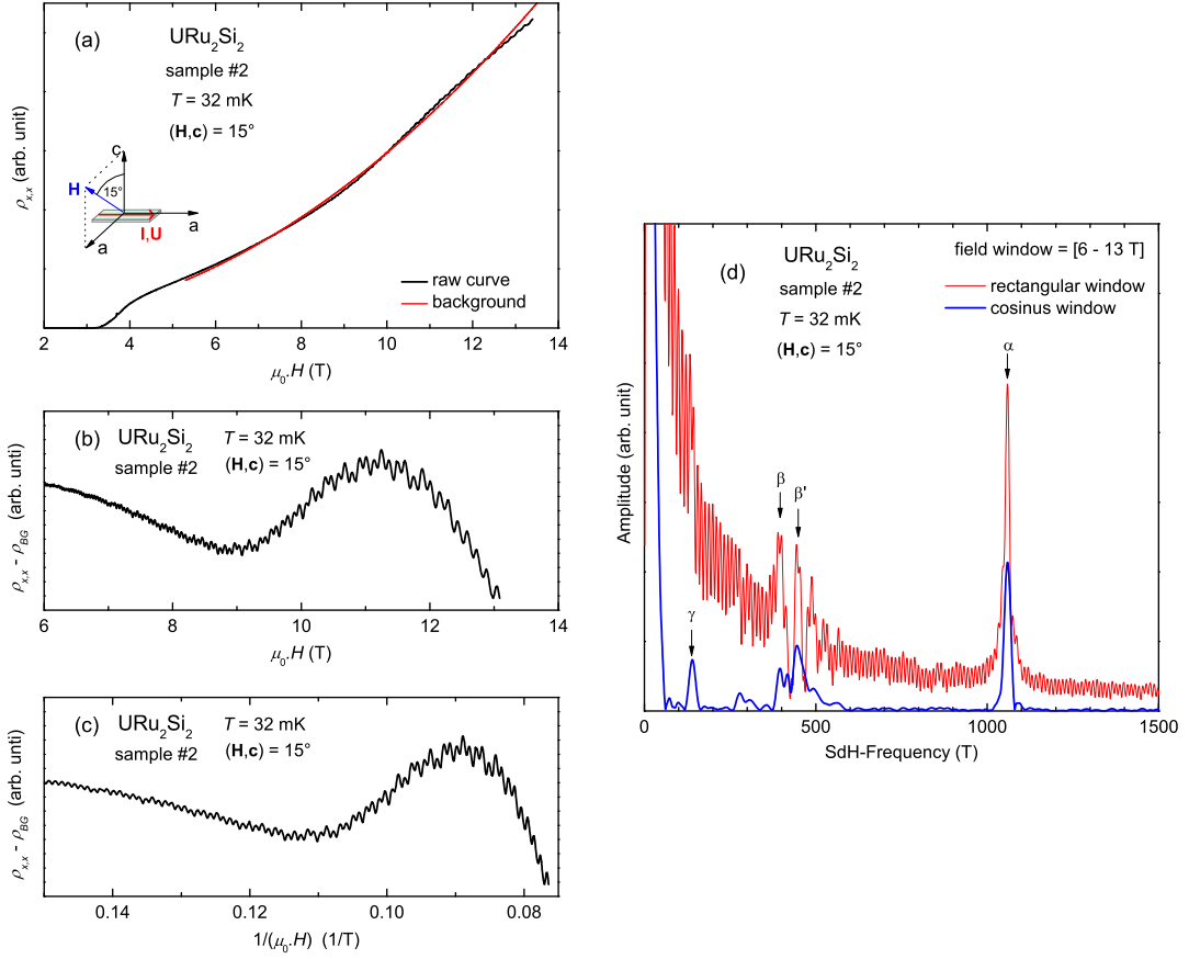
Figure 3.13: (a) Magnetoresistivity \rho_{x,x}(H) of URu 2 Si 2 sample #2 at T = 32 mK. The resistivity is modulated by Shubnikov-de Haas oscillations. The red line represents a non-oscillating polynomial background. (b) Oscillating signal \rho_{x,x}^{osc}(H) extracted from the raw resistivity by subtracting a non-oscillating polynomial background. (c) \rho_{x,x}^{osc} versus 1/(\mu_0 H) . (d) Resulting Fourier spectra using the rectangular (red) and the cosine (blue) window functions.
