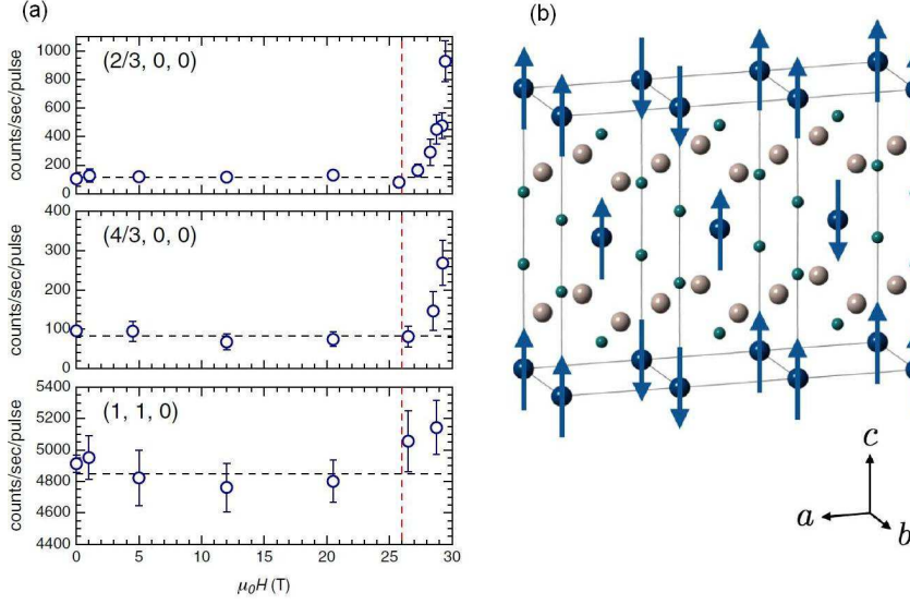
Figure 6.3: (a) Magnetic field-dependence of the intensity at the (2/3, 0, 0) , (4/3, 0, 0) , and (1, 1, 0) -Bragg peaks at T = 1.7 K. The vertical red dashed lines correspond to the critical field \mu_0 H_1 = 26 T. (b) Up-up-down magnetic structure of the field-induced phase II of U(Ru_{0.96}Rh_{0.04})_2Si_2 . Figures taken from [Kuwahara 2013].
