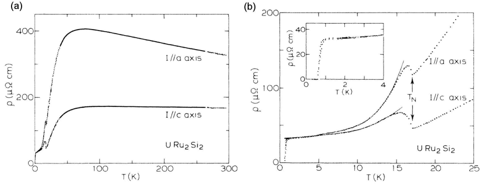
Figure 4.3: (a) Temperature dependence of the electrical resistivity of an URu 2 Si 2 single crystal with I parallel to the a and c axes. (b) Low temperature resistivity of URu 2 Si 2 showing the second-order transition at T_0 (noted here T_N ) and the superconducting transition at T_{SC} . Figures taken from [Palstra 1986].
