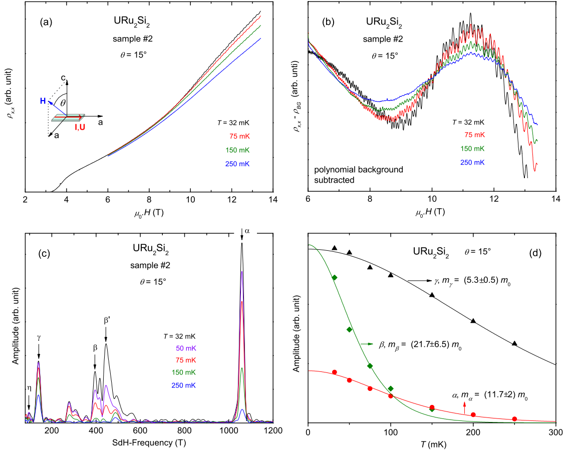
Figure 9.2: (a) \rho_{x,x}(H) of URu 2 Si 2 sample #2 for \theta = 15^\circ at temperatures from 32 to 250 mK. (b) Oscillating signal \rho_{x,x}^{\text{osc}} = \rho_{x,x} - \rho_{BG} versus H , where \rho_{BG} is a non-oscillating polynomial background. (c) Fourier spectra of the Shubnikov-de Haas oscillations observed in magnetic fields up to 13 T, for \theta = 15^\circ . (d) Mass-plots of the frequencies \gamma , \beta , and \alpha , for \theta = 15^\circ . The solid lines represent fits with the R_T -damping function.
