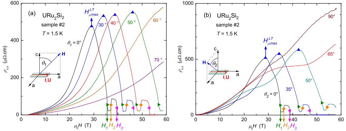
Figure 8.4: (a) Magnetoresistivity \rho_{x,x} of sample #2 versus the magnetic field H at T = 1.5 \text{ K} for different angles \theta_1 between \mathbf{H} and \mathbf{c} . The field is turning in the (\mathbf{a}, \mathbf{c}) -plane from the transverse ( \theta_1 = 0^\circ ) to the longitudinal ( \theta_1 = 90^\circ ) configurations. (b) Magnetoresistivity \rho_{x,x} of sample #2 versus H at T = 1.6 \text{ K} for different angles \theta_2 between the magnetic field and the \mathbf{c} -axis. The magnetic field is turning in the transverse (\mathbf{a}, \mathbf{c}) -plane.
