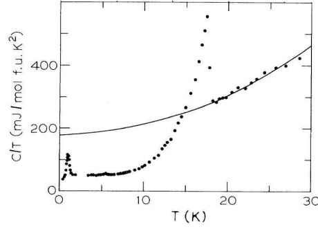
Figure 4.4: Specific heat C/T of polycrystalline URu 2 Si 2 . Figure taken from [Palstra 1985].
