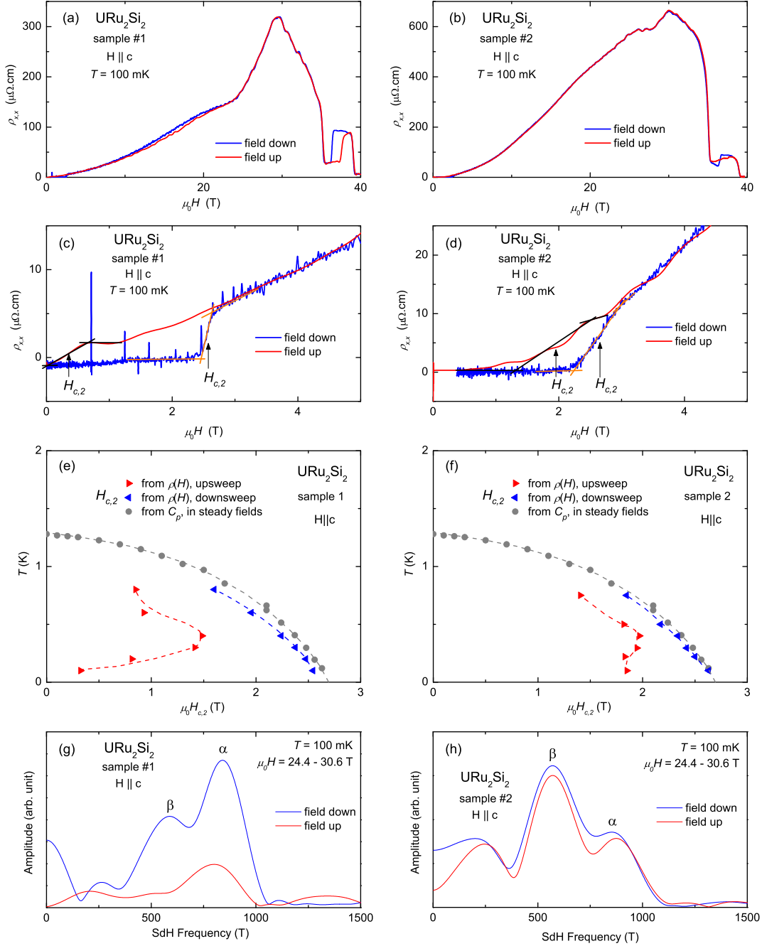
Figure 3.14: Resistivity data from URu 2 Si 2 samples #1 (left) and #2 (right) measured at T = 100 mK with \mathbf{H} \parallel \mathbf{c} in a 60 T magnet using the dilution fridge. (a,b) \rho_{xx} versus \mu_0 H . (c,d) Zoom on the superconducting critical field H_{c2} in \rho_{xx}(H) . H_{c2} is defined at the middle of the resistivity step (see black lines) for the rise (red) and fall (blue) of the pulsed field. (e,f) Phase diagram of H_{c2} from specific heat data (grey dots, [Aoki, private com. ]), rising- (red triangles), and falling-field (blue triangles) resistivity. (g,h) Shubnikov-de Haas spectra in the field window 24.4 \text{ T} < \mu_0 H < 30.6 \text{ T} from rising- (red triangles), and falling-field (blue triangles).
