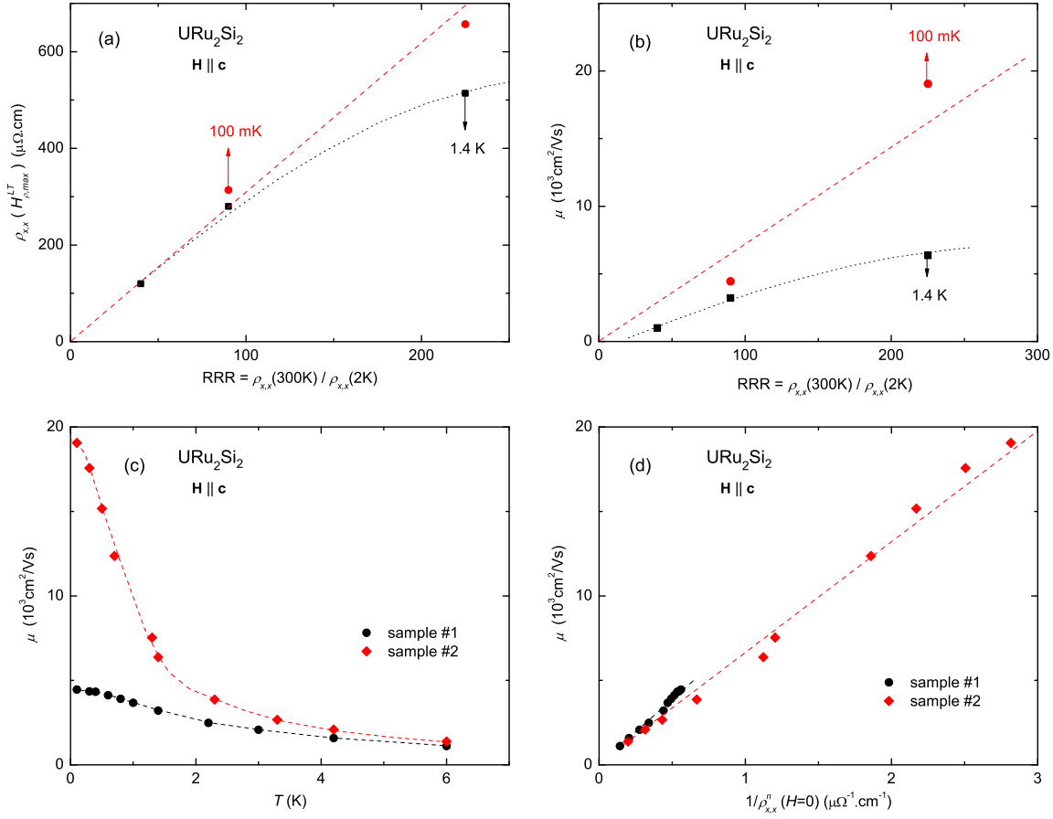
Figure 7.7: (a) Maximum of \rho_{x,x}(H) at H_{\rho,max}^{LT} in \mathbf{H} \parallel \mathbf{c} and (b) mobility \mu versus the RRR, from samples #1 (RRR = 90), #2 (RRR = 225) and that studied by Levallois et al. (RRR = 40) [Levallois 2009]. The mobilities were extracted from by the slope of \rho(H) versus (\mu_0 H)^2 in \mathbf{H} \parallel \mathbf{c} [see Fig. 7.6]. The dashed lines are guides to the eyes. Mobility \mu of samples #1 and #2 versus (c) T and (d) 1/\rho_{x,x}^n(H=0) . The dashed lines are guides to the eyes.
