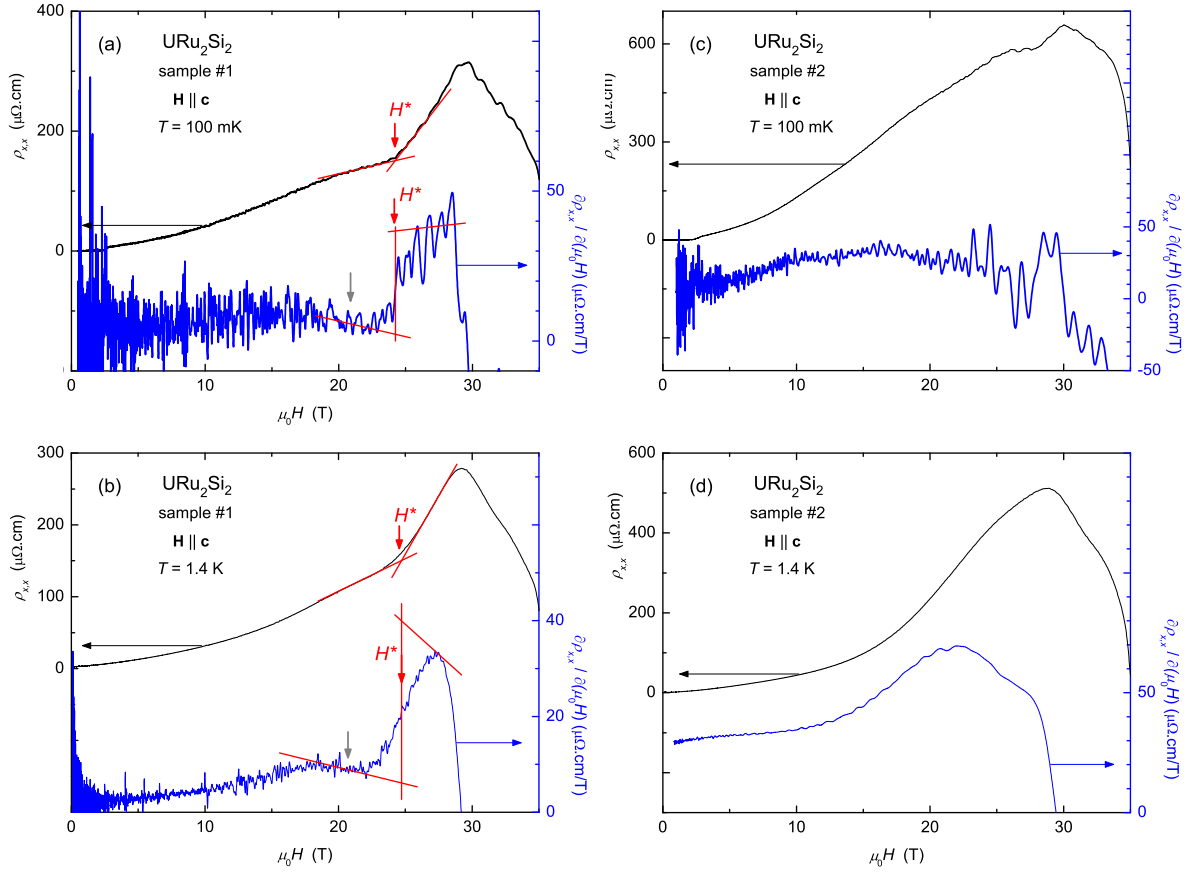
Figure 7.4: Resistivity \rho_{x,x} and field derivative of the resistivity \partial\rho_{x,x}/\partial(\mu_0 H) versus the magnetic field \mathbf{H} \parallel \mathbf{c} : (a) sample #1, T = 100 mK, (b) sample #1, T = 1.4 K, (c) sample #2, T = 100 mK, (d) sample #2, T = 1.4 K.
