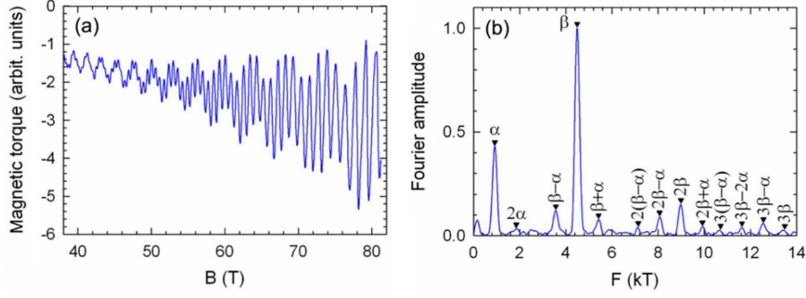
Figure 2.7: (a) De Haas-van Alphen effect in the magnetization of \theta -(ET) _4 ZnBr _4 (C _6 H _4 Cl _2 ) measured with the magnetic torque technique. (b) Resulting Fourier spectrum indicating the two fundamental frequency peaks from the Fermi surface sheets \alpha and \beta and peaks from their harmonics and linear combinations. Data published in [Béard 2012].
