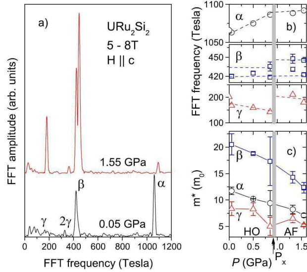
Figure 4.8: (a) Shubnikov-de Haas spectra in URu_2Si_2 for H \parallel c at T = 35 mK for p = 0.05 GPa and at T = 25 mK for p = 1.5 GPa. (b) Pressure-dependence of the Shubnikov-de Haas frequencies. (c) Pressure-dependence of the effective masses. Figures taken from [Hassinger 2010].
