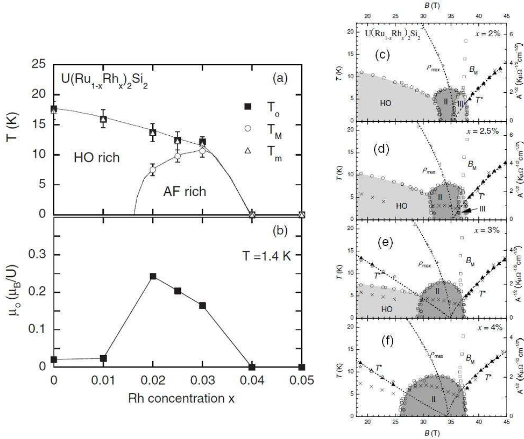
Figure 6.1: (a) Rhodium concentration-temperature phase diagram of \text{U}(\text{Ru}_{1-x}\text{Rh}_x)_2\text{Si}_2 . (b) Staggered moment m_0 (noted here \mu_0 ) of the antiferromagnetic order versus the Rh-concentration x . Figures taken from [Yokoyama 2004]. (c-d) H - T -phase diagrams of \text{U}(\text{Ru}_{1-x}\text{Rh}_x)_2\text{Si}_2 compounds for x = 0.02, 0.025, 0.03 , and 0.04 . Figures taken from [Kim 2004].
