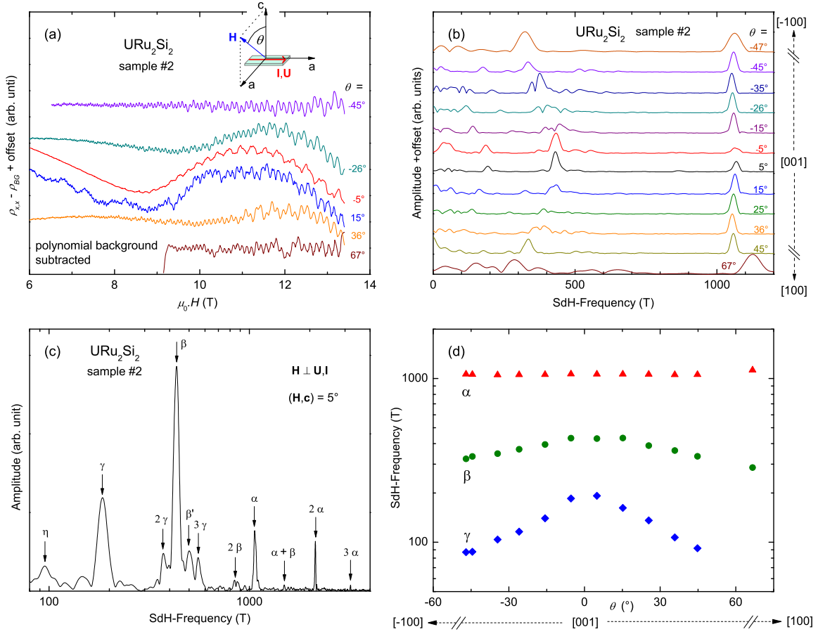
Figure 9.1: Shubnikov-de Haas data of \text{URu}_2\text{Si}_2 sample #2 at T = 32 mK and in a magnetic field up to 13 T, applied along different directions in the (a,c)-plane with an angle \theta between \mathbf{H} and \mathbf{c} . Data extracted from that shown in Sect. 8.1, Fig. 8.1. (a) Oscillating signals \rho_{xx}^{\text{osc}} = \rho_{xx} - \rho_{BG} versus H , where \rho_{BG} is a non-oscillating polynomial background. (b) Resulting Fourier spectra. (c) Example of the Fourier spectrum for \theta = 5^\circ . (d) Angle-dependence of the low-field Shubnikov-de Haas frequencies \gamma , \beta , and \alpha .
