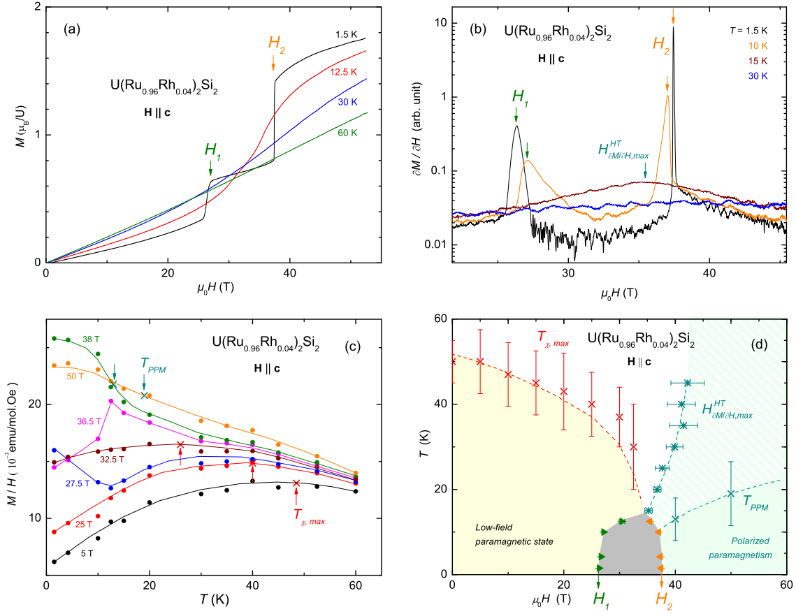
Figure 6.2: (a) Magnetization M of \text{U(Ru}_{0.96}\text{Rh}_{0.04})_2\text{Si}_2 versus the magnetic field H applied along \mathbf{c} , at temperatures between 1.5 and 60 K. (b) \partial M / \partial H versus \mathbf{H} \parallel \mathbf{c} at temperatures between 1.5 and 30 K. (c) M/H versus T at different magnetic fields \mathbf{H} \parallel \mathbf{c} . (d) Resulting H - T phase diagram of \text{U(Ru}_{0.96}\text{Rh}_{0.04})_2\text{Si}_2 .
