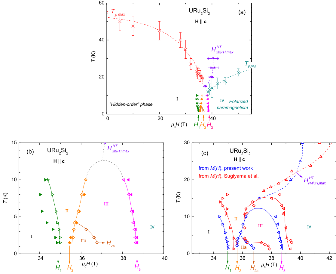
Figure 5.3: (a) H - T phase diagram constructed from our magnetization experiments for H \parallel c . Open symbols stand for the rise and full symbols for the fall of the pulsed magnetic field. (b) Zoom in the critical region of the transitions H_1 , H_2 , and H_3 . (c) Comparison of the H - T phase diagram from the magnetization experiments (from the rise of the field only) of this work and from [Sugiyama 1999].
