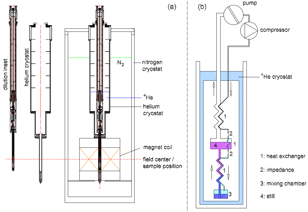
Figure 3.6: (a) Technical drawing of the LNCMI-T dilution cryostat and (b) scheme of the 3 He-cycle [Nardone private com.].
