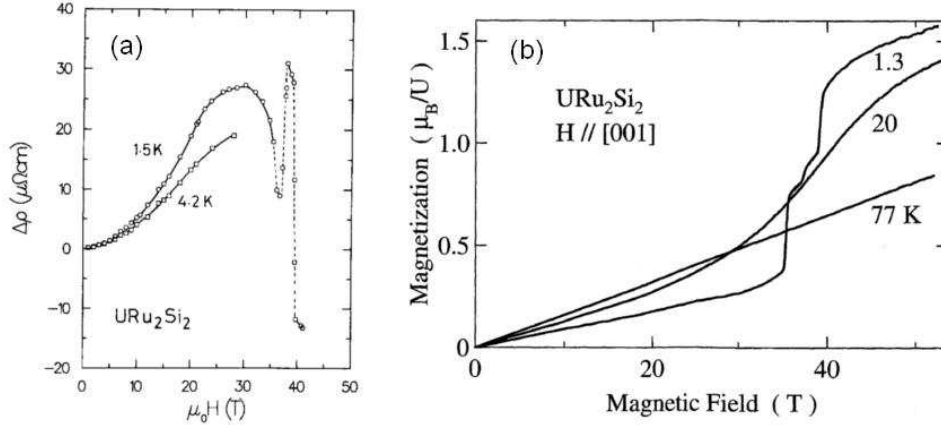
Figure 4.11: (a) Longitudinal magnetoresistivity of URu 2 Si 2 measured in a magnetic field \mathbf{H} \parallel \mathbf{I} \parallel \mathbf{c} at T = 1.5 and 4.2\text{ K} . Figure taken from [de Visser 1987]. (b) Magnetization of URu 2 Si 2 measured in a magnetic field \mathbf{H} \parallel \mathbf{c} at T = 1.3\text{ K} , 20\text{ K} , and 77\text{ K} . Figure taken from [Sugiyama 1999].
