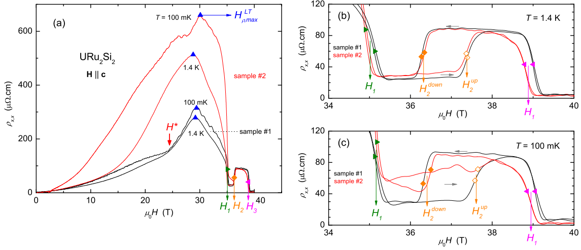
Figure 7.3: (a) Transverse magnetoresistivity \rho_{x,x} of URu 2 Si 2 samples #1 and #2 versus the magnetic field H applied along \mathbf{c} at T = 100 mK and 1.4 K. Zoom on \rho_{x,x}(H) of samples #1 and #2 for \mu_0 \mathbf{H} \parallel \mathbf{c} between 34 T and 40 T at (b) T = 1.4 K and (c) T = 100 mK. The grey arrows indicate the directions of the rise and fall of the pulsed field.
