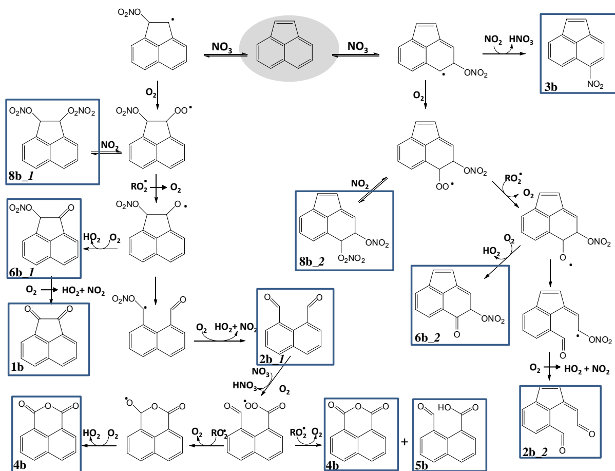
Figure 4: Proposed mechanism for the reaction of acenaphthylene with \text{NO}_3 radicals. Blue boxes correspond to compounds identified using both analytical techniques.
