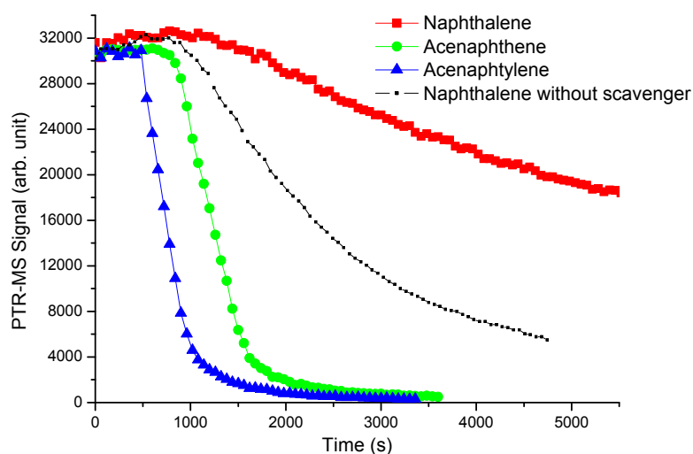
Figure 1: Concentration time profiles of naphthalene (with and without scavenger), acenaphthene and acenaphthylene when adding chlorine atoms in the presence of oxygen.
