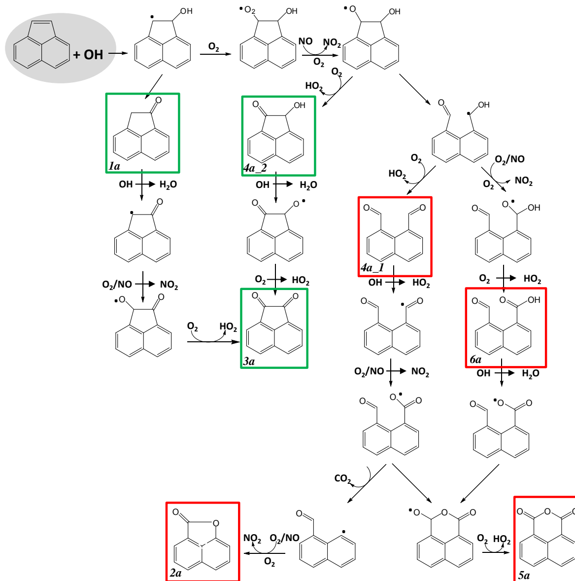
Figure 2: Proposed mechanism for the acenaphthylene photooxidation under high-NO x conditions.
