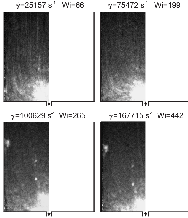
Figure 5.7.: Picture series of PEO50 55/45 immediately upstream of the contraction for different flow rates. The corresponding shear rates and Weissenberg numbers are given above each picture. As described in the text, the other half of the channel could not be recorded, due to experimental problems. In the lower pictures, it is again possible to observe vortices upstream of the constriction.
