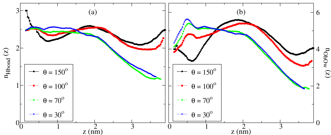
Figure 6.13: Number of hydrogen-bonds per \text{H}_3\text{O}^+ n_{\text{Hbond}}(z) and number of first neighbours n_{\text{OhOw}}(z) as a function of the distance z from the wall.
