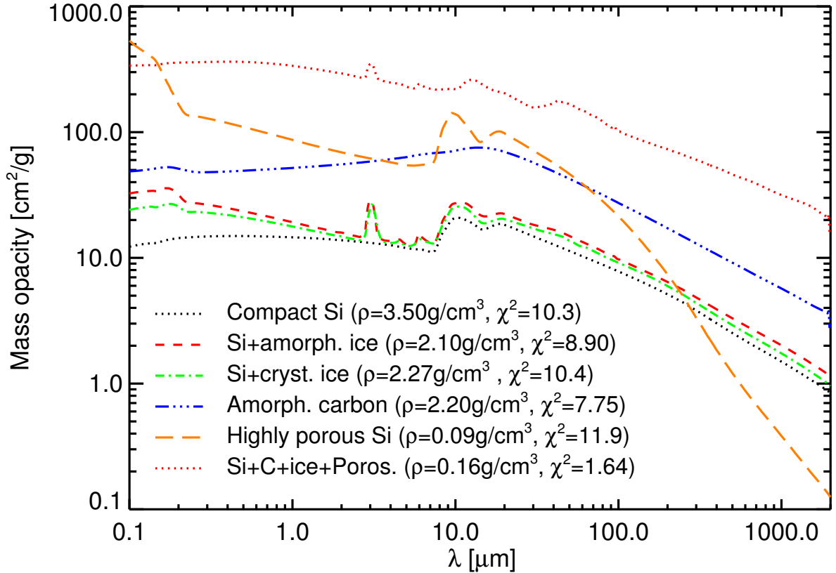
Figure 3.8: Mass opacity of spherical grains computed with the Mie theory and Bruggeman mixing rule for several prototypical compositions detailed in Tab. 3.6 and their associated best-fit size distributions.
